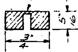
CROSS SECTION FULL SIZE
