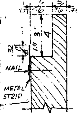
FULL SIZE CROSS-SECTION OF ENDS
