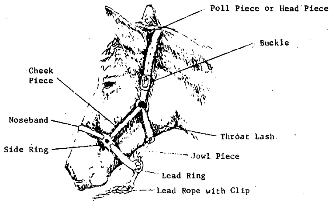
Leather Halter for Horses, Donkeys, Mules, or Cattle
