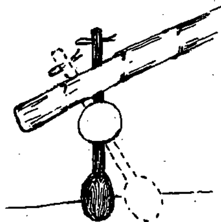
Side view of handle crossbar joint showing how joint affects tooth penetration angle.
