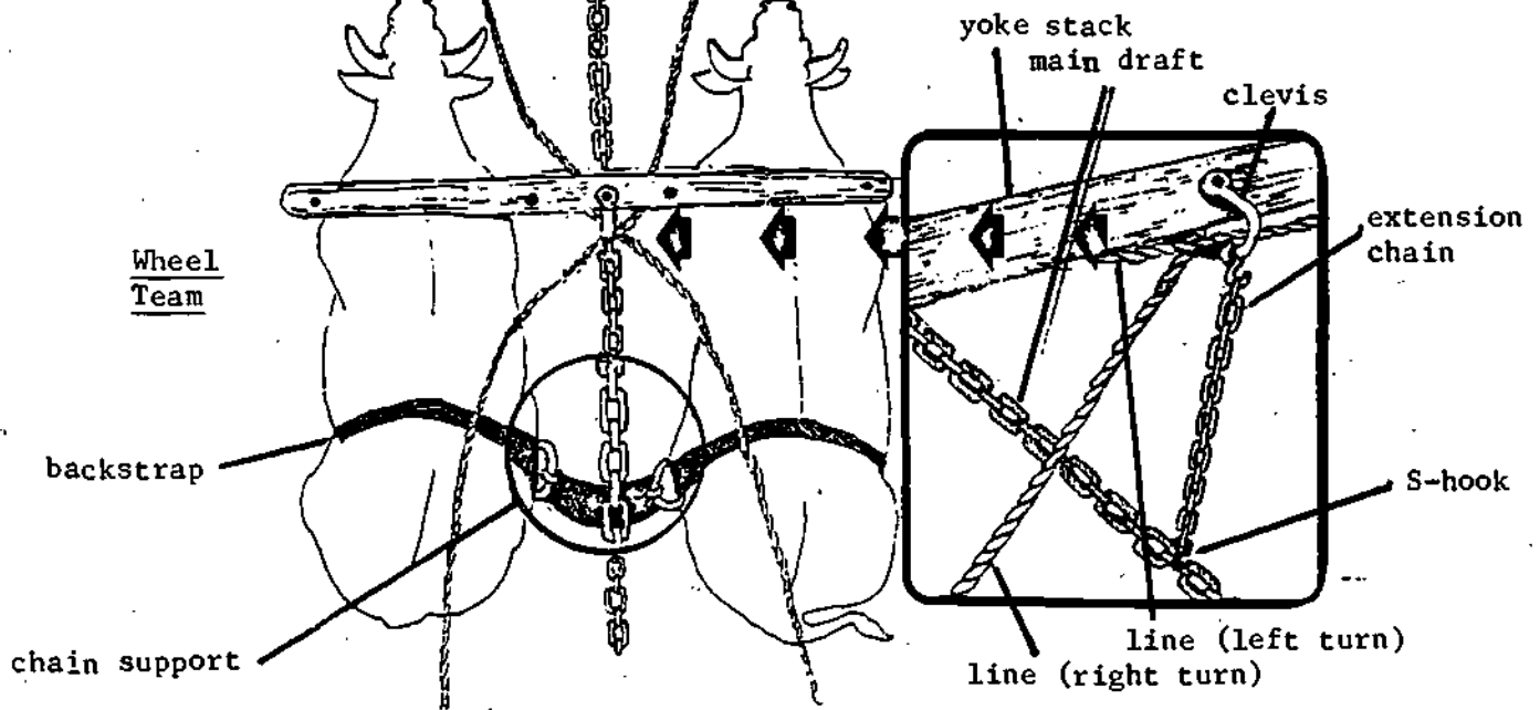
Tandem Yokes to Implement (with magnifications of hitchpoints)
