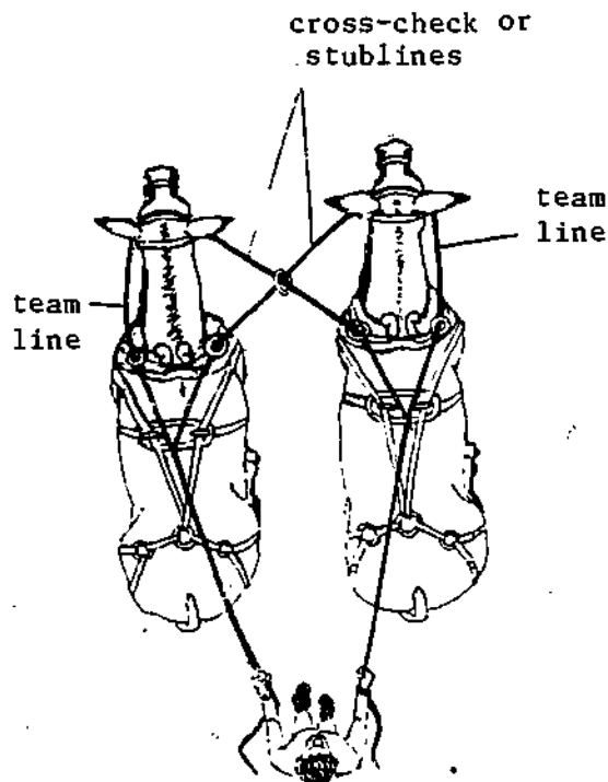
Team Lines with Cross-Check
