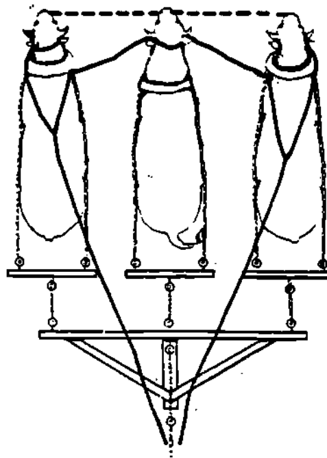
Three-Abreast Hitch
