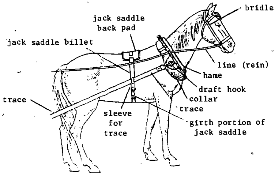
Collar Harness Consisting of Collar and Hames, Jack Saddle, Traces, and Bridle with Lines
