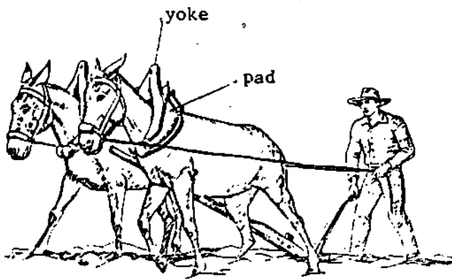
Wooden-Sling Type Yoke Used with Collar. The sling is similar to a set of hames.
