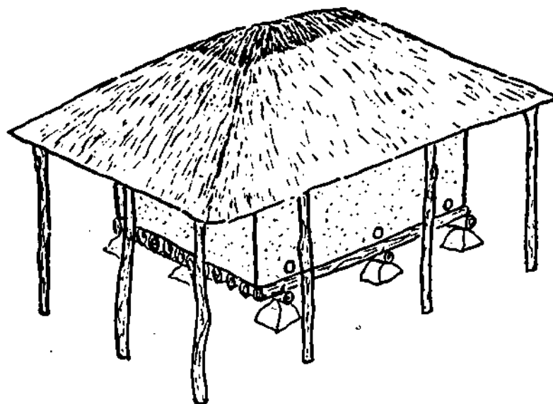
Wide thatch to keep rain and sun off the mud crib.
