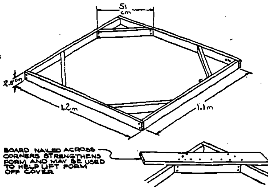
FRAME A
