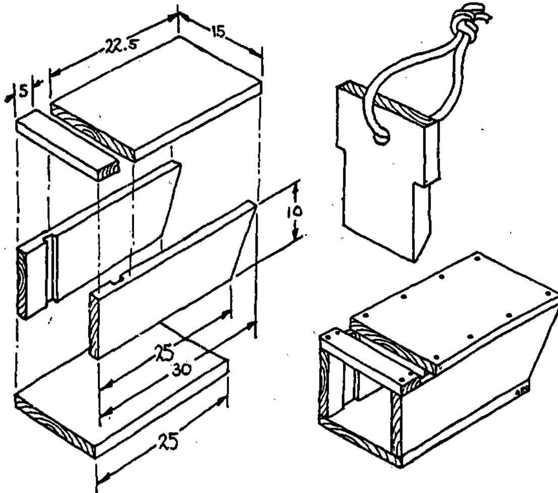
GRAIN CHUTE
