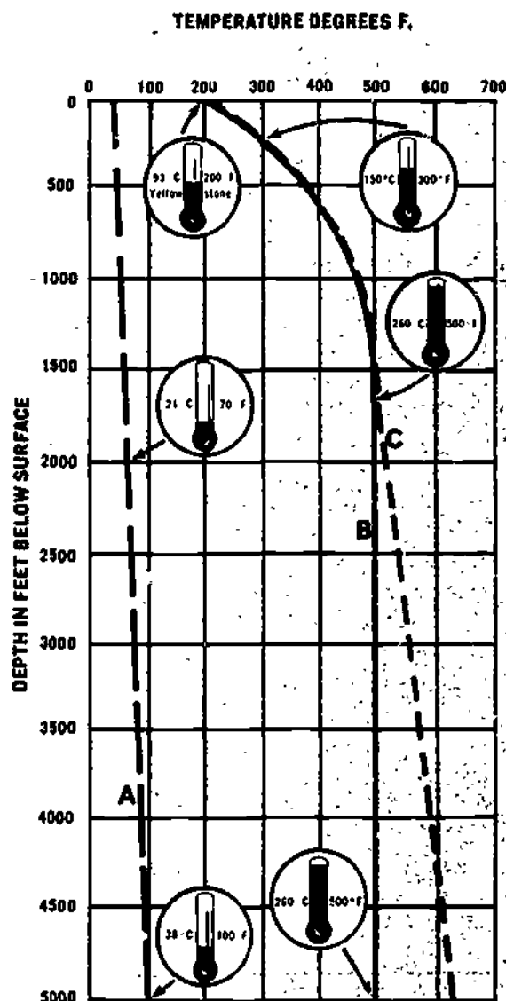
Figure 2.—Temperature variations in the Earth
