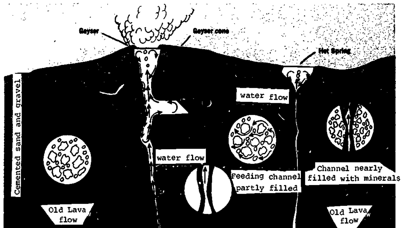
Figure 4.—Model of geyser tube showing reservoir of pore spaces and narrow feeding channels
