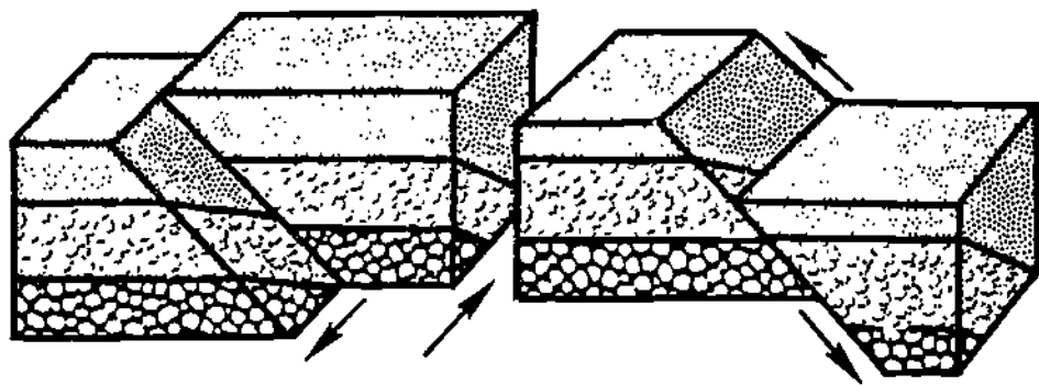
Movement along strike-slip fault (left). Movement along dip-slip fault (right).
