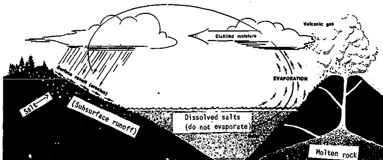
Sources of salts in the ocean.
