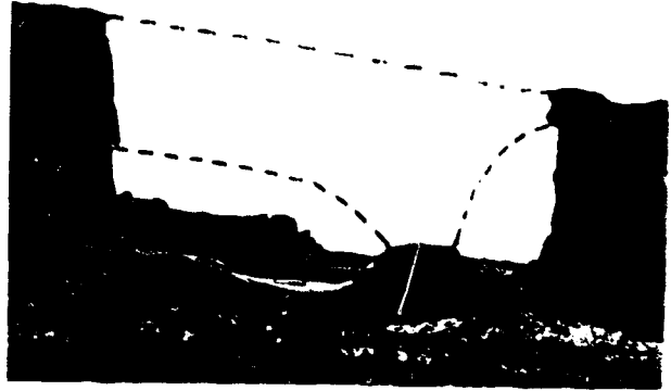
Sheep Rock is a prime example of what will eventually happen to a fin. The dotted lines represent where an arch might have existed years ago, but through erosion and weathering the fin has worn down to what we see today.
