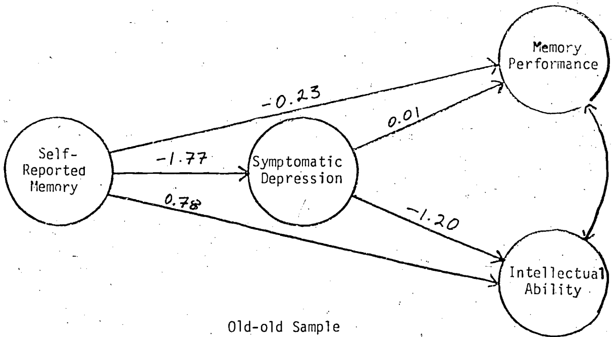
Figure 3. T-values of LISREL parameter estimates (path coefficients) for the alternative model, for young-old (top panel) and old-old (bottom panel) samples. Negative signs indicate inverse relationships between latent variables. Standard values for significant parameter estimates are given in parentheses for purpose of comparison across age and models.
