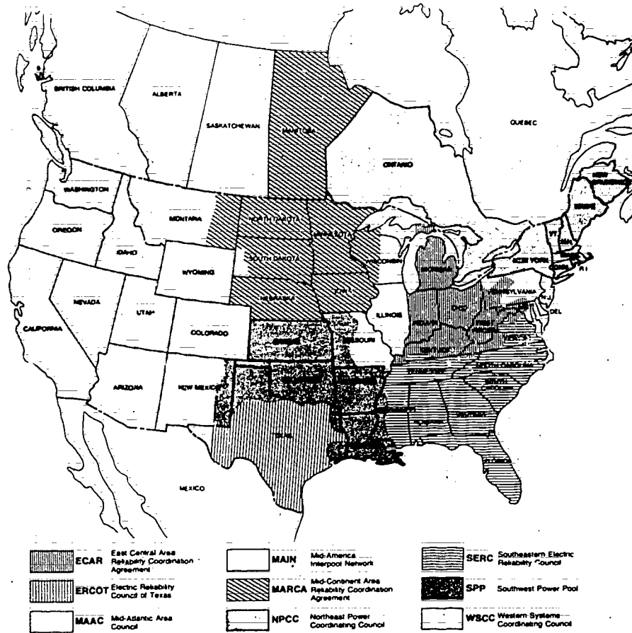
FIGURE 7 NATIONAL ELECTRIC RELIABILITY COUNCIL REGIONS (Source: NERC, 10th Annual Review, August 1980. Reproduced by permission).
