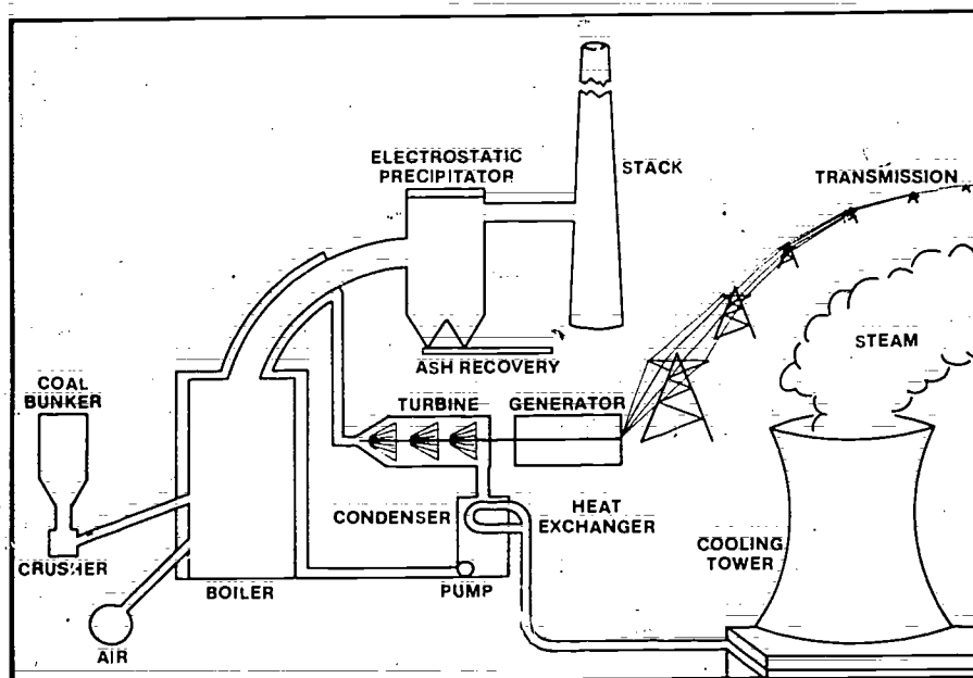
FIGURE 3 MAJOR COMPONENTS OF A COAL-FIRED POWER PLANT
