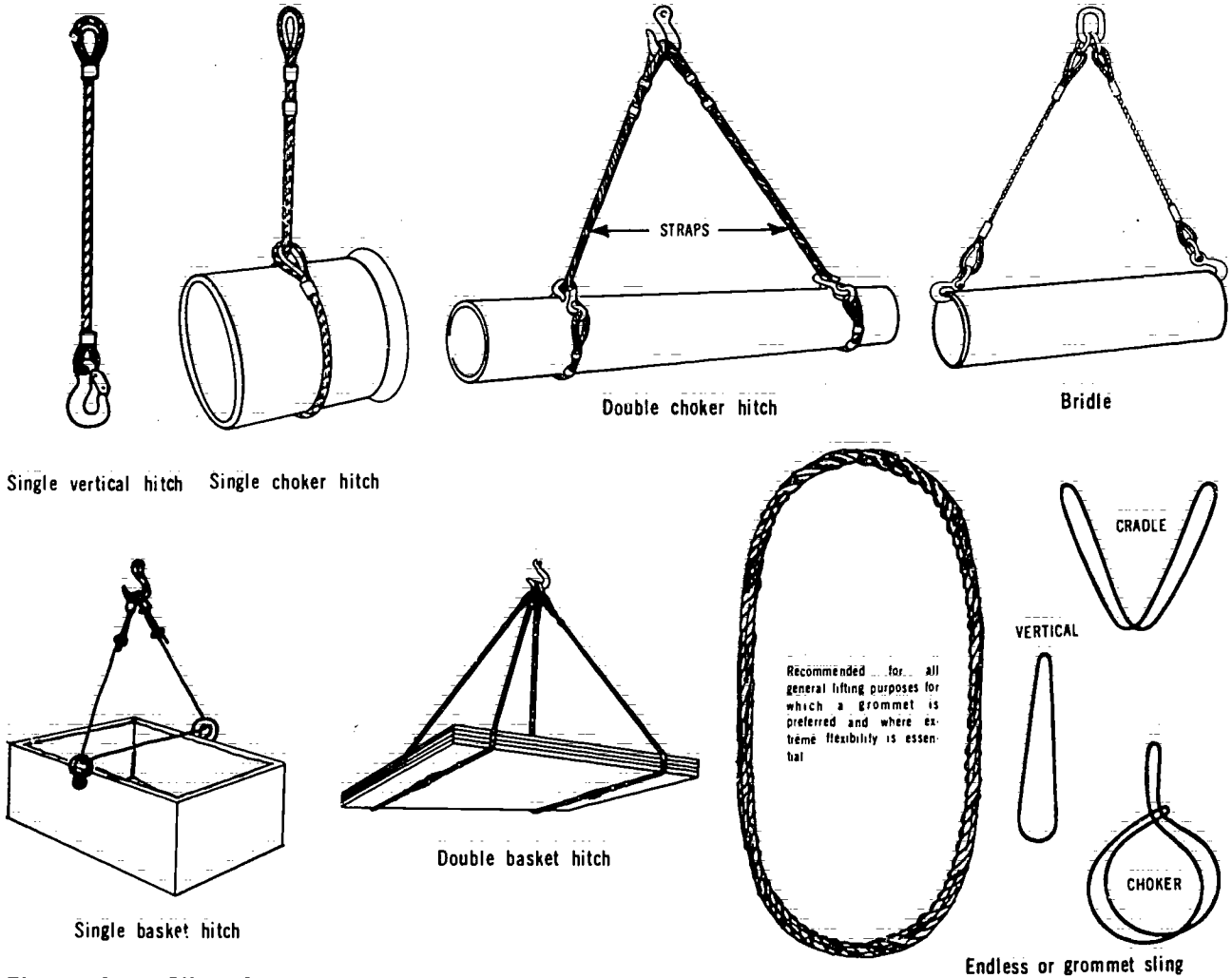
Figure 7-72. Sling Arrangements
