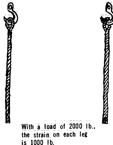
Figure 7-77. Sling Angle Principles
