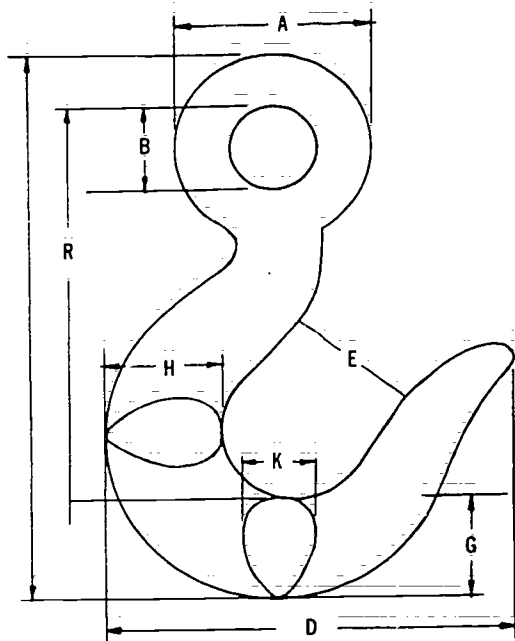
Figure 7-79. Standard Eye Hook
