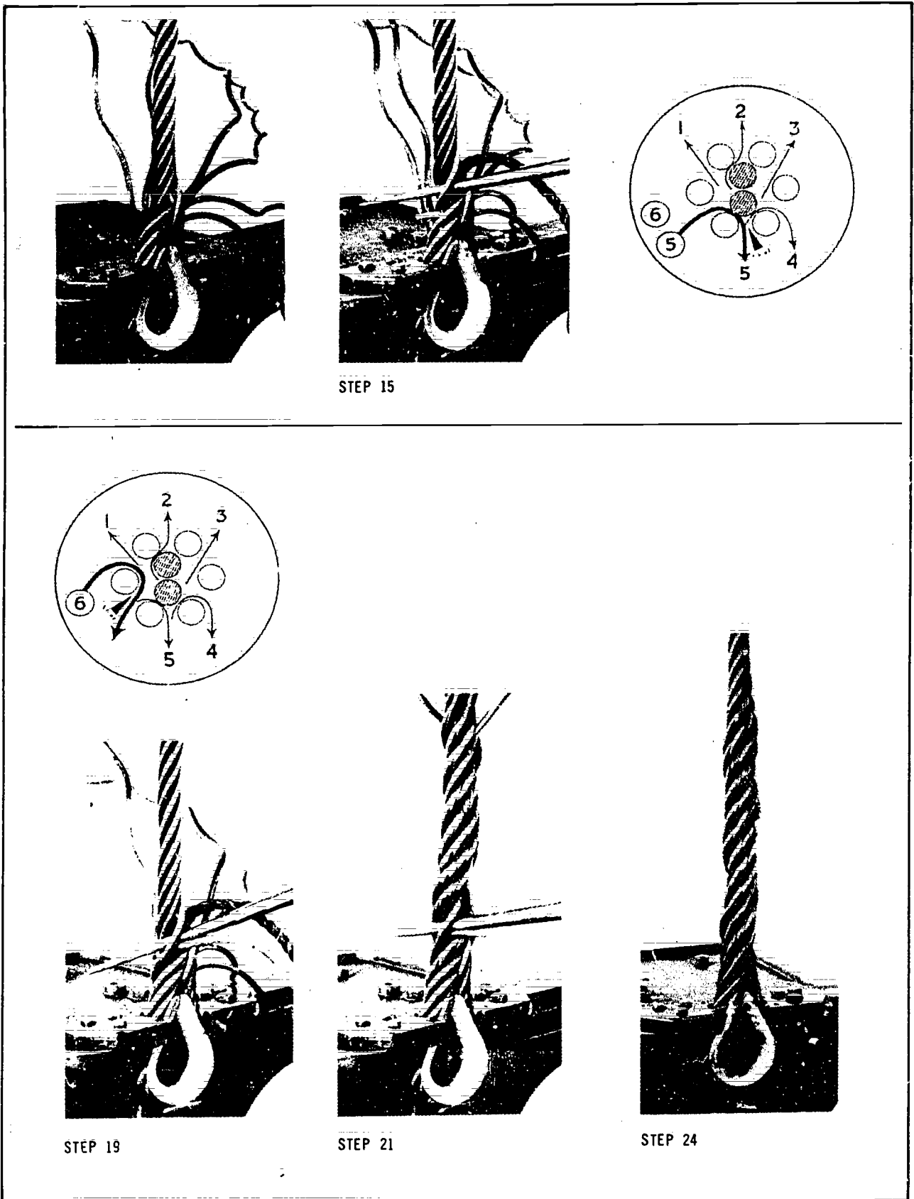
Figure 7-53. Making an Eye Splice (continued)
