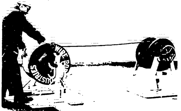
Figure 7-52. Re-Reeling Wire Rope
