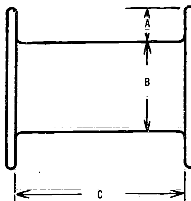
395 Figure 7-70. Determining Winch Drum Capacity
