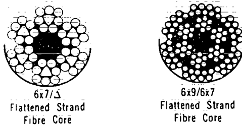
Figure 7-40. Flattened Strand Rope
