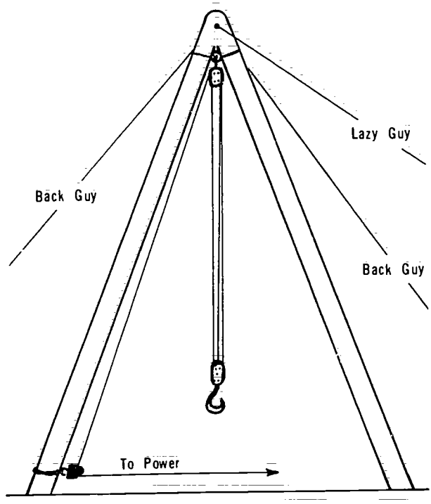
Figure 7-109. A-Frame Derrick
