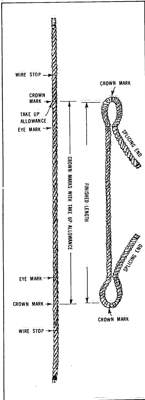
Figure 7-78. Making a Choker
