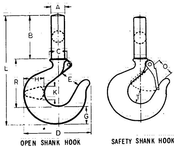
Figure 7-82. Shank Hooks
