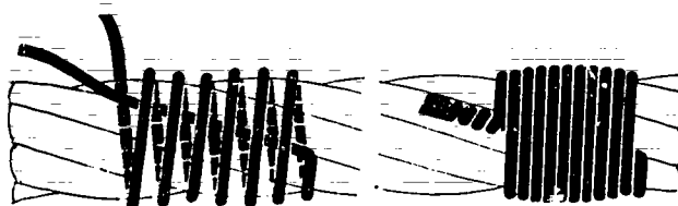
Figure 7-66. Stranding Rope-Method 1
