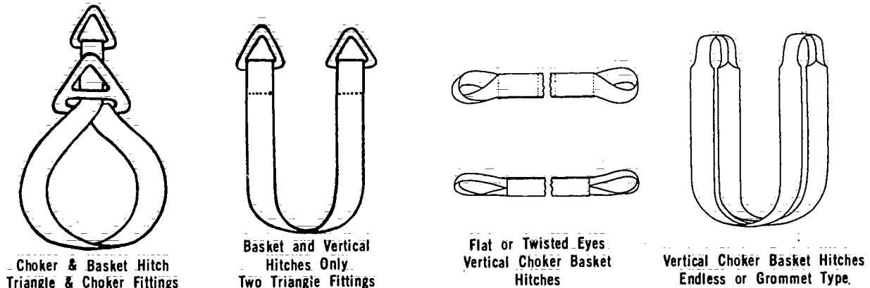
Figure 7-73. Synthetic Web Sling Constructions
