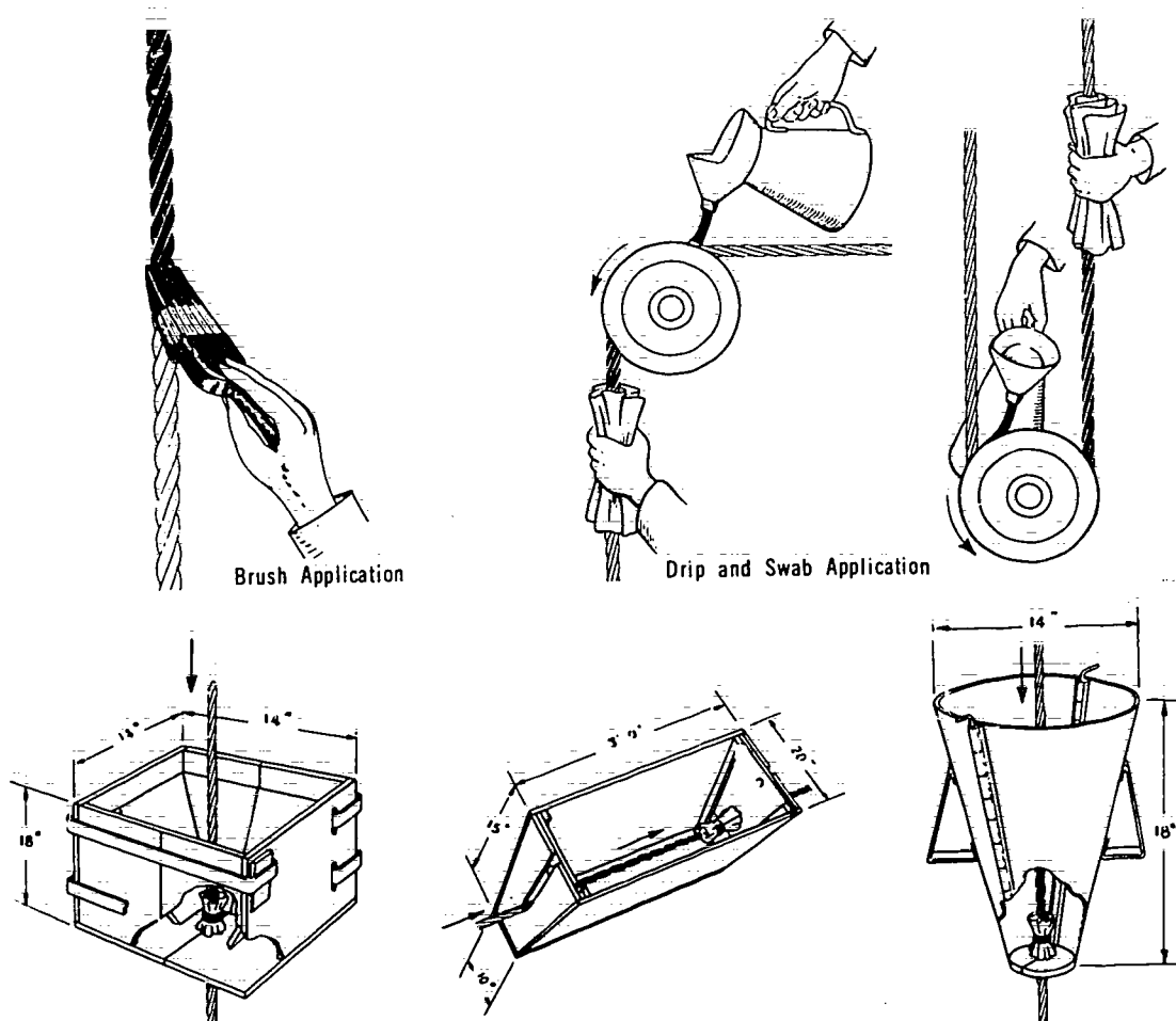
Split wooden or metal boxes. Rope passes through burlap or similar wiper at outlet end of box.
