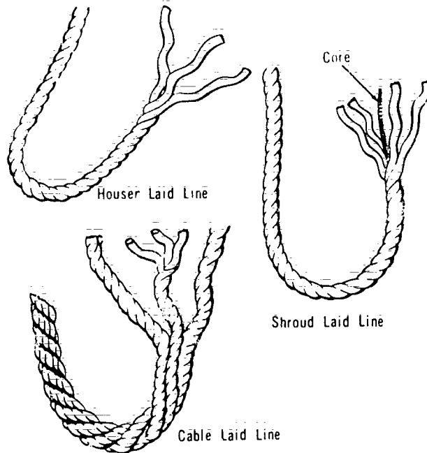
Figure 7-36. Forms of Natural Fibre Line
