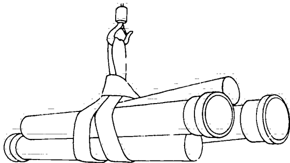
Figure 7-74. Synthetic Web Slings in Operation
