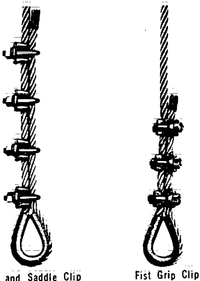
Figure 7-85. Clips For Wire Rope
