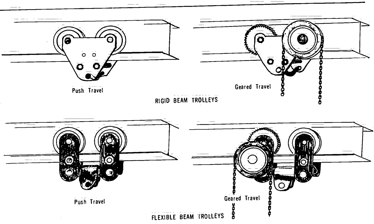
Figure 7-95. Beam Trolleys
