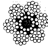
Figure 7-46. Armoured Core
