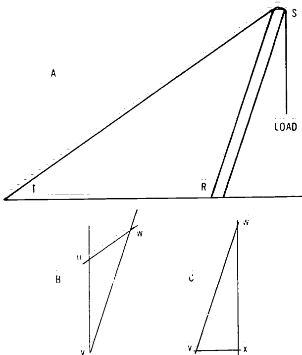
Figure 7-108. Determining the Kick at the Heel of a Gin Pole
