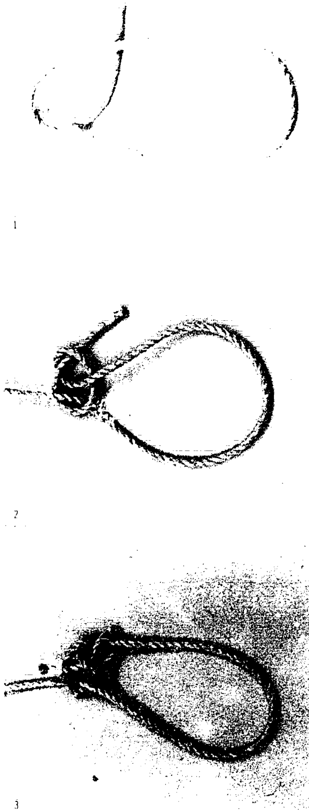
Figure 7-12. Tying a Running Bowline Knot
