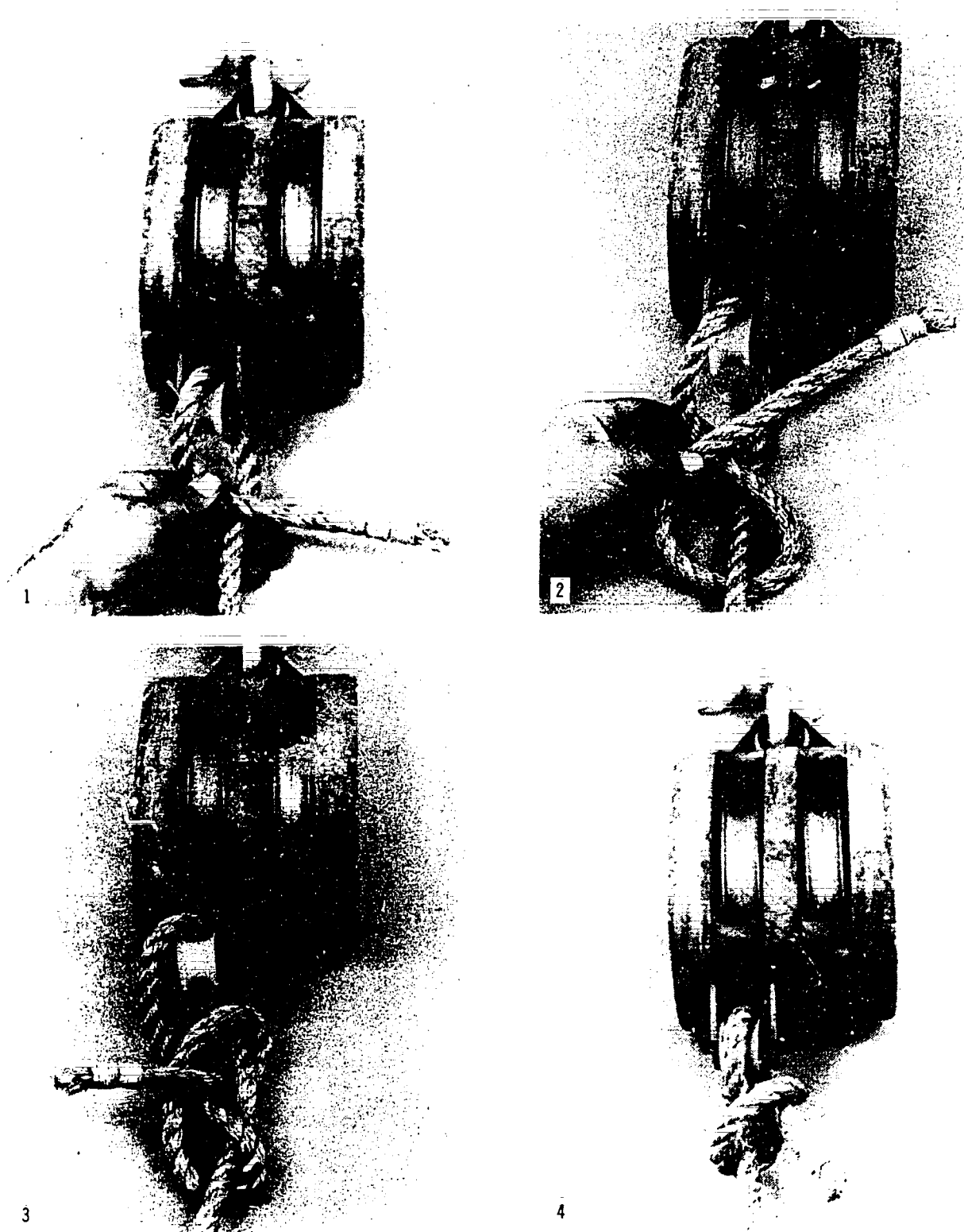
Figure 7-29. Tying a Becket Hitch
