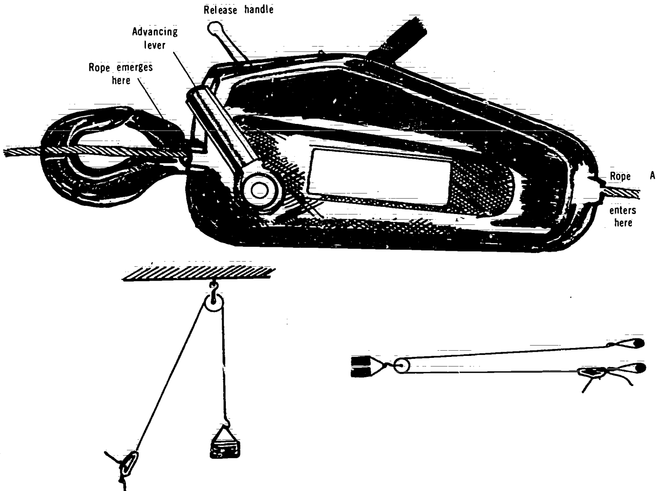
Figure 7-92. Tirfor Jack
