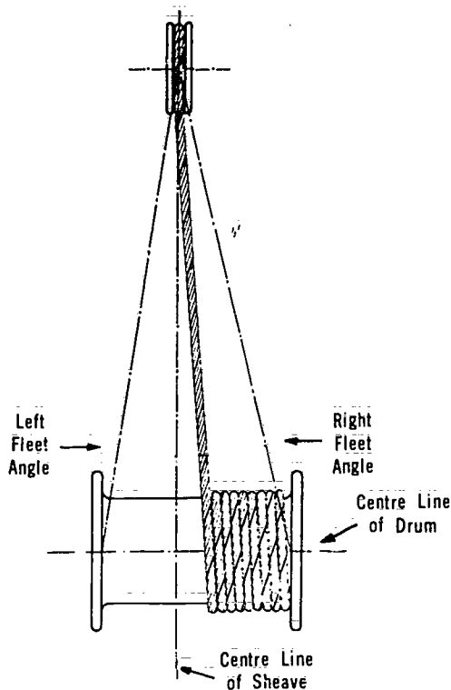
Figure 7-69. Fleet Angles
