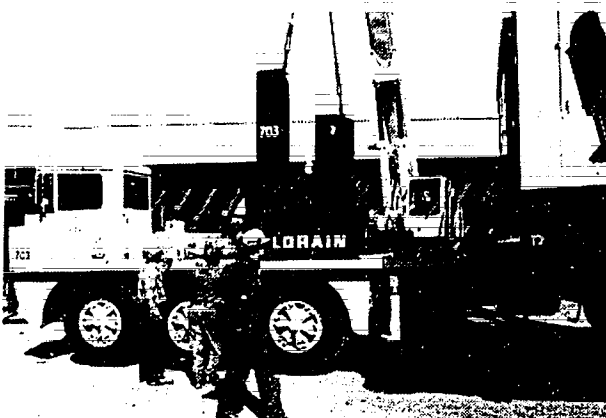
INSTALLING REAR COUNTERWEIGHT WITH SECOND RIG
