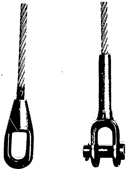
SPELTER SOCKET (closed type)
