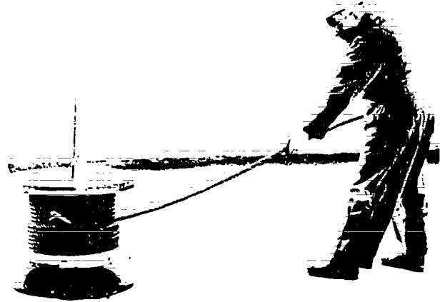
Figure 7-61. Unwinding Wire Rope-Method 3
