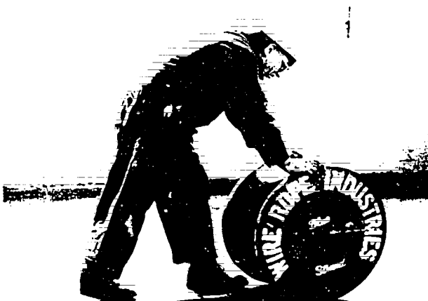
Figure 7-60. Unwinding Wire Rope-Method 2
