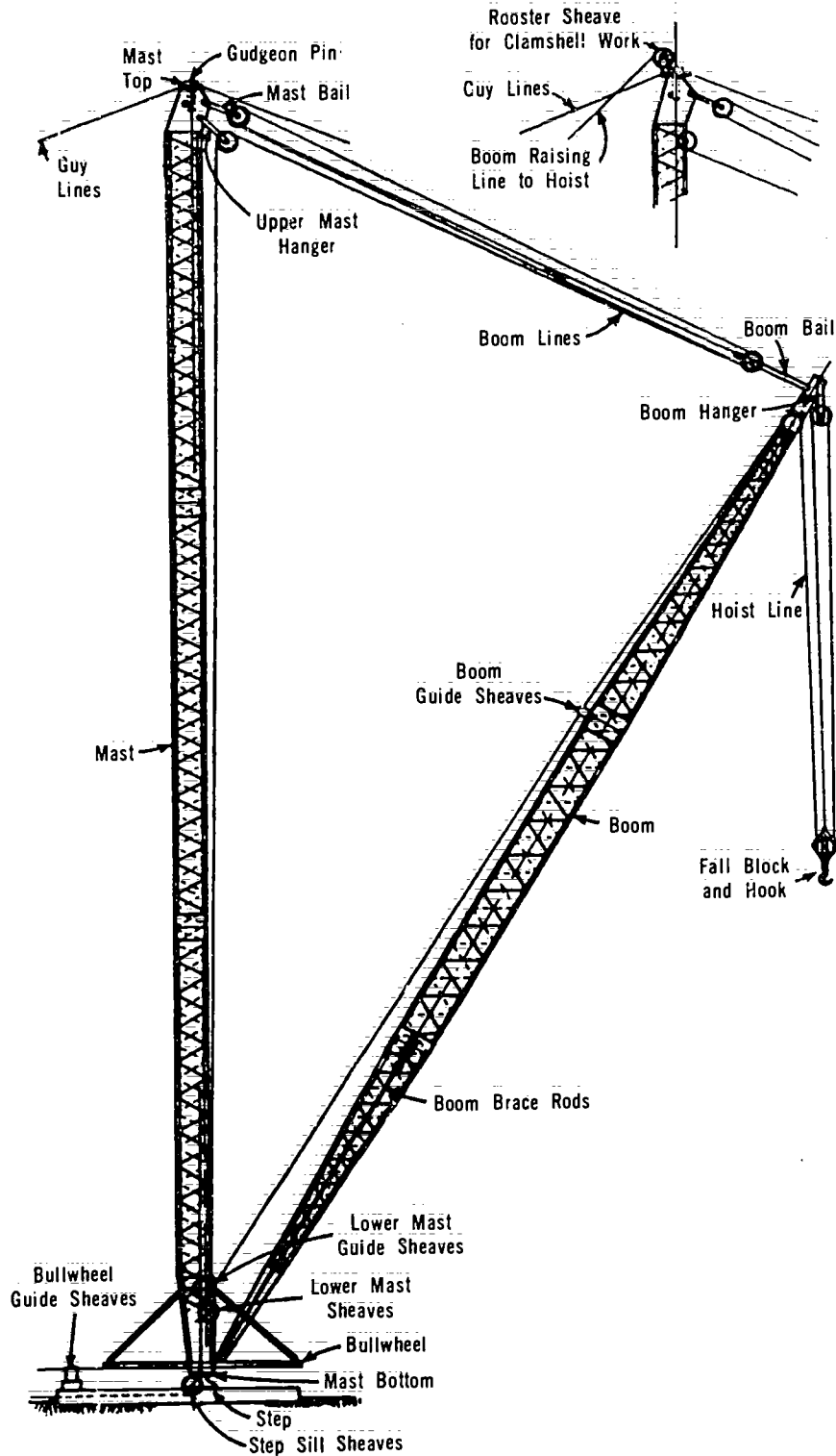
Figure 7-104. Sections of a Guy Derrick
