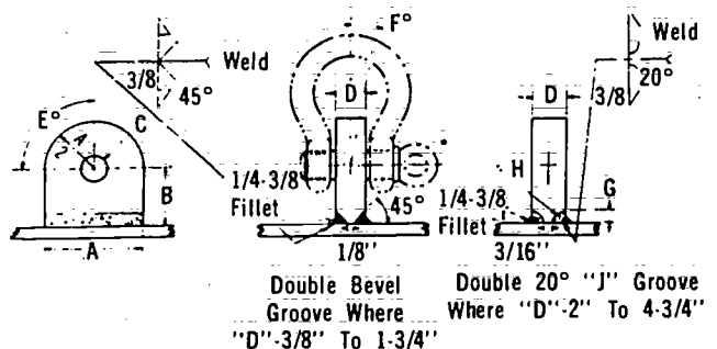
Figure 7-84. Dimensions for Welded Lugs
