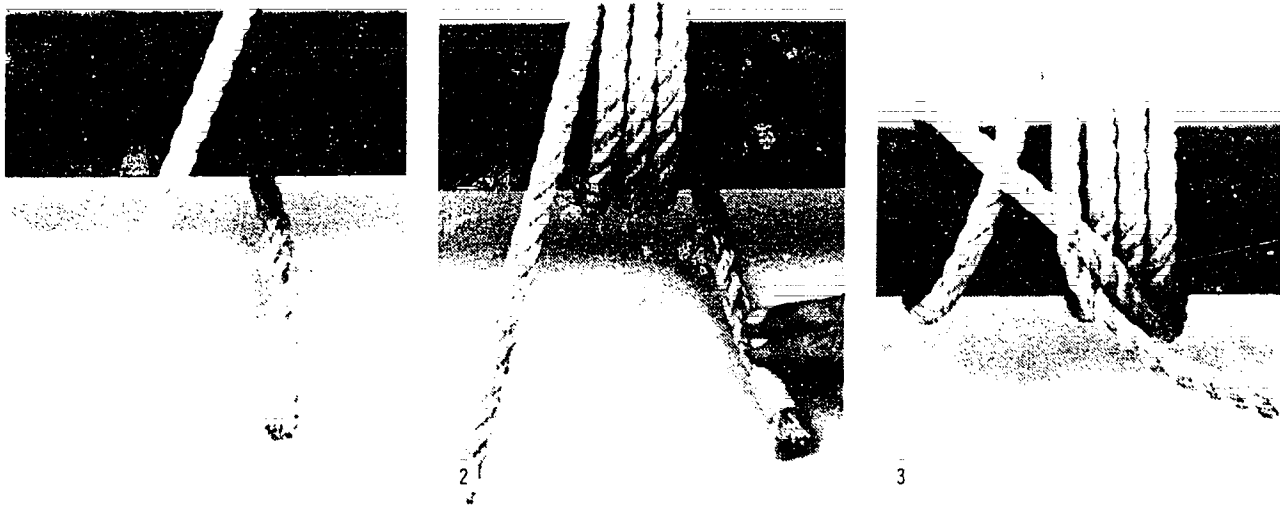
Figure 7-21. Tying a Rolling Hitch
