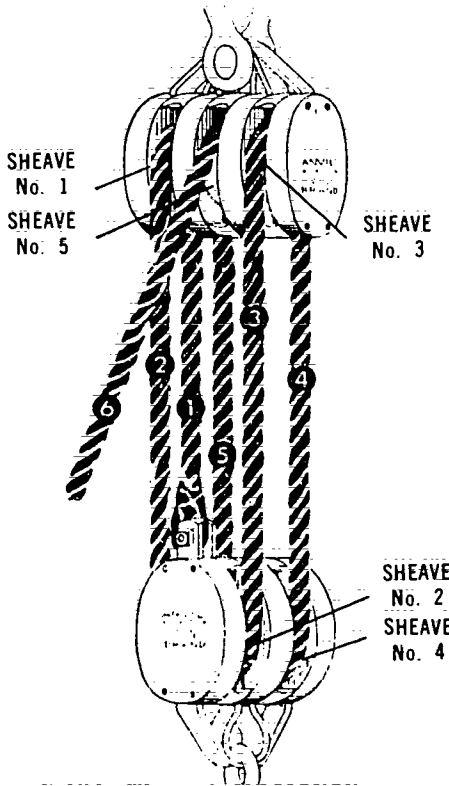
Figure 7-101. Sheave Operation
