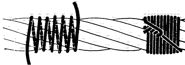
Figure 7-67. Stranding Rope-Method 2
