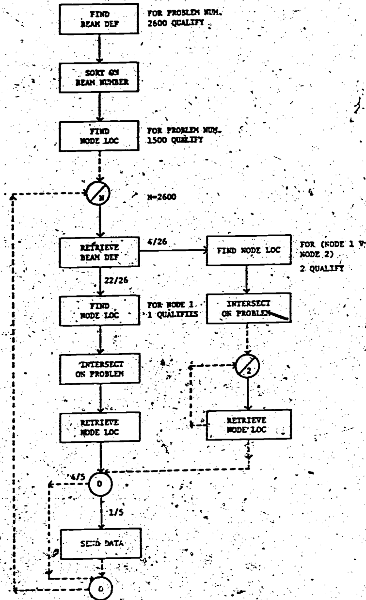
Figure 4.3.6-2 Revised Optimization Example (reference (1))
