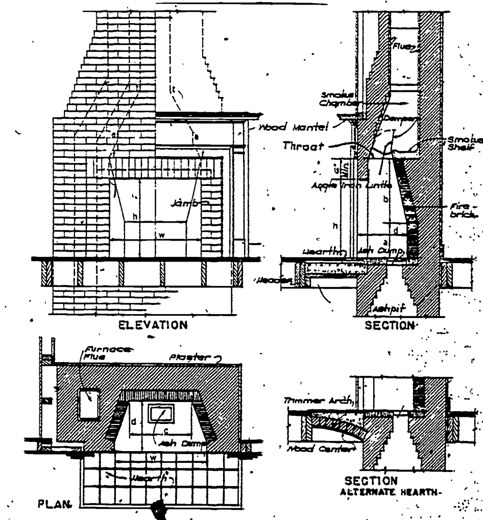
Recommended Dimensions For Fireplaces And Size of Flue Lining Required
