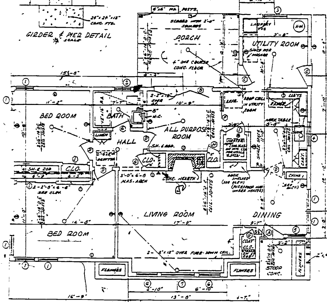
FLOOR PLAN SCALE
