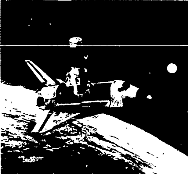
The large Space Telescope is being designed as an optical telescope observatory to be used in Earth orbit, unhindered by atmospheric distortion. Here, it is being shown deployed in orbit by the Space Shuttle.
