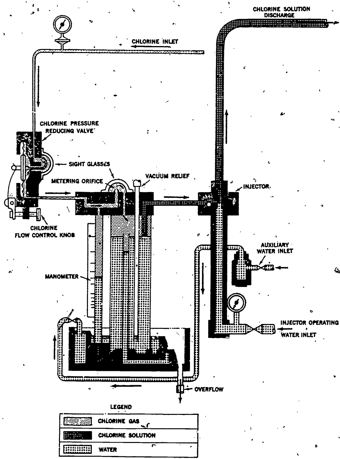
Vacuum Type, Mechanical Diaphragm Chlorinator, Manufactured by Wallace and Tiernan, Inc. (See Figure 4.)
