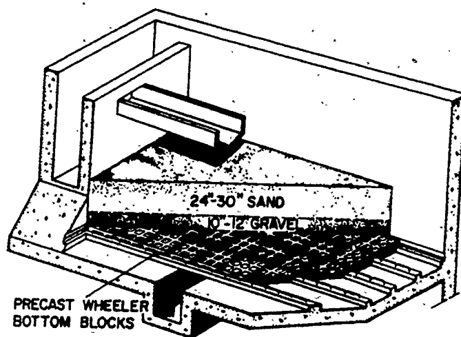
Figure 2. Cutaway of Gravity Type Filter
