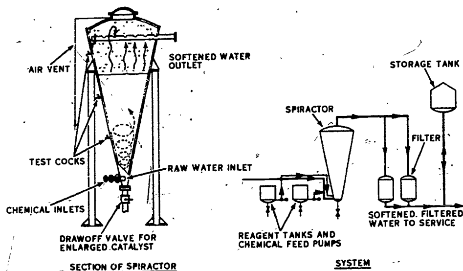
Figure 1. Spiractor Softener
