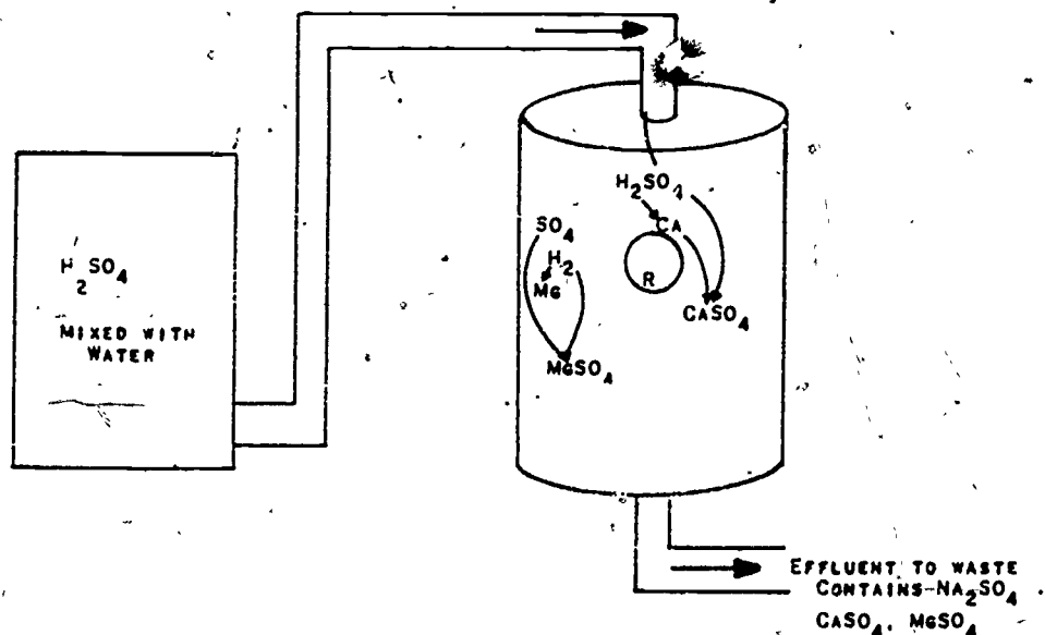
Figure 13. Regeneration with H_2SO_4
