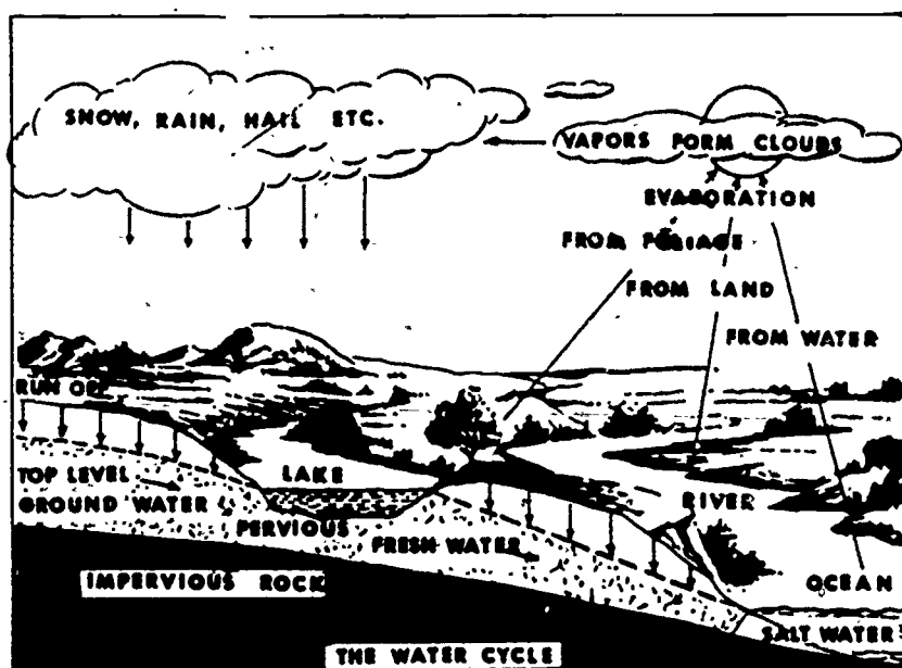
Figure 1. Hydrologic Cycle
