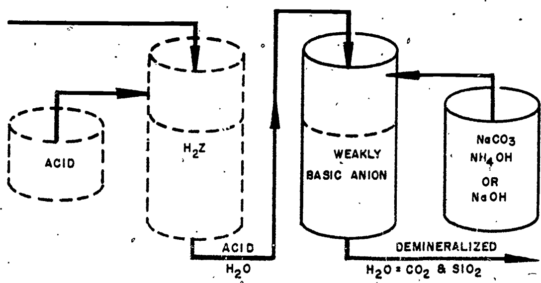
Figure 7. Weakly Basic Anion Process
