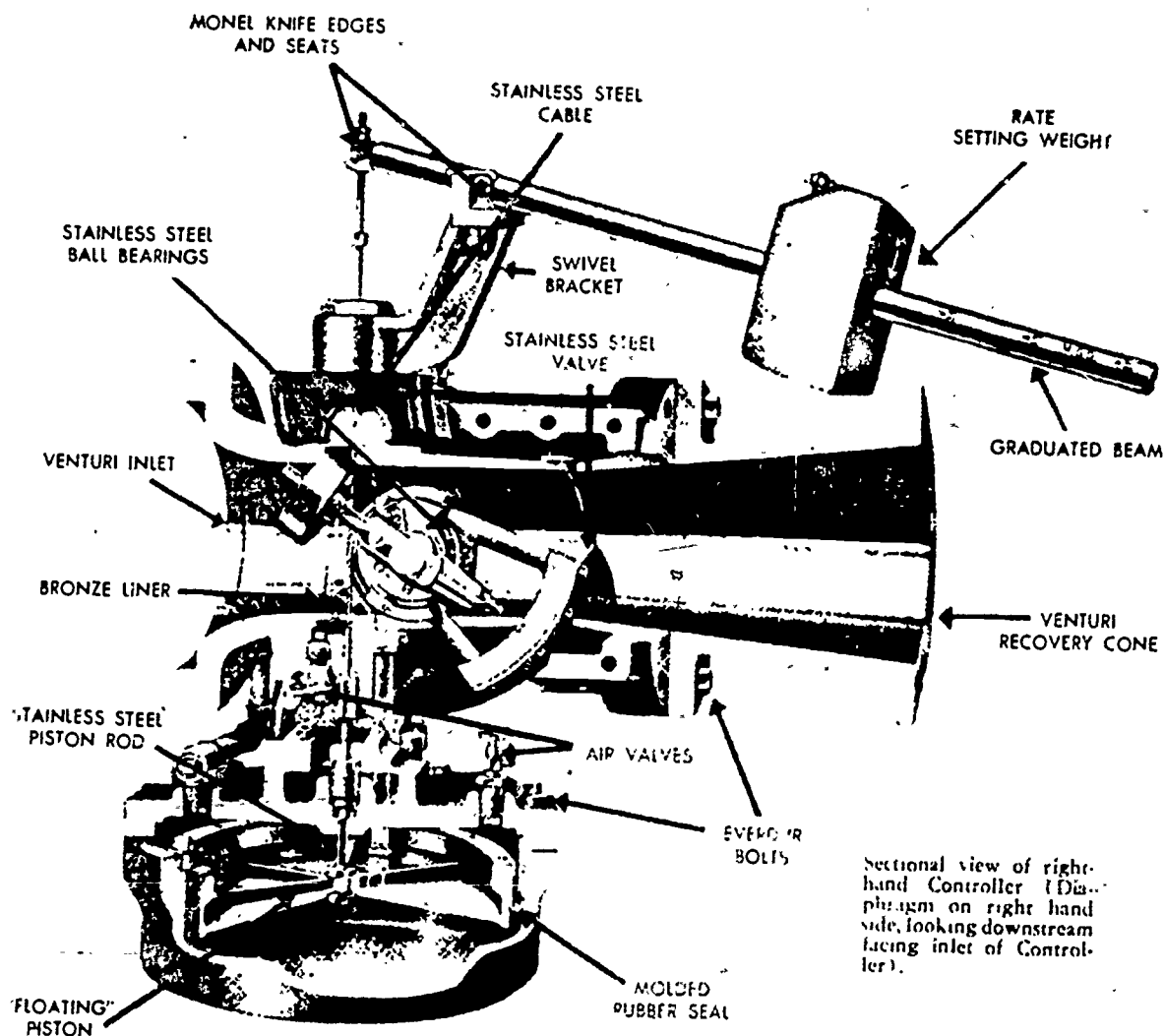
Figure 5. Rate-of-Flow Controller
