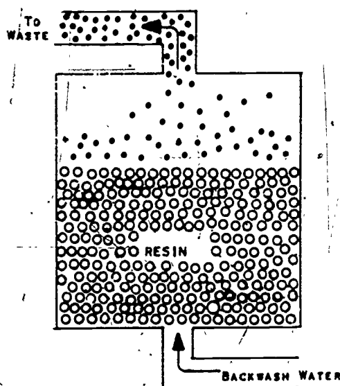
Figure 12. Deposits Being Removed from Resin Surface by Backwashing
