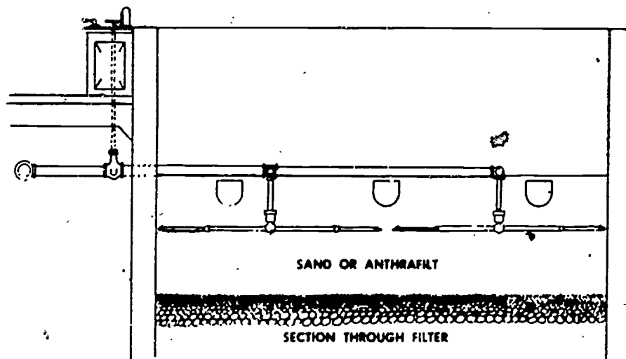
Figure 16. Surface Wash. 50
