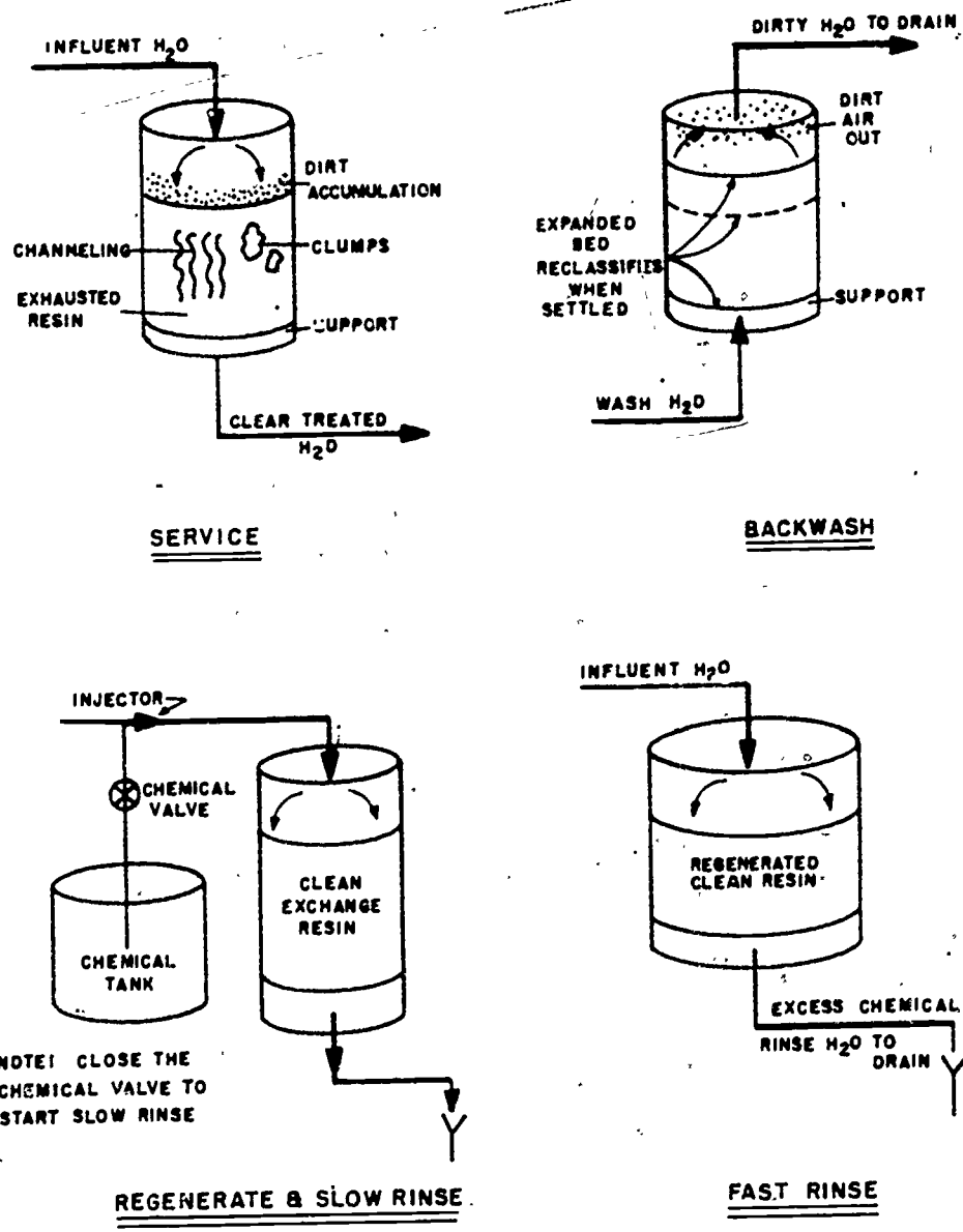
Figure 3. Regeneration Cycle
