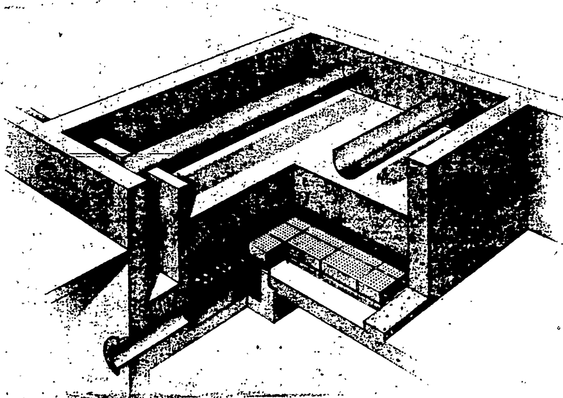
Figure 4. Underdrain System
