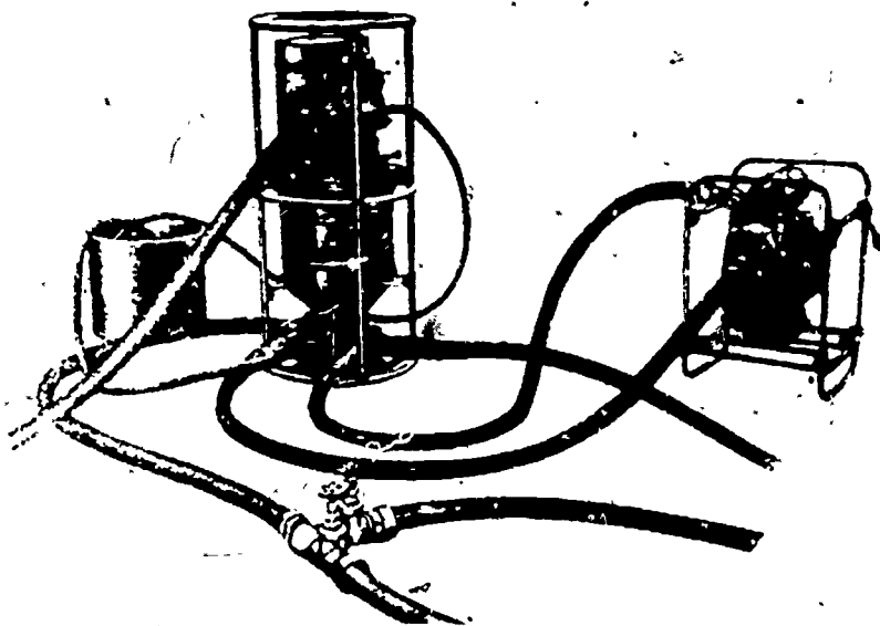
Diatomite water purification set No. 3, 35 gpm
