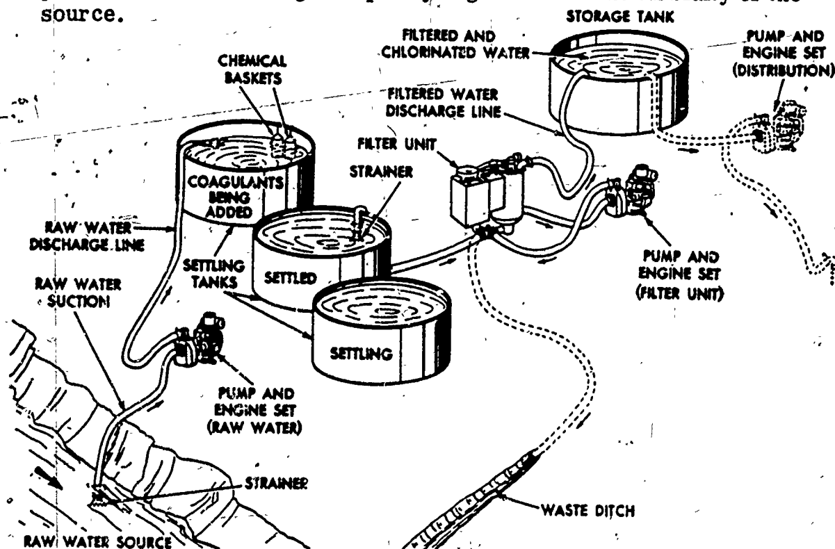
Figure 10. Portable Water Purification Equipment
