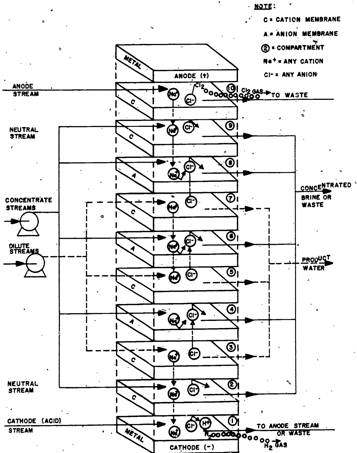
Figure 4. Water and Ion Flow in an Electric Membrane Stack
