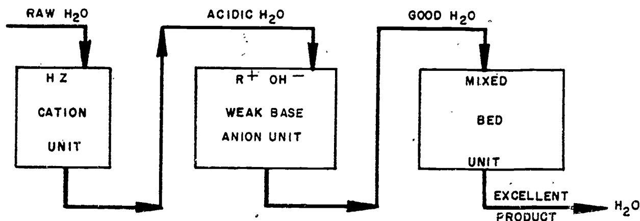
• Figure 9. Combination Demineralizers
