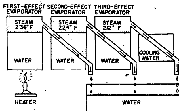
Figure 3. Multiple Effect Distillation Unit
