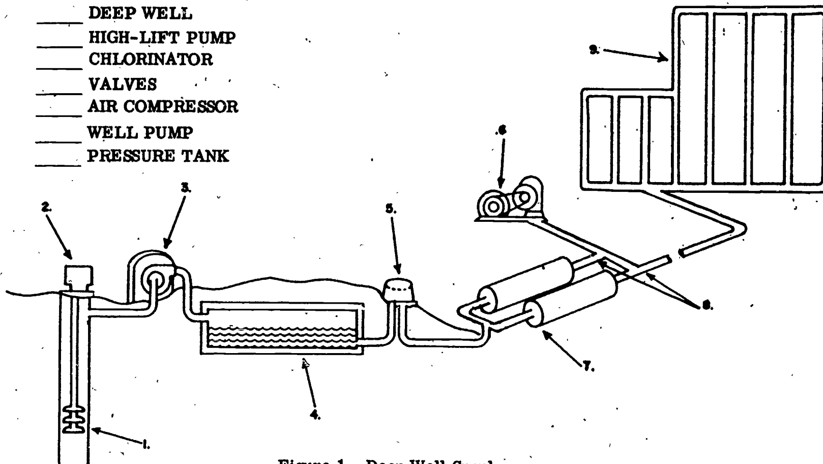
Figure 1. Deep Well Supply
