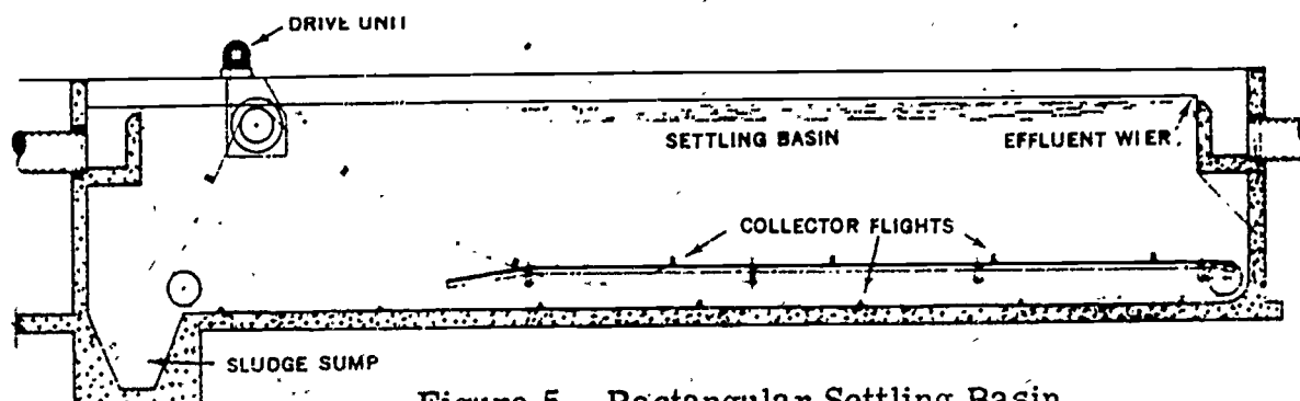
Figure 5. Rectangular Settling Basin
