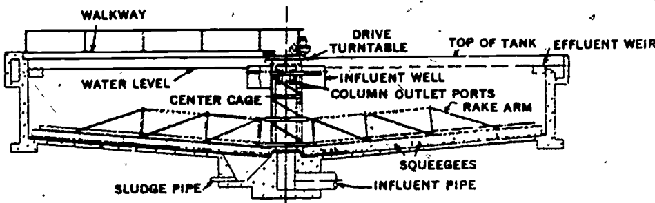
Figure 4. Circular Settling Basin
