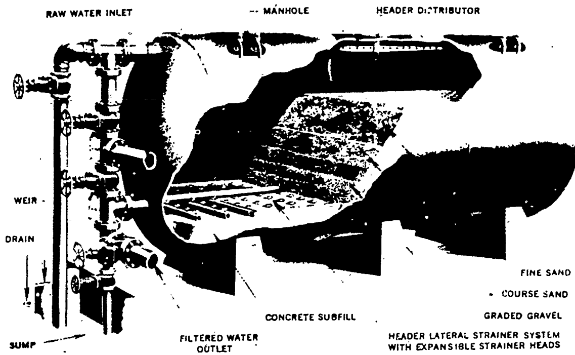
VERTICAL PRESSURE FILTER
