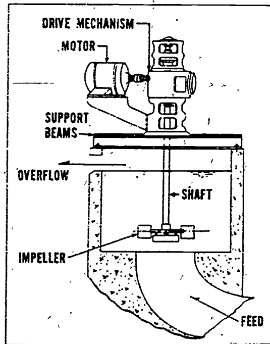
Figure 2. Flash Mixer
