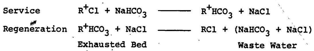
Figure 6. Chloride Dealkalizer
