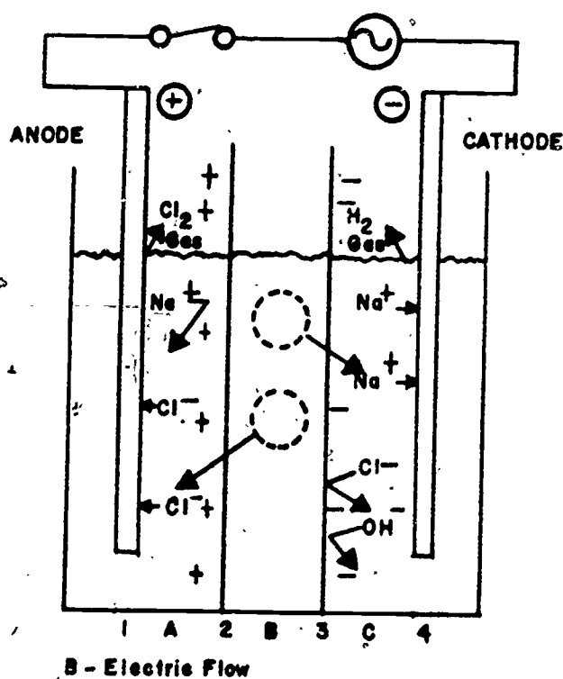
Figure 3. Basic Operation of Permeable Membrane
