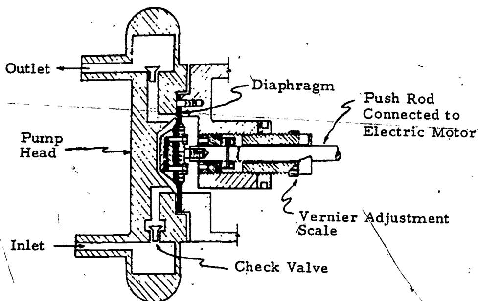
Figure 6. Cross Section of Typical Diaphragm Pump
