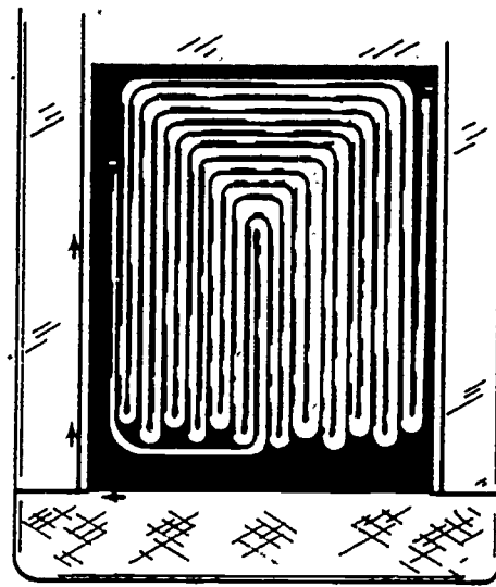
Figure 7. Horse Shoe Load Construction. 21
