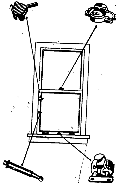
Figure 19. Locking Devices for Checkrail Windows.
