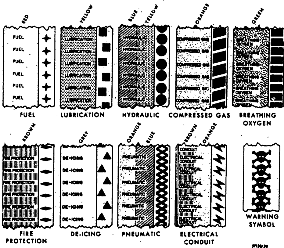
Figure 6. Color Code for Aircraft Tubing and Hose.
