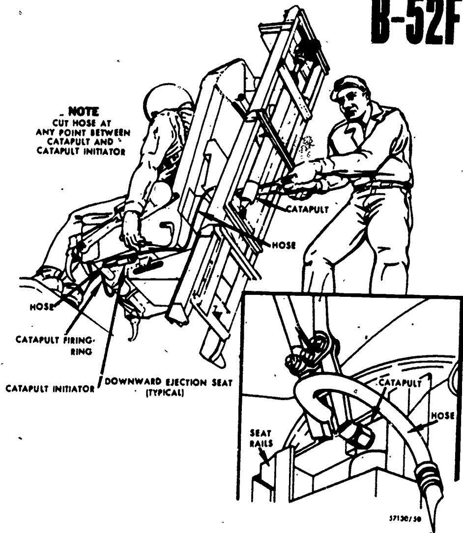
Figure 12. Cutting the Initiator Hose.
