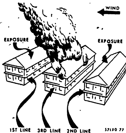
Figure 24. Protecting External Exposures.
