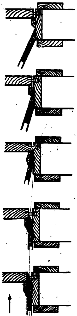
PUSH Figure 16. Springing a Door In a Spanned Frame.
