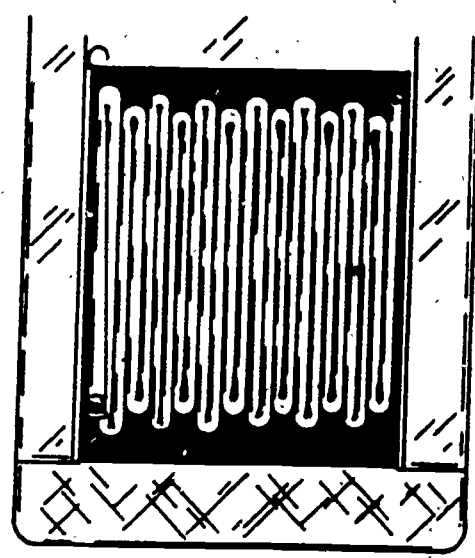
Figure 8. Accordion Load Construction.
