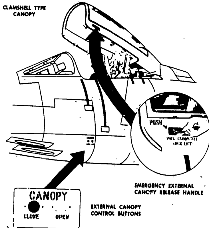
Figure 8. Manual and Electrical Canopy Controls.
