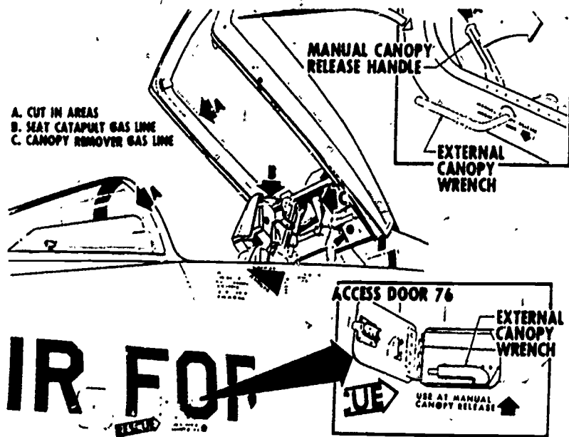
Figure 9. Manual Canopy Release.
