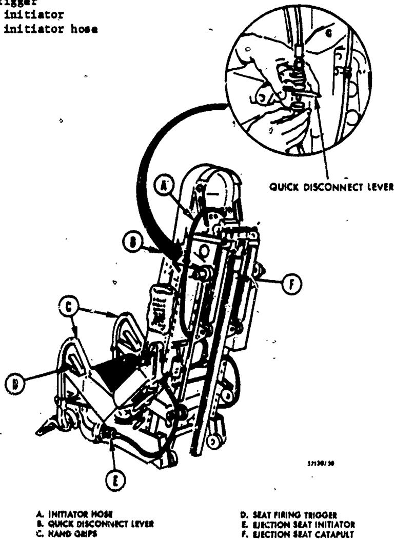
Figure 11. Seat Ejection System.
