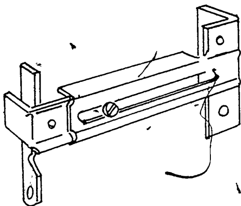
Traverse Bracket Used with a regular traverse rod.
