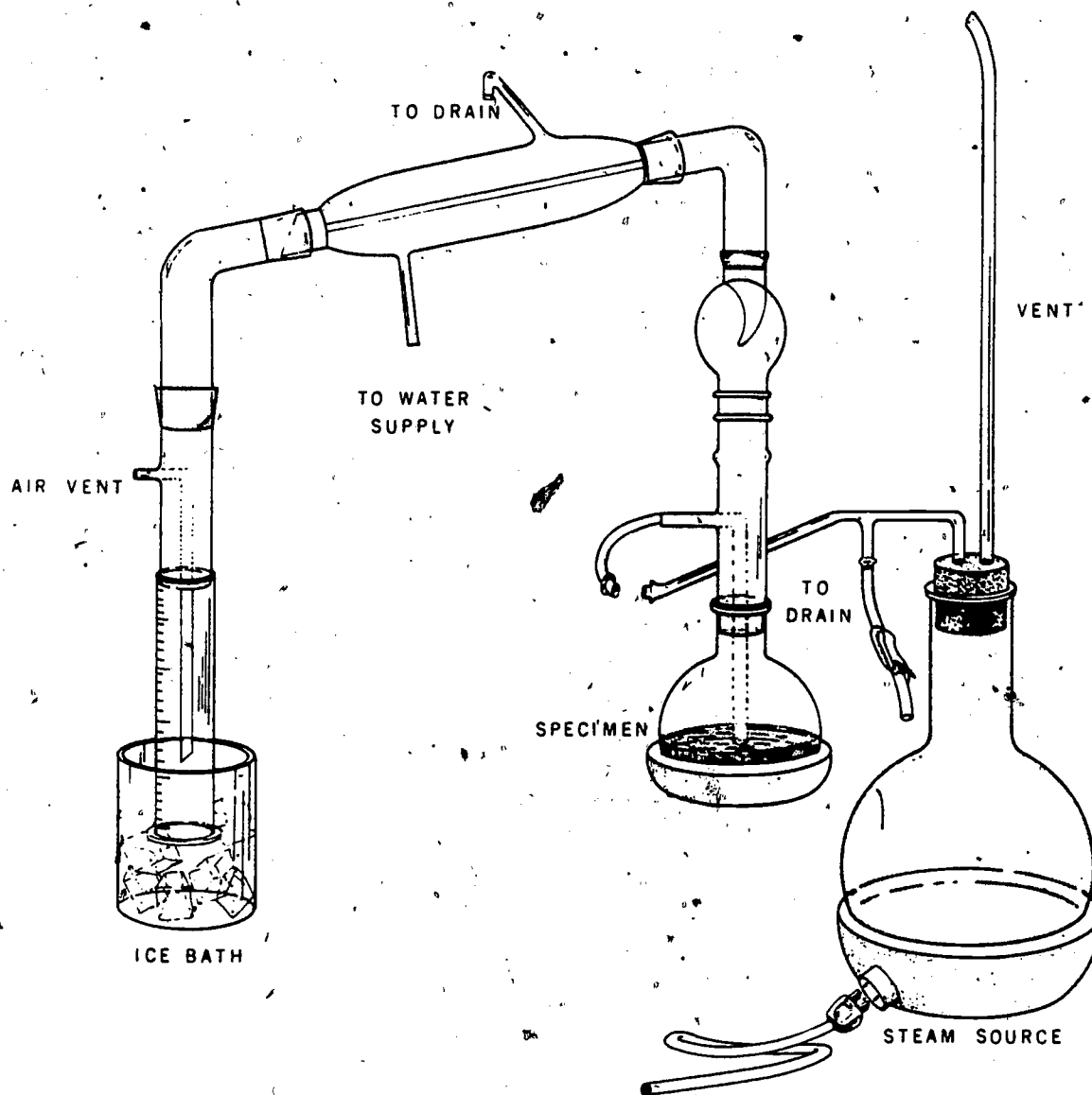
Figure 12. Distillation apparatus.
