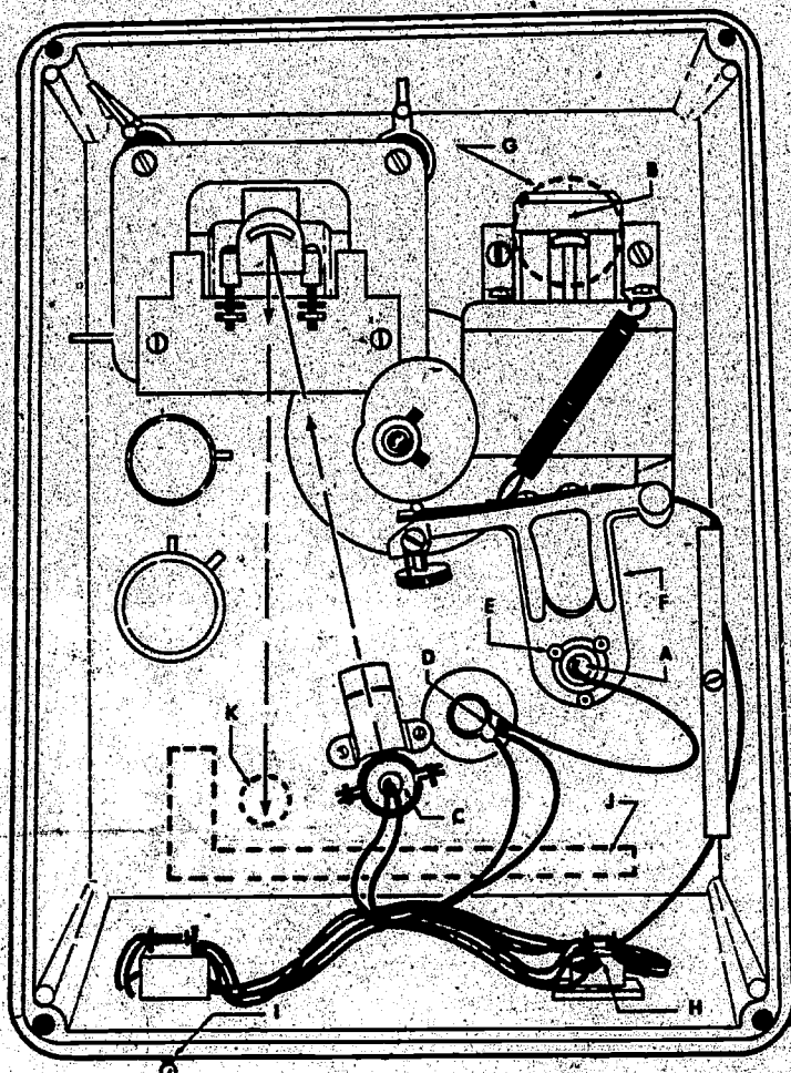
Figure 17. Bottom view of the Coleman, Jr. spectrophotometer.
