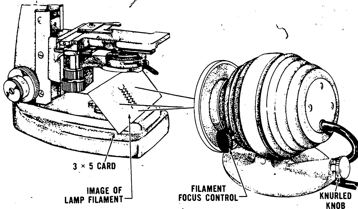
Figure 2. Microscope lamp illumination.
