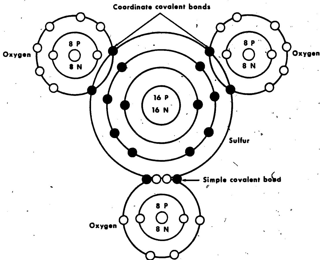
Figure 6. Coordinate covalent bonding in the SO 2 molecule.
