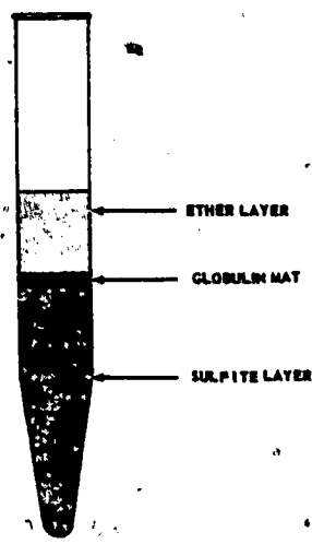
Figure 9. Diagram of tube in which globulins have been "salted out" from a serum protein solution with 26.9 percent \text{Na}_2\text{SO}_4 .
