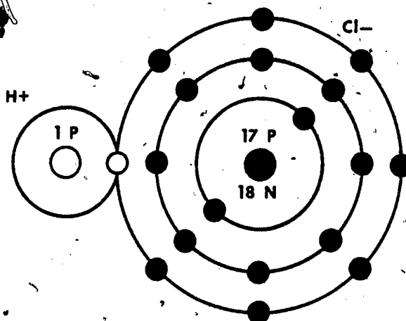
Figure 5. Covalent bonding in the HCl molecule.
