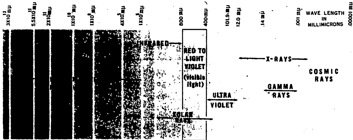
Figure 11. Position of visible spectrum with reference to other wavelengths of energy.
