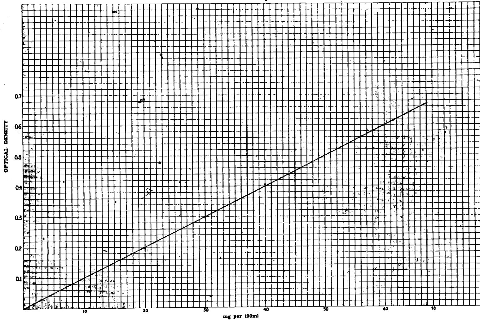
Figure 13. Concentration-absorbance curve.
