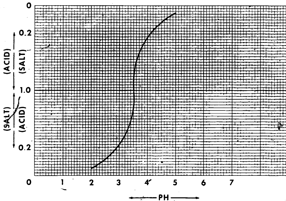
Figure 10. Approximate efficiency curve for a buffer of pK_a = 3.5 pH units.
