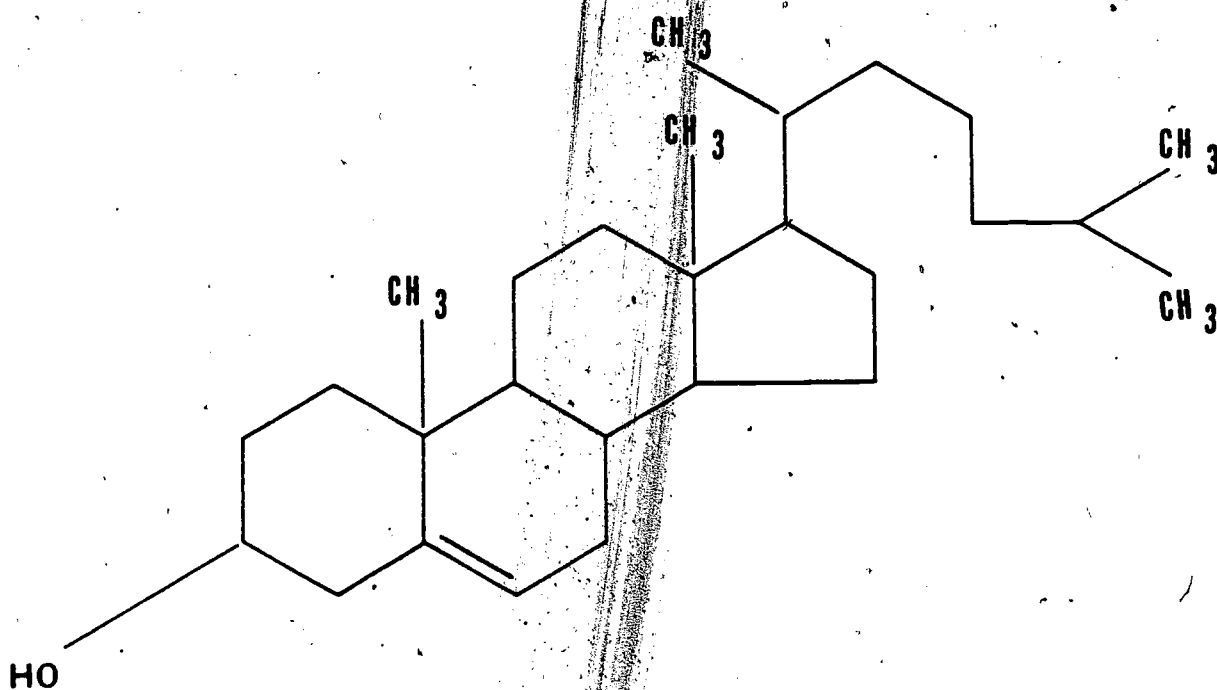
Figure 6. Cholesterol (C 27 H 46 O).
