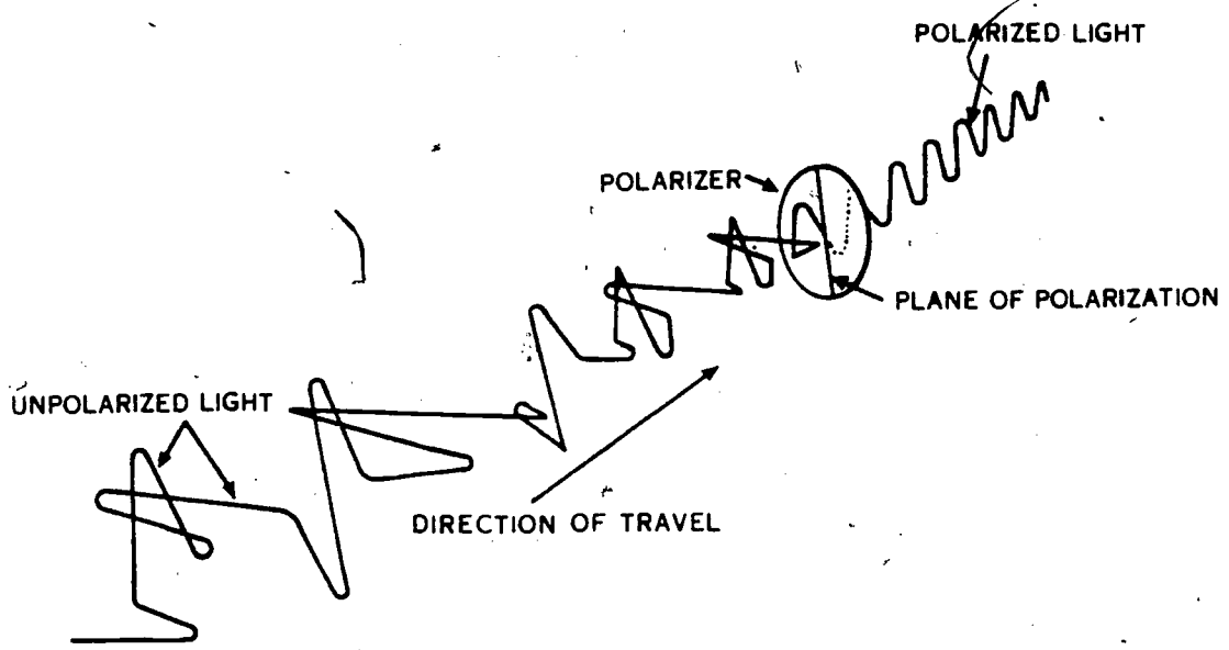
Figure 11. Diagram illustrating principle of polarization.
