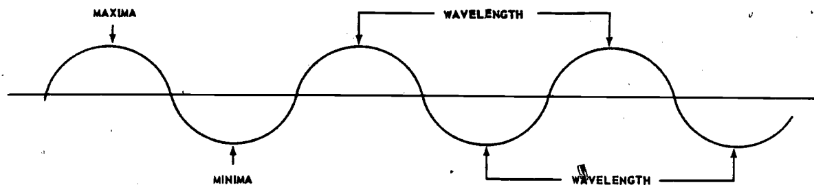
Figure 12. Diagrammatic representation of light waves, showing principle of wavelength measurement.
