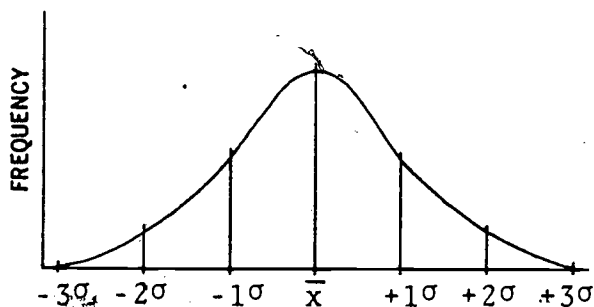
Figure 19. Frequency distribution curve.
