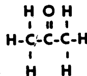
Figure 9. Structural formula for acetone.
