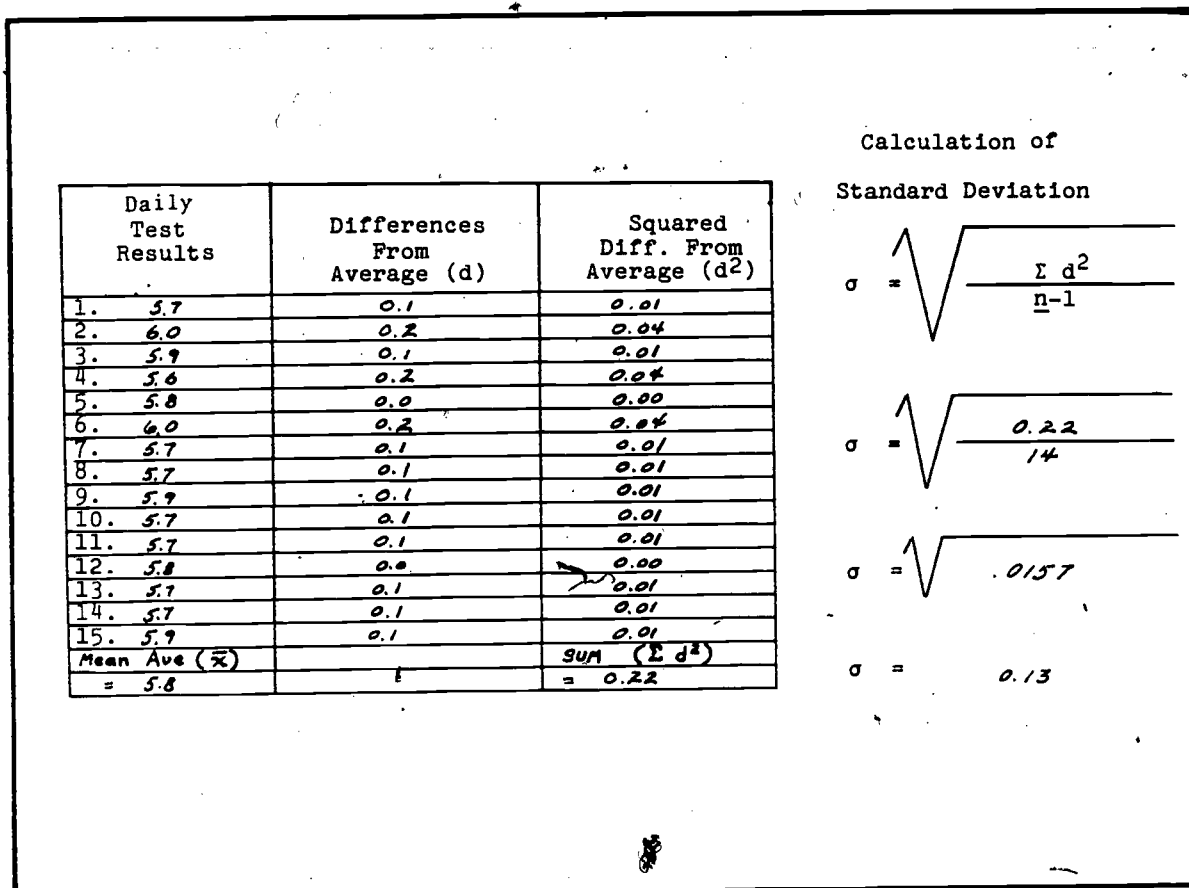
Figure 20. Data chart for entering test results and expressing standard deviation (values for potassium are entered).
