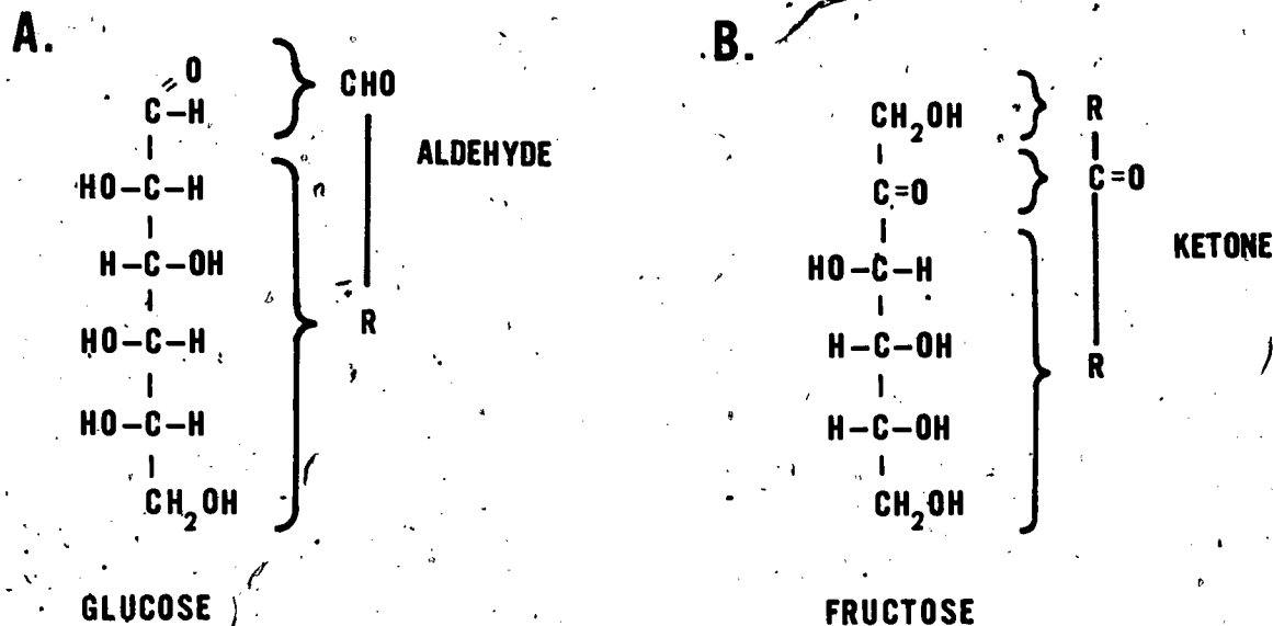
Figure 20. Relationship between the general formulas for (A) aldehyde with glucose and (B) keto- with fructose.
