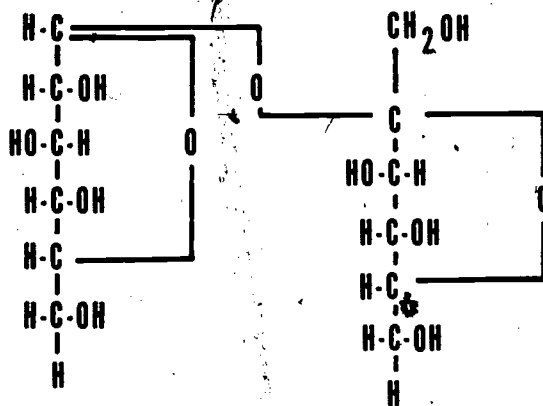
Figure 10. Structural formulas of a monosaccharide, D-(+) glucose, and a disaccharide sucrose.
