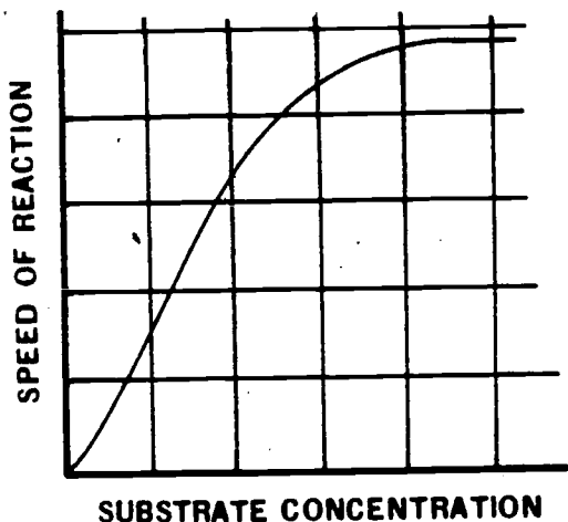
Figure 15. Effect of substrate concentration of enzyme activity.
