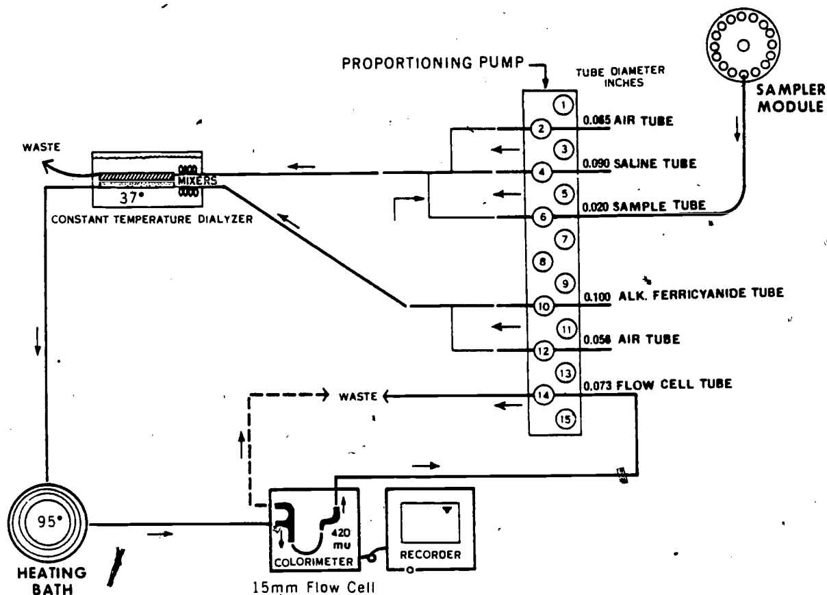
Figure 14. Ferricyanide method for glucose.
