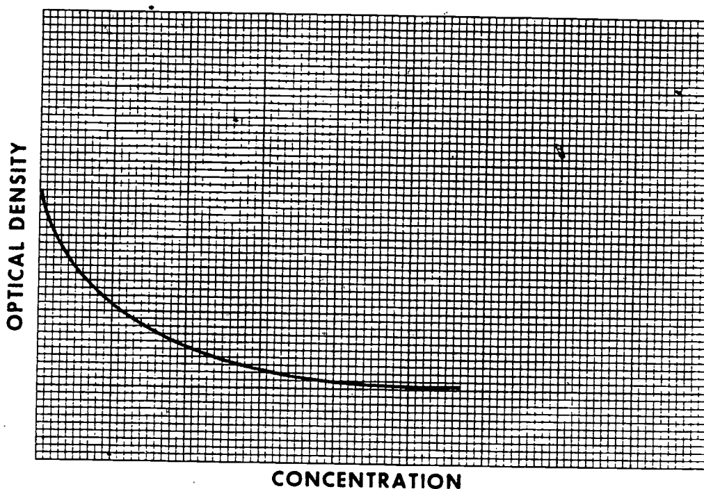
Figure 14. Nonlinear curve as used in enzyme studies.
