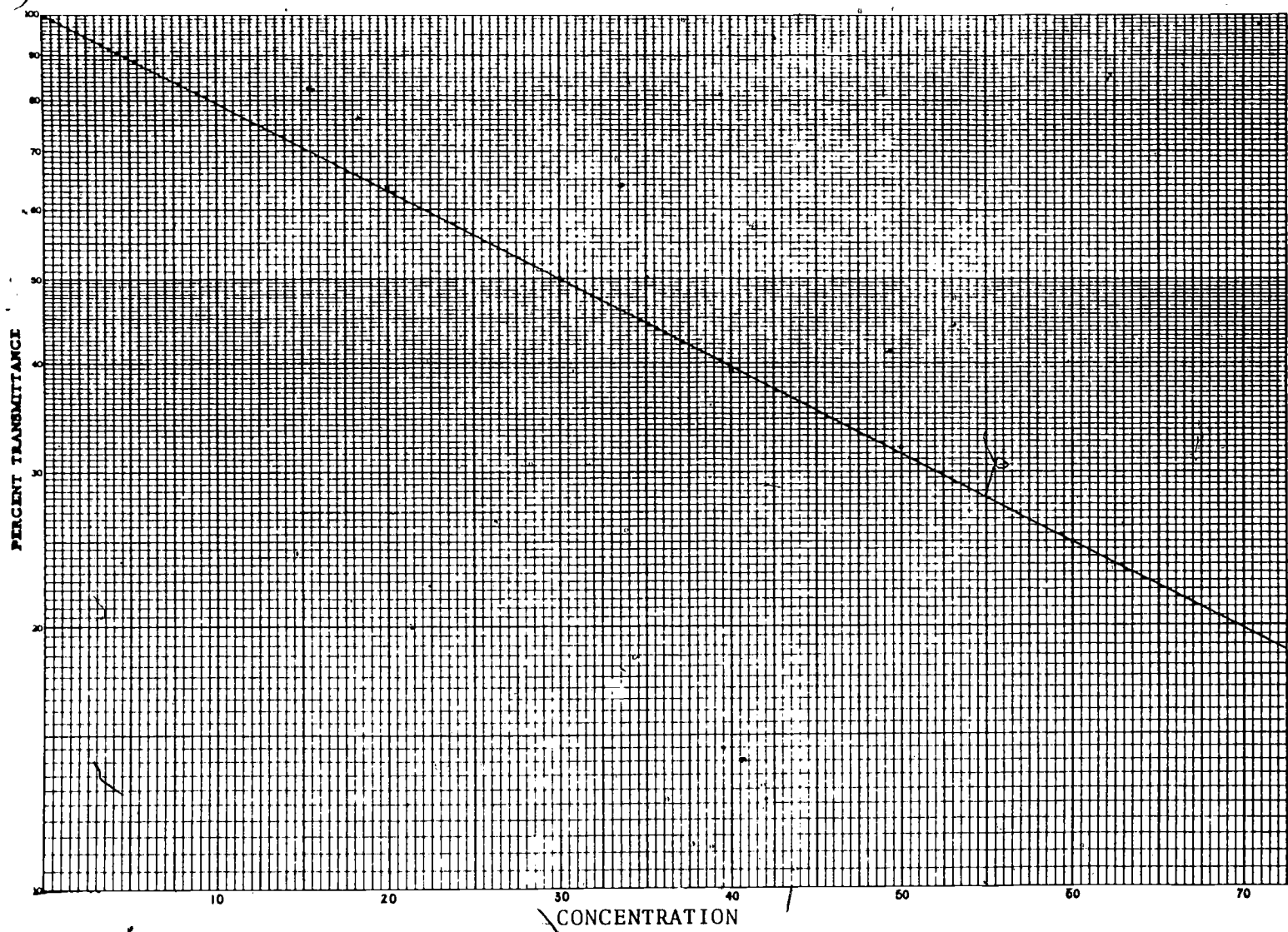
Figure 15. Concentration transmittance curve.
