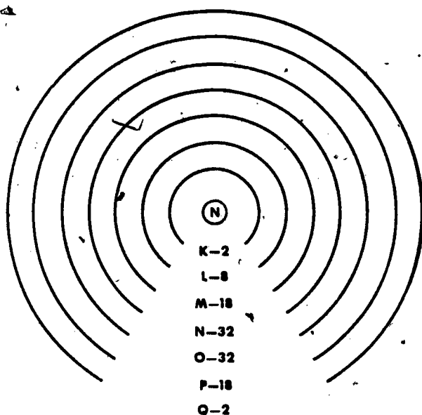
Figure 3. Energy shells by alphabetical designation.
