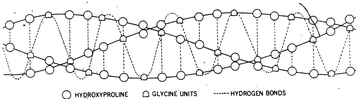
Figure 8. Diagram showing helix structure of a protein molecule.
