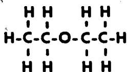
Figure 8. Structure of diethyl ether.
