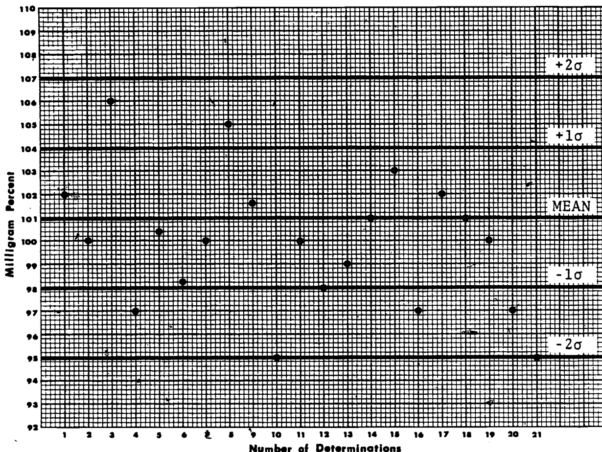
Figure 21. Quality control chart for glucose.
