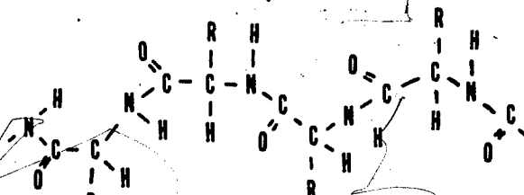
Figure 7. Portion of repeating chain of amino acids in polypeptide linkage.
