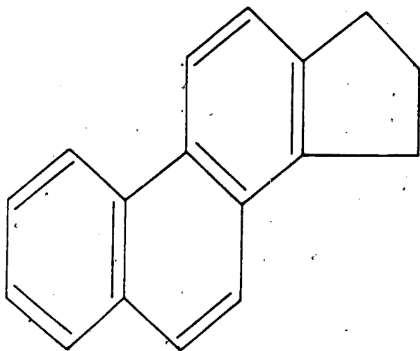
Figure 6. Structure of the cyclopentenophenanthrene ring.
