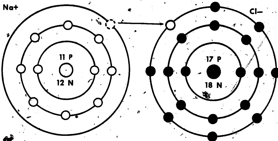
Figure 4. Electrovalent bonding in the NaCl molecule.
