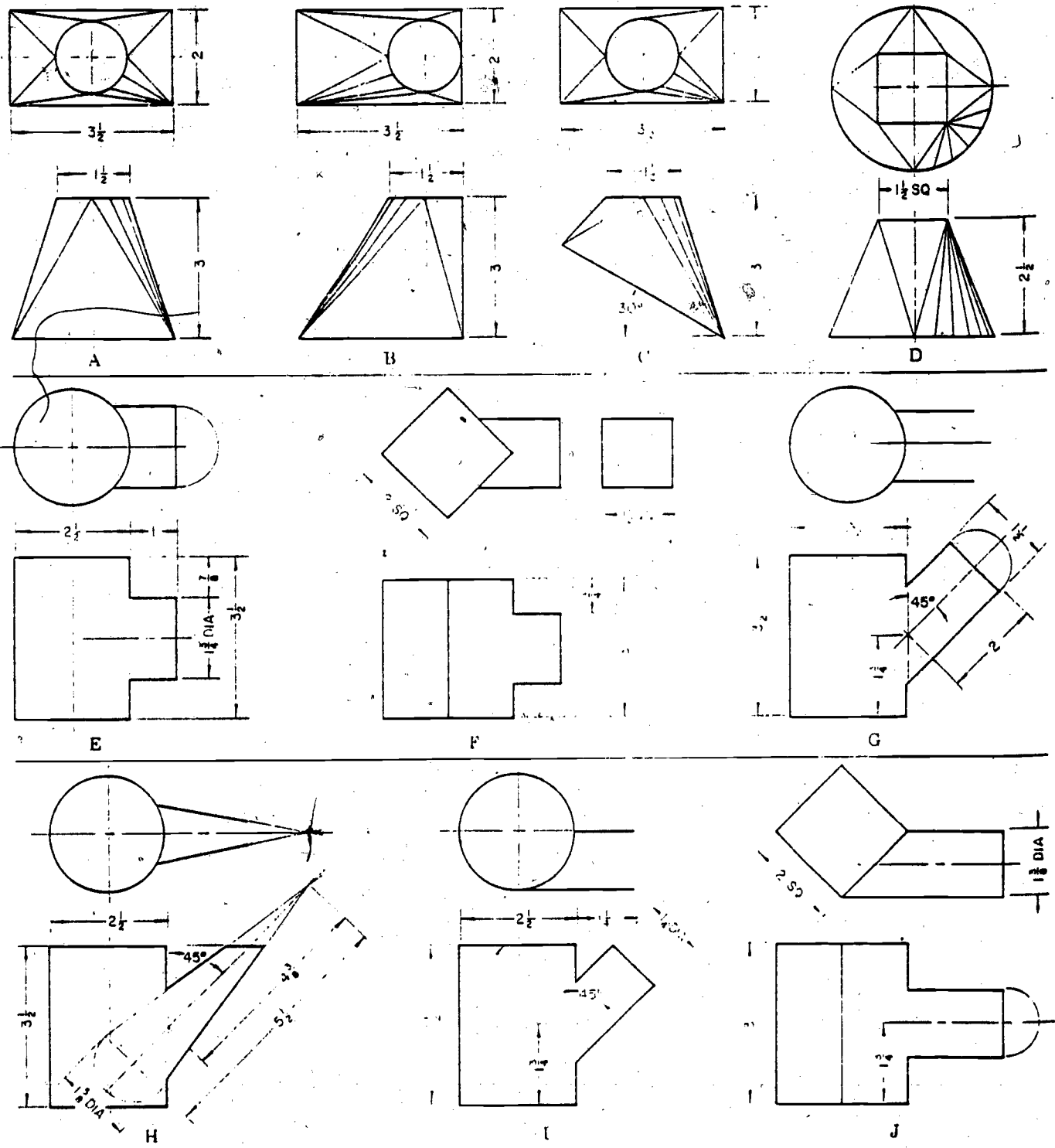
Fig. 18-55 Make two views of the problem assigned. In problems A through D, complete the top view and develop the pattern. In problems E through J, complete views where necessary by developing the line of intersection and completing the top view in G, H, and I. Develop patterns for both parts in problems E through J.
