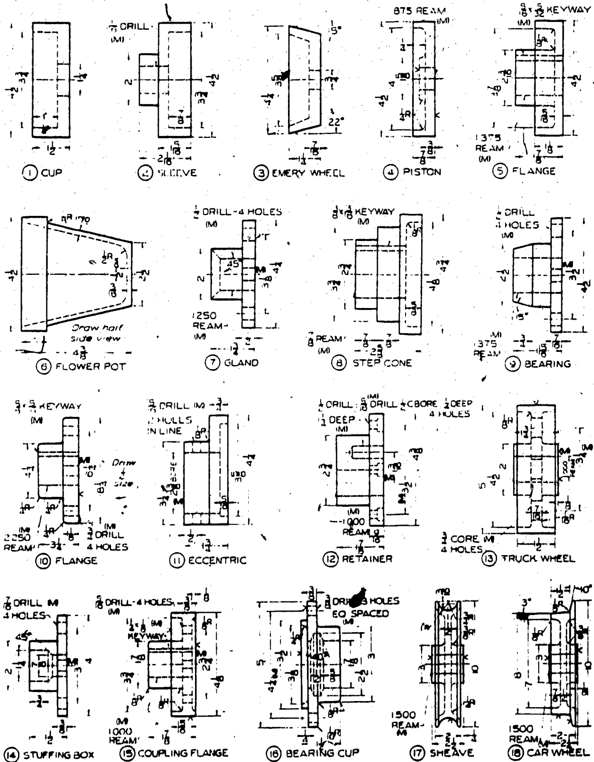
Fig. 11-24. Sectioning Problems. Page 204, Spencer. Make sketch or mechanical drawing of problem assigned from above. In each case draw a circular view and a full or half section as assigned. Vertical dimensions are diameters. Dimensions marked (M) should be moved to circular view. Holes are equally spaced. Give part names in title strips.
