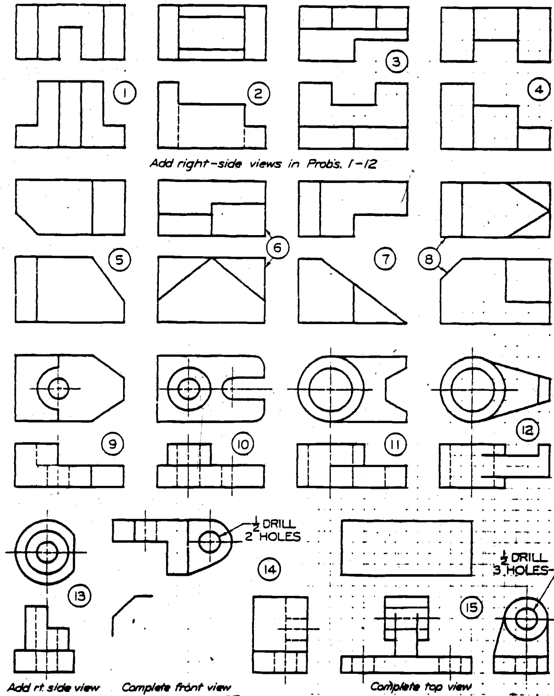
Fig. 6-28. Missing-View Problems. Sketch the given views, and then add the third view in each problem. Use cross-section paper or plain paper, as assigned. In most cases, spacing between views can be improved by spacing views farther apart than shown here. Each grid space = 1/4".
