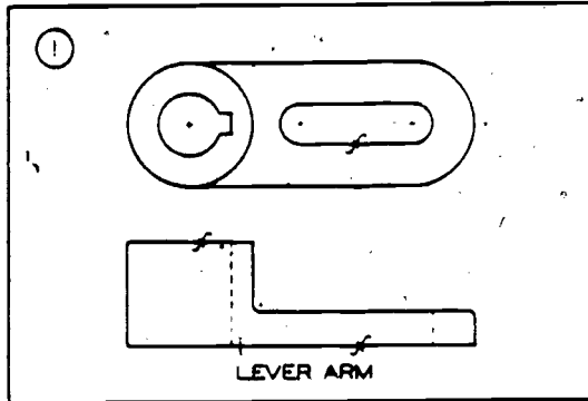
Fig. 9-41, p. 167, Dimensioning
