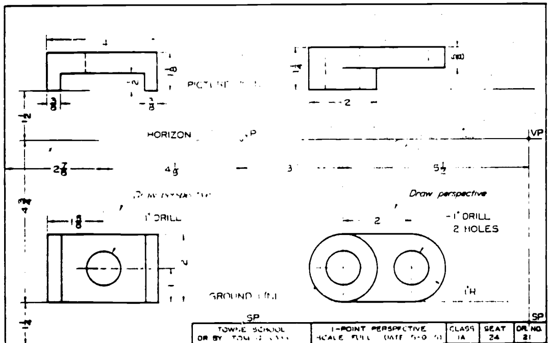
Fig. 16-55, p. 339, Basic Technical Drawing , Spencer. One-Point Perspective Problems. Omit all dimensions. Letter VPL, SP, etc.
