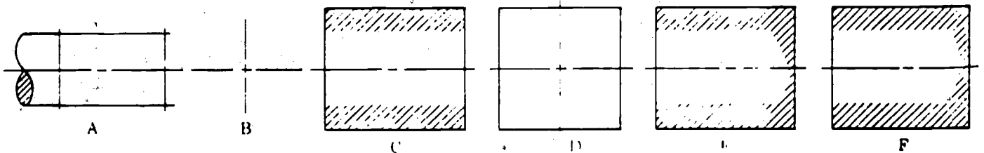
Fig. 10-49 Simplified representation of screw threads. Take dimensions from the printed scale at the bottom of the page, using dividers. Draw the views as shown and complete each as follows: A = simplified representation showing 1"-8UNC-2A threads; B = end view of A; C = simplified representation of
