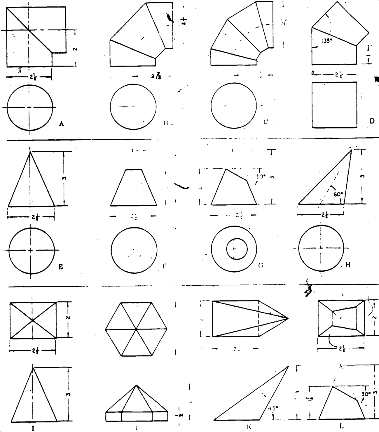
Fig. 18-54 Make two views of the problem assigned and develop the pattern. Scale: full size.
