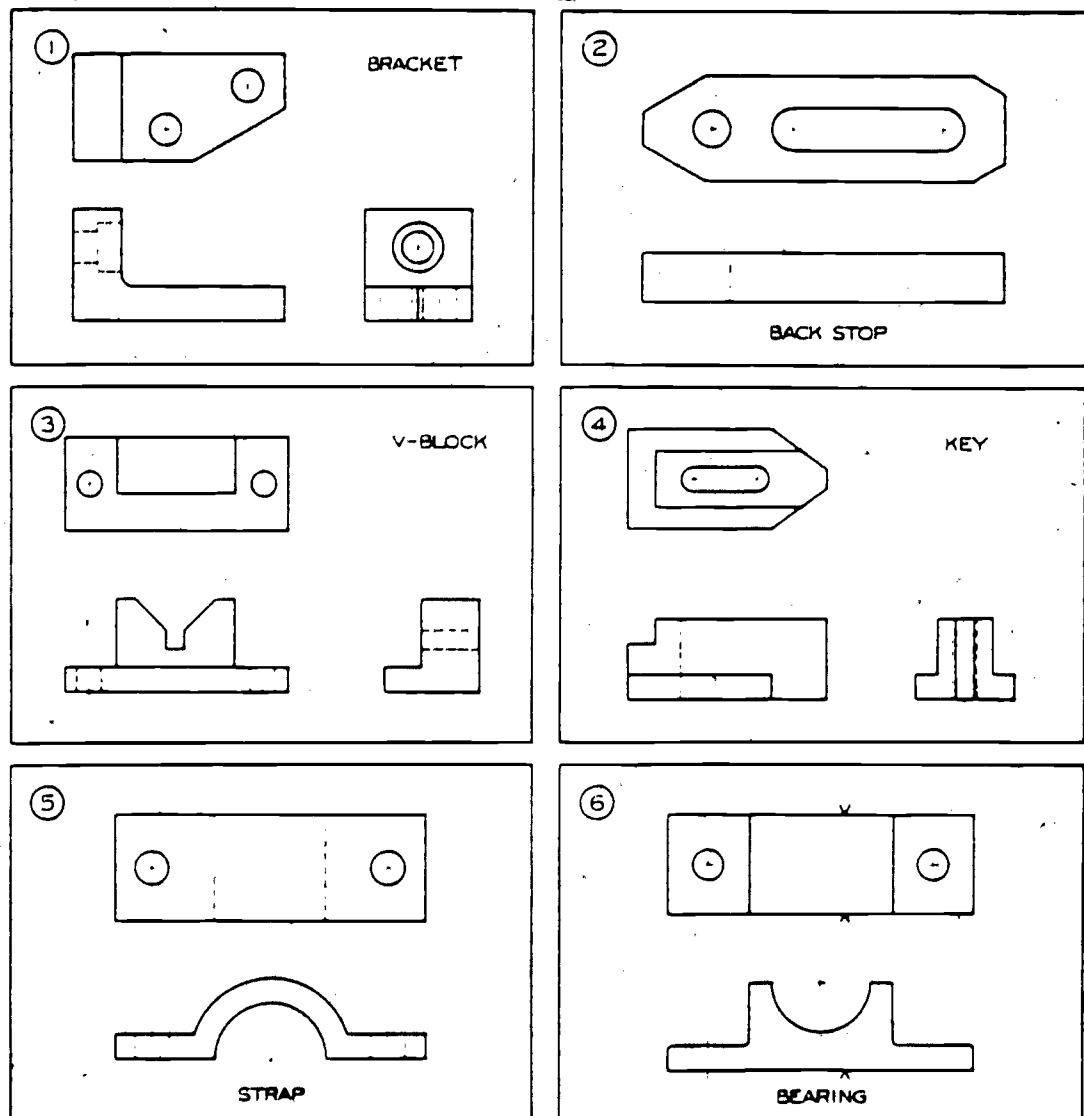
Fig. 9-40, p. 166, Dimensioning
