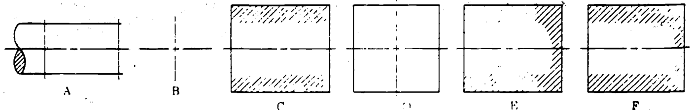
Fig. 10-48 Schematic representation of screw threads. Take dimensions from the printed scale at the bottom of the page, using dividers. Draw the views as shown and complete each as follows: A = schematic representation showing 1"-8UNC-2A threads; B = end view of A; C = schematic representation of
