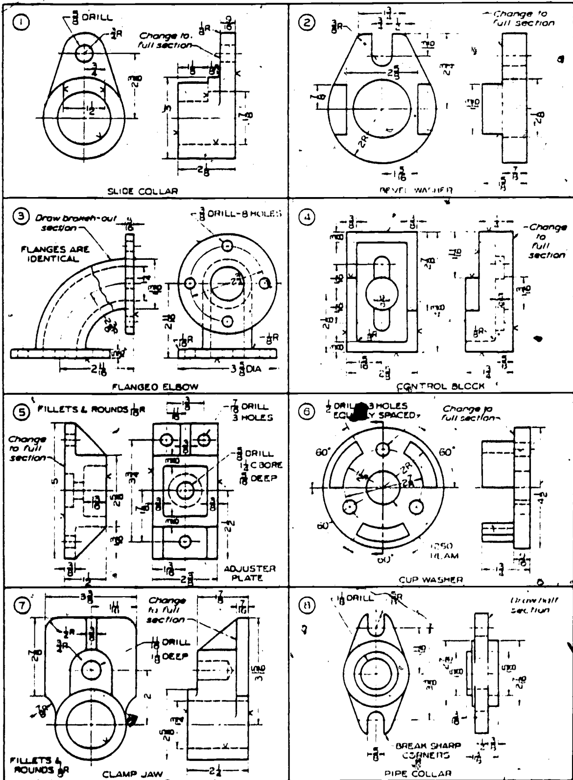
Fig. 11-25, Sectioning Problems. Page 205, Spencer. Make sketch or mechanical drawing. Section as indicated. Omit instructional notes. Give part names in title strips.
