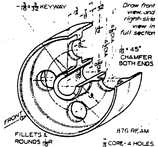
Pulley
