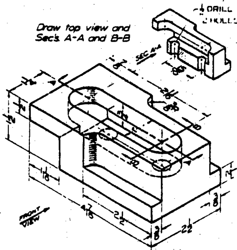
Guard Block
