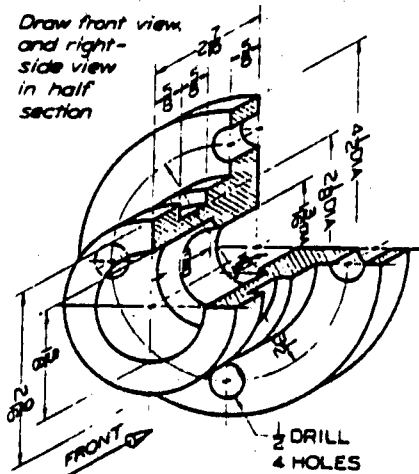
Stuffing Box
