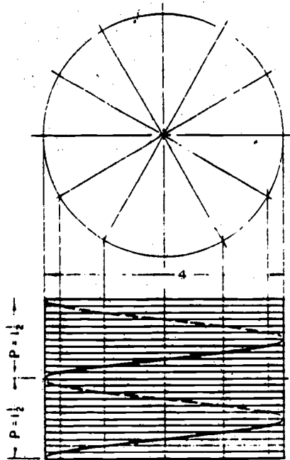
Fig. 10-44 Draw two complete turns of a right-hand helix as shown above. Use dimensions indicated and work full size. Number all points to avoid errors.
