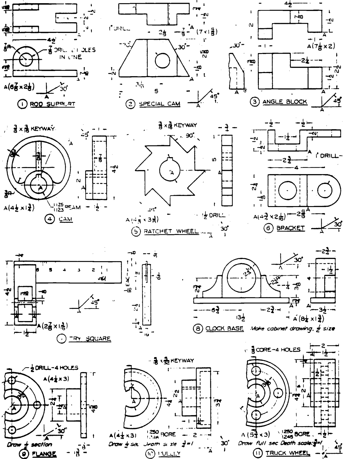
Fig. 16-53, p. 337, Basic Technical Drawing , Spencer. Oblique Problems. Locate starting corners A. Move titles to title strip and omit dimensions unless assigned.
