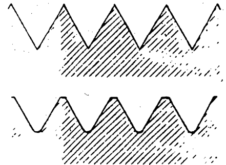
Fig. 10-46 Draw the profiles of the sharp "V" and the American National Unified thread. Letter the name of each under it. Pitch = 1".
