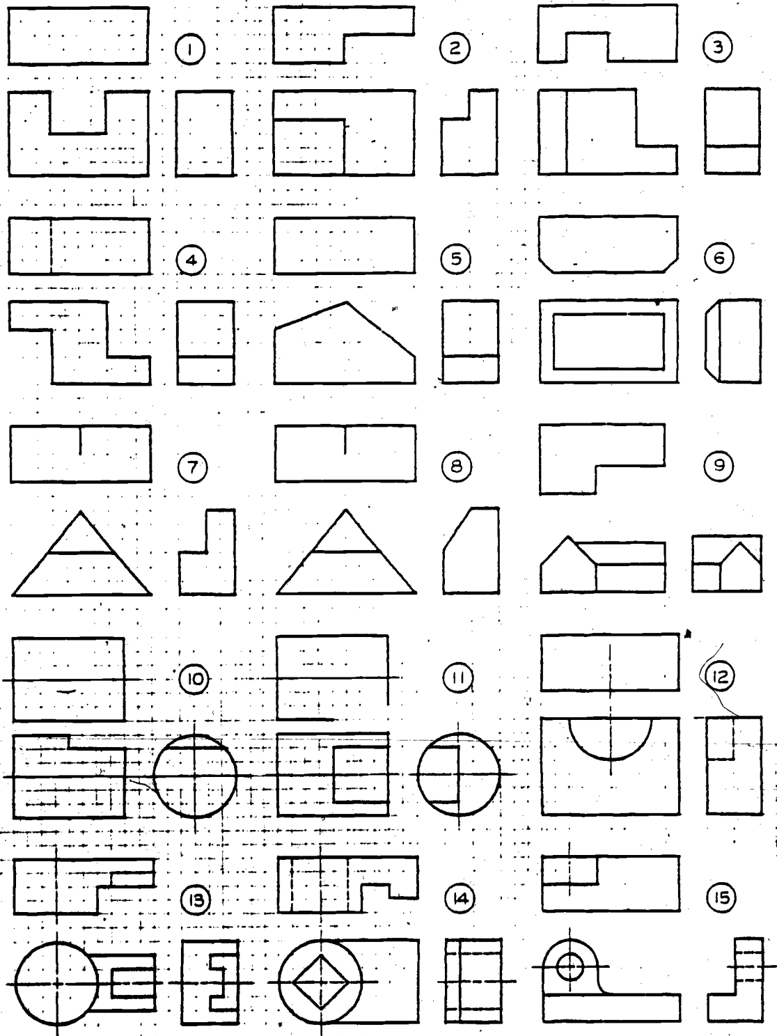
Fig. 6-29. Missing-Line Problems. Sketch the views of assigned problems, adding all missing lines. Each grid space = 1/4". In most cases, spacing between views can be improved by spacing views farther apart.
