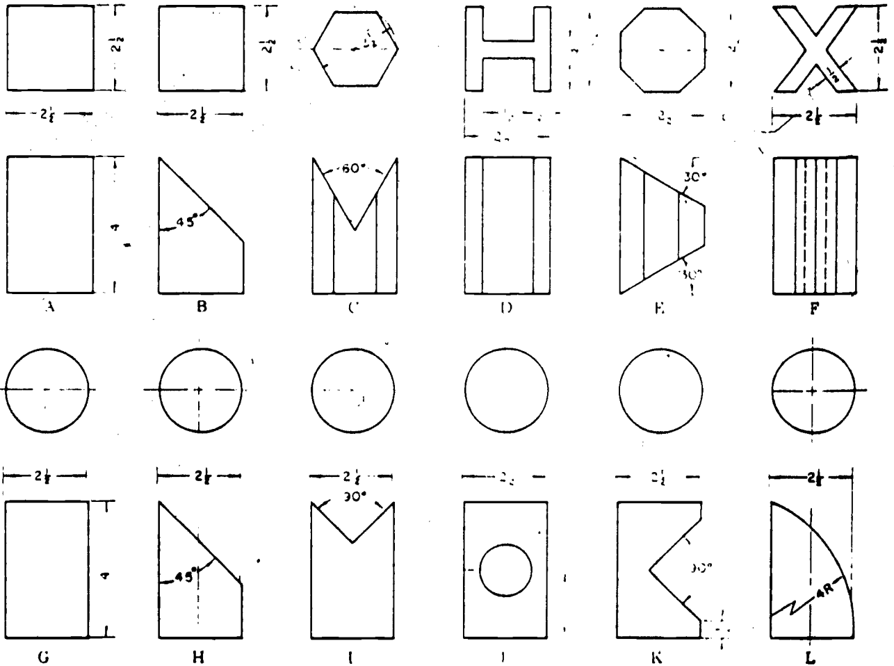
Fig. 18-53, p. 340, and 18-54, p. 341, Mechanical Drawing , French.
