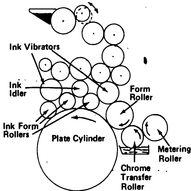
Integrated System Dahlgren Chrome Transfer Roller acts as Pan Roller
