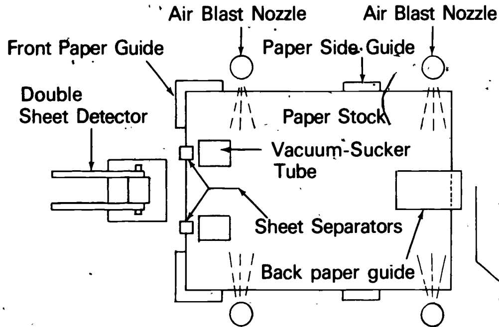
Top View of Feeding System
