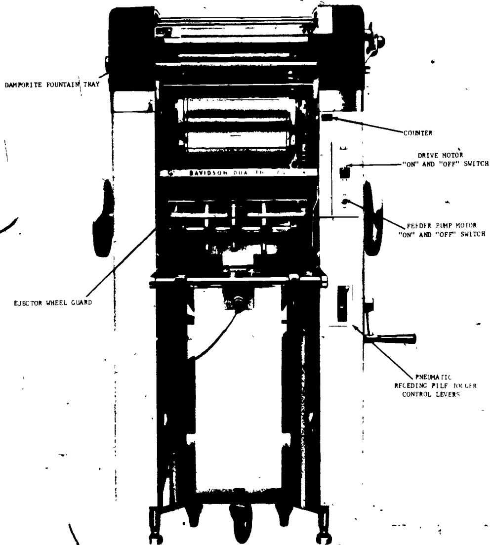
BACK OF MACHINE
