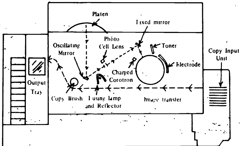
Schematic of a Typical Electrostatic Copier
