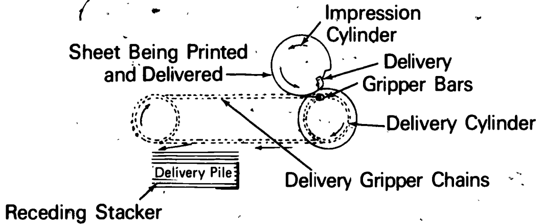
Chain Delivery With Receding Stacker
