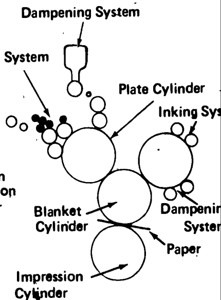
Two Color Common Blanket Cylinder
