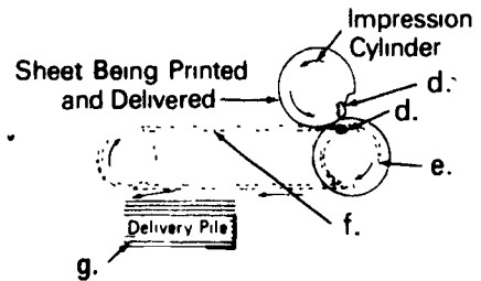
Chain Delivery With Receding Stacker
