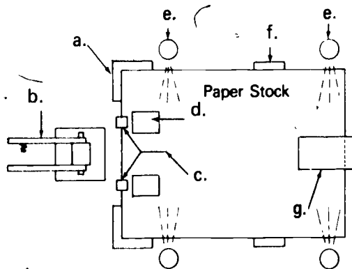
Top View of Feeding System
