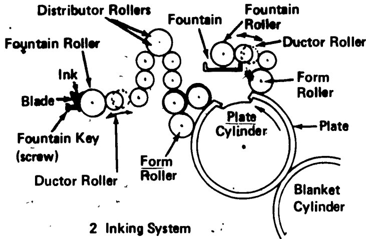
Conventional Inking and Dampening System
