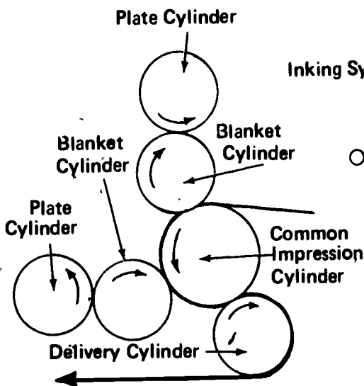
Two Color Common Impression Cylinder
