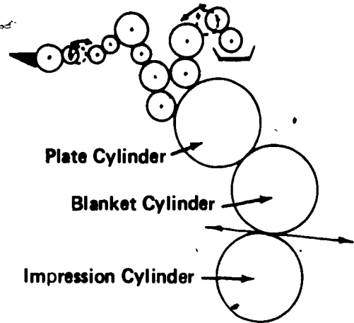
Integrated System A.B. Dick
