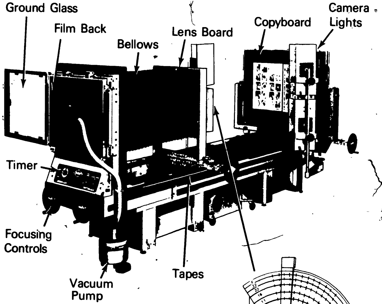
Horizontal Process Camera
