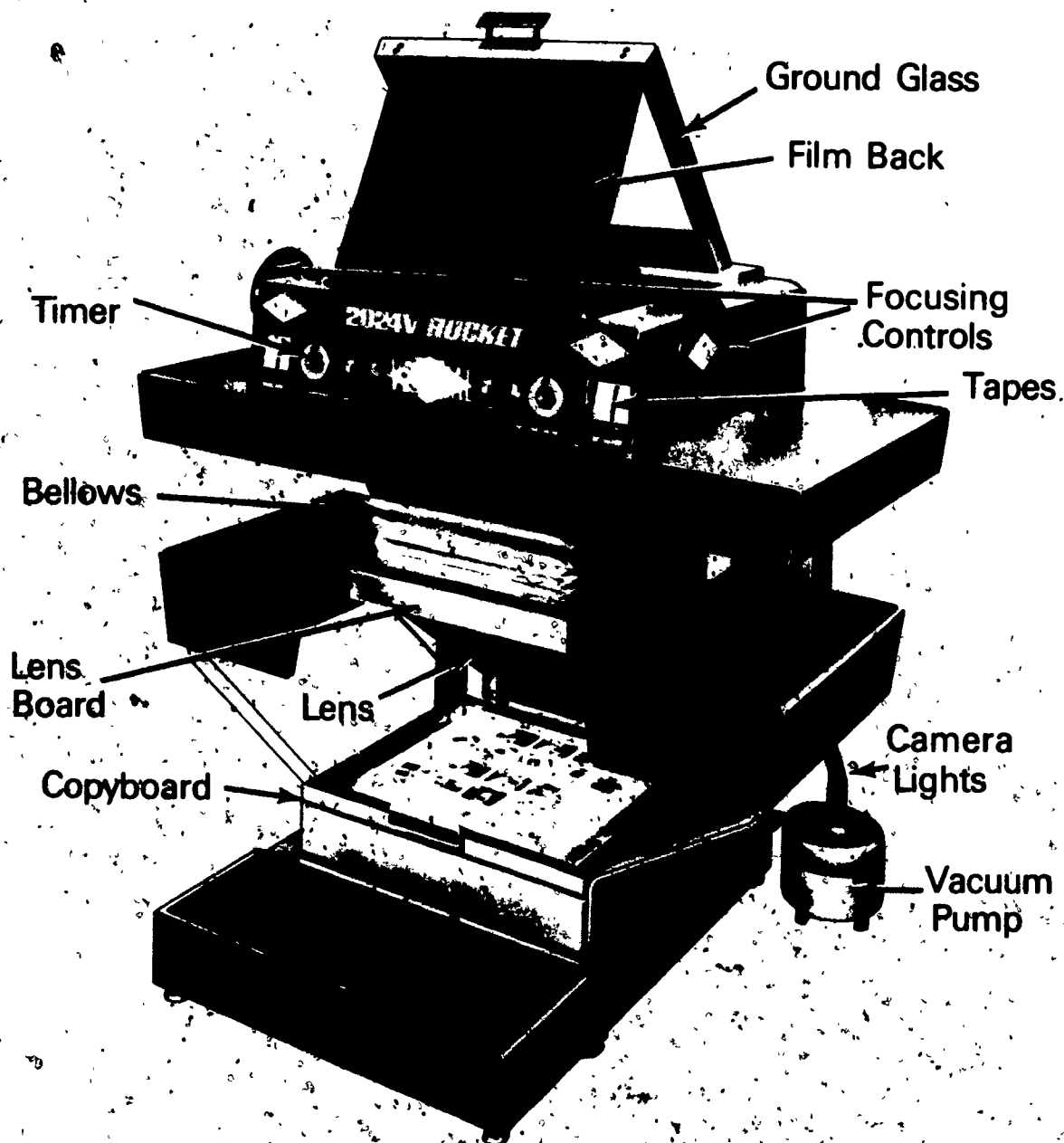
Vertical Process Camera
