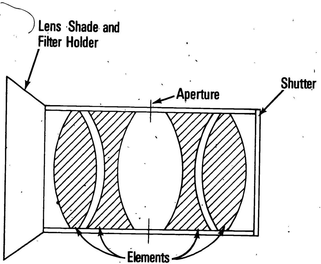
Schematic cross section of a typical process lens.
