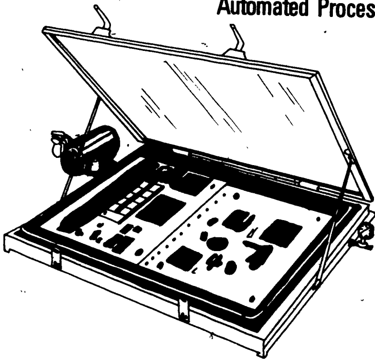
Vacuum Frame
