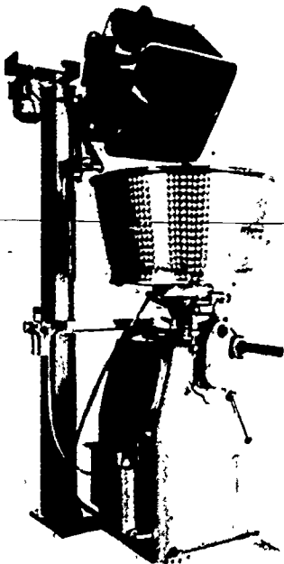
Fig. C-5. Stuffer
