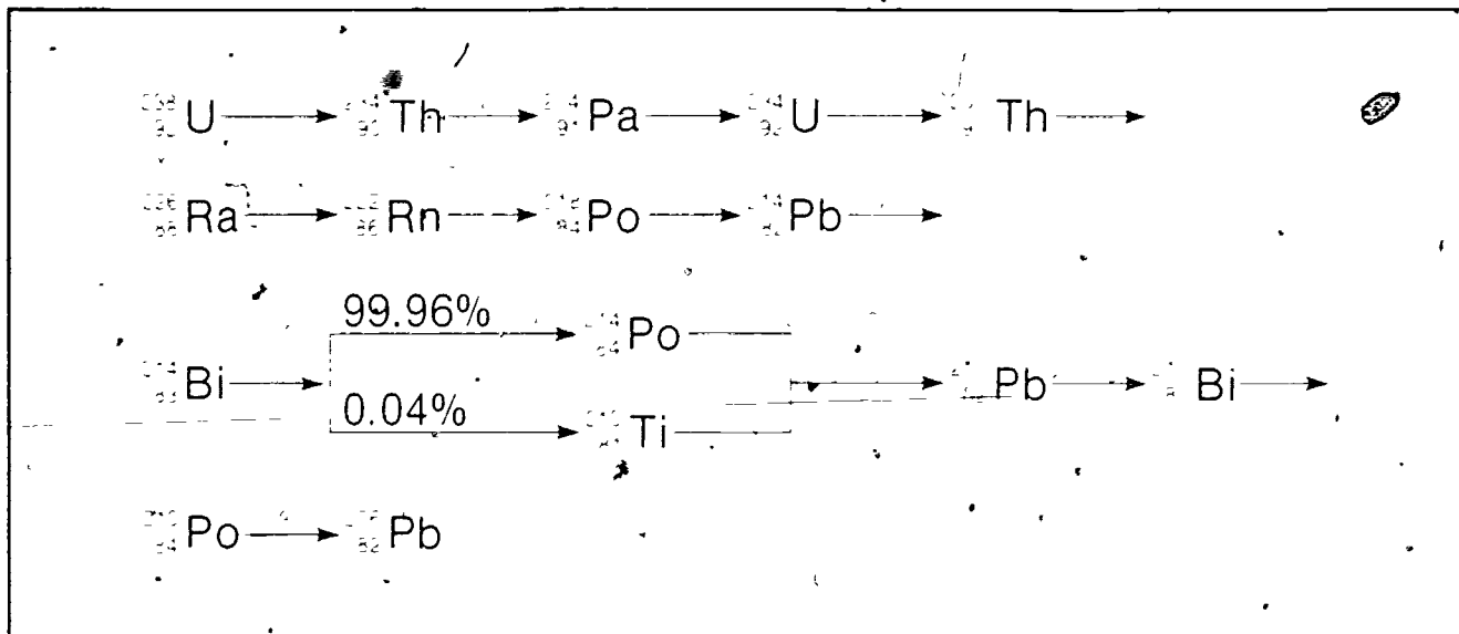
Figure A. Stages in the radioactive decay of Uranium-238.
