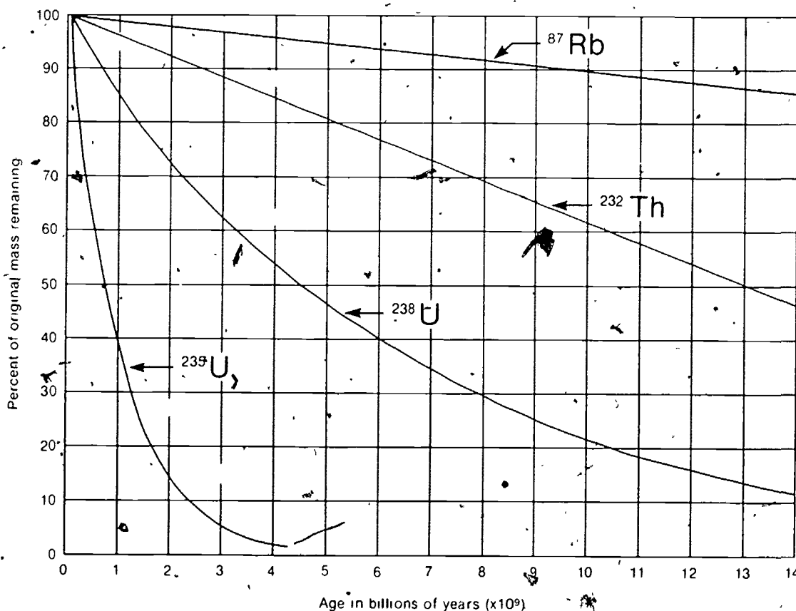
Figure 1. Graph of radioactive decay curve.
