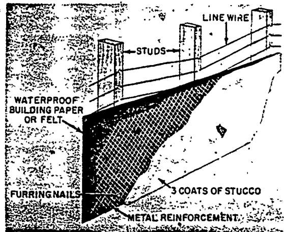
Figure 14-9.—Open frame construction. 133.156
