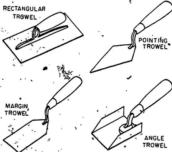
Figure 14-3.—Plastering trowels. 29.164
