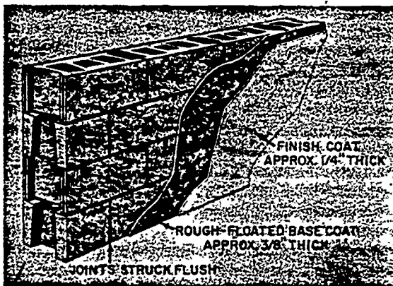
Figure 14-8—Masonry (2 coat work directly applied). 133.155
