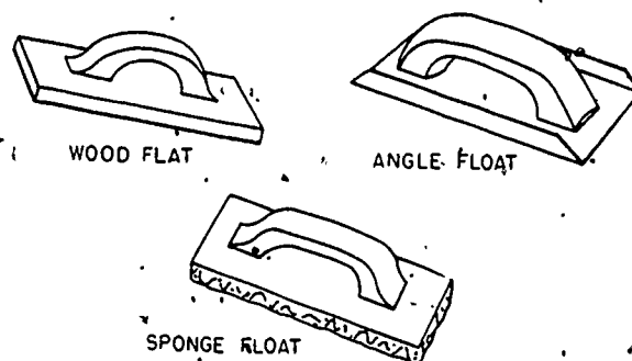
Figure 14-5.—Plastering floats. 29.161
