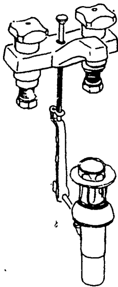
CENTERSET FITTING
