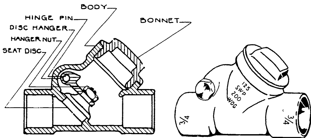
Check Valve
