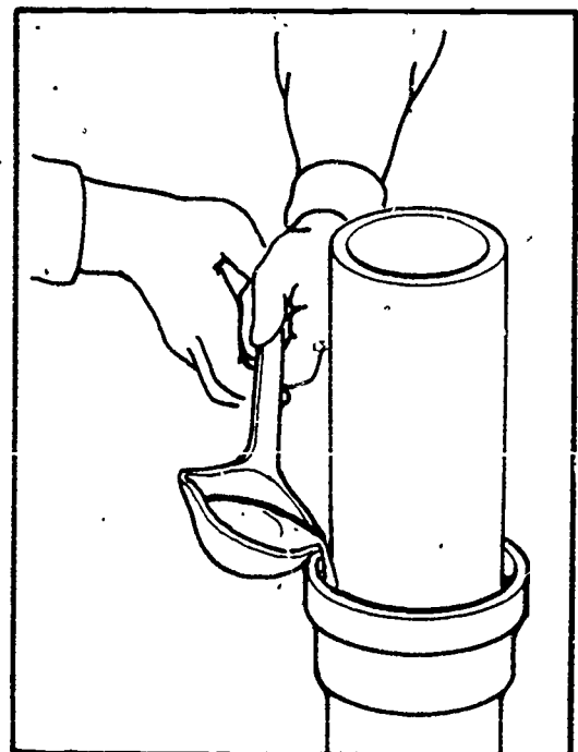
POURING MOLTEN LEAD
