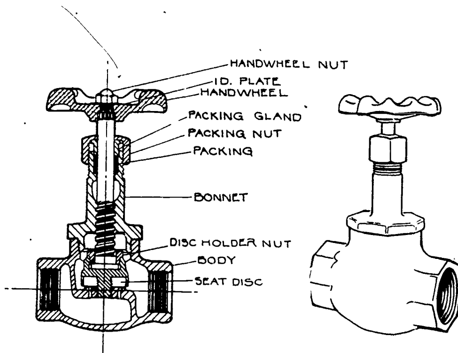
Bronze Globe Valve
