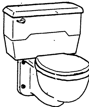
WALL-HUNG SIPHON JET WATER CLOSET WITH A CLOSE-COUPLED TANK AND BOWL
