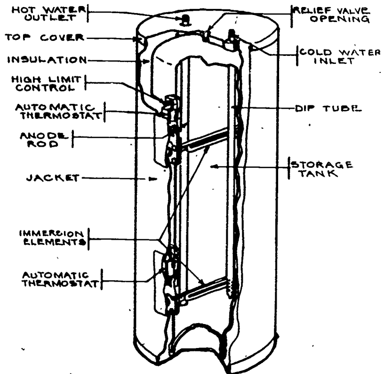
SECTIONAL VIEW OF AN AUTOMATIC ELECTRIC STORAGE TANK WATER HEATER
