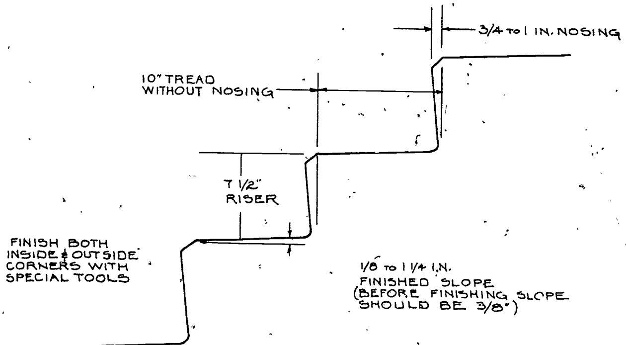
TYPICAL STEP DIMENSIONS FOR STAIRS 30" OR LESS HIGH
