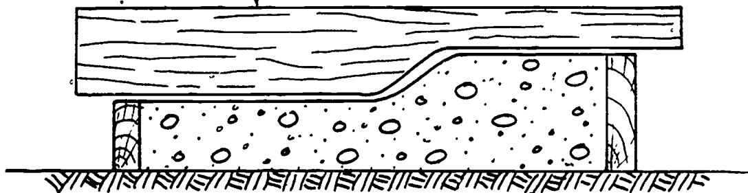
A WOOD TEMPLATE CAN BE USED FOR STRIKING-OFF A CURB
