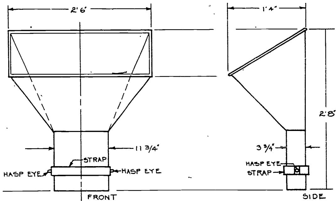
A RECTANGULAR DROP CHUTE WITH HOPPER AT TOP FOR PLACING CONCRETE IN NARROW WALLS
