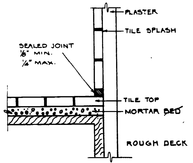
DECK AND SPLASH JOINT LINE
