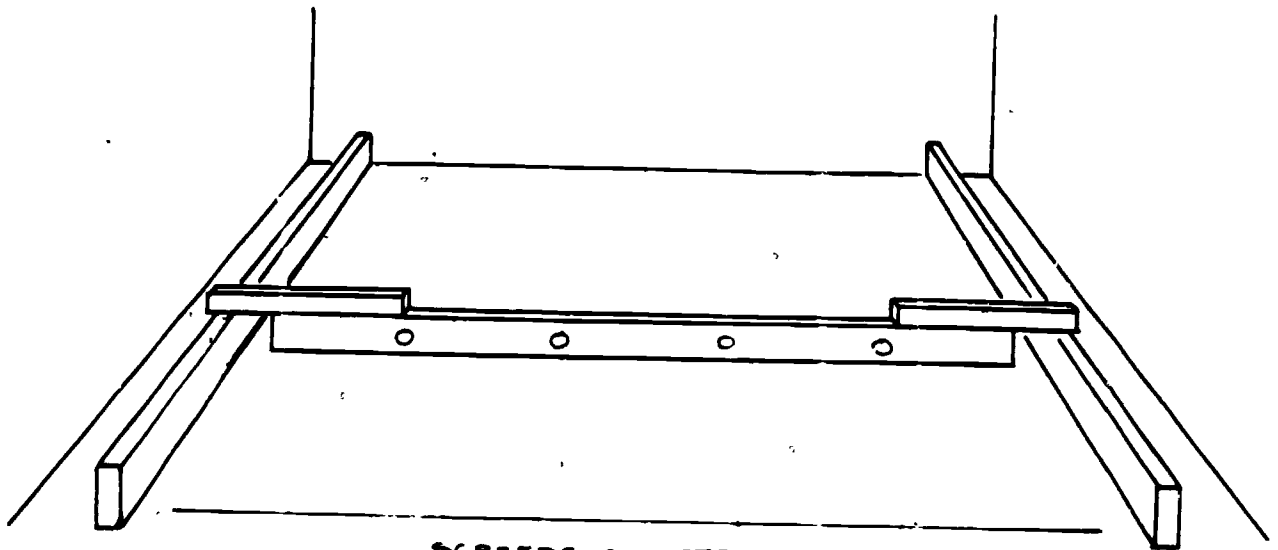
SCREEDS AND STRAIGHTEDGE IN PLACE FOR SCREEDING OFF
