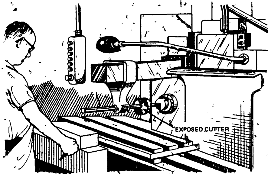
Figure 7. Horizontal milling machine without cutter enclosure.
