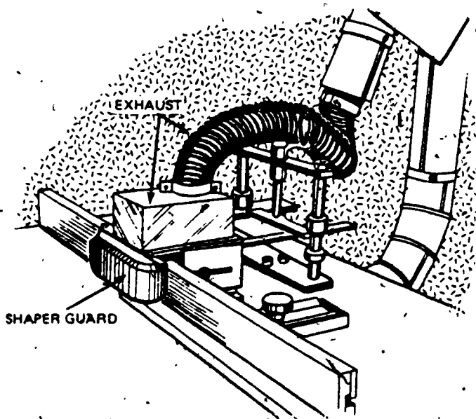
Figure 8. Shaper guard with attachment for chips to be exhausted through a flexible hose.
