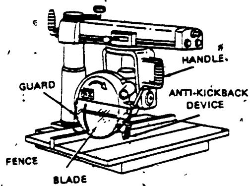
B. Radial arm saw.
