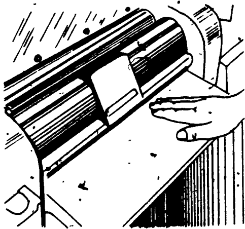
Figure 17. A single-surface planer. Note that there is no gap between the surface of the material being planed and the entrance to the cutterhead of the planer.
