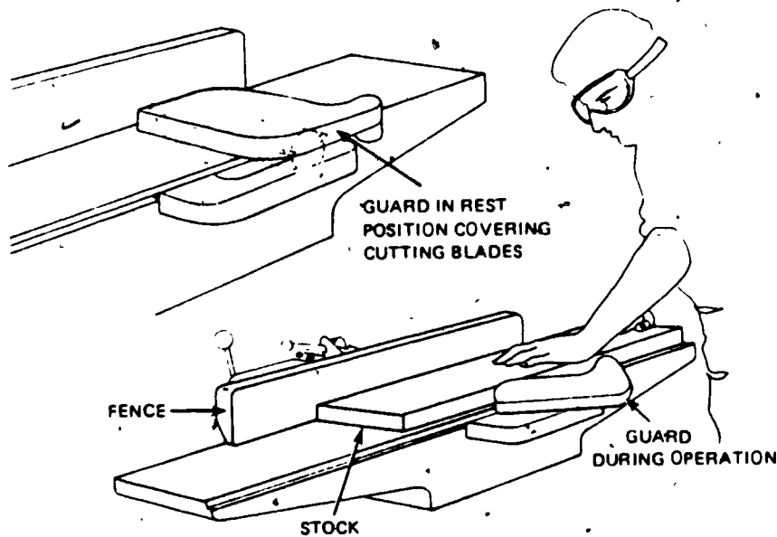
Figure 18, A jointer.
