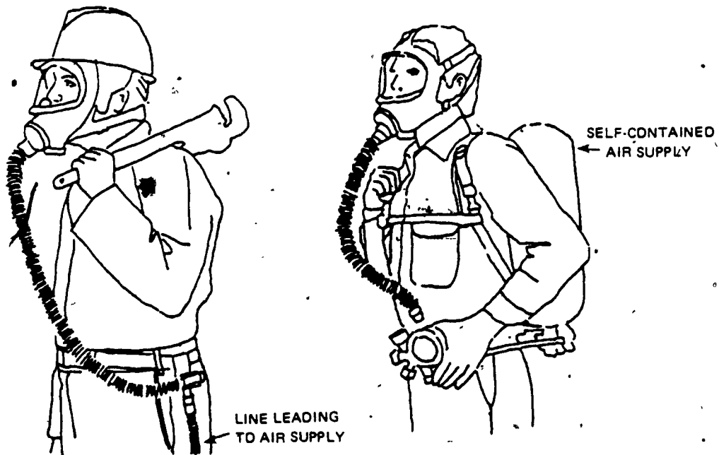
Figure 10. Supplied-air (airline) respirator (left) and self-contained air-supplying respirator (right).
