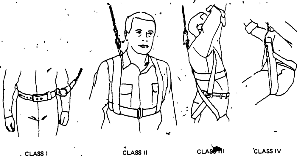
Figure 11. From left to right, body belt, chest harness, body harness, and suspension belt.
