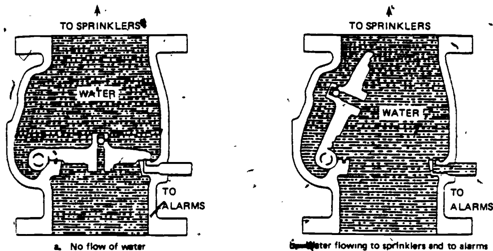
Figure 5. A wet-pipe sprinkler system.
