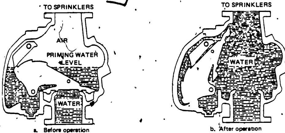
Figure 6. A dry-pipe system valve.
