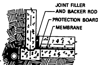
Foundation Wall
