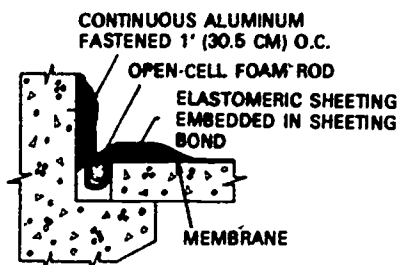
Expansion Joint at Wall
