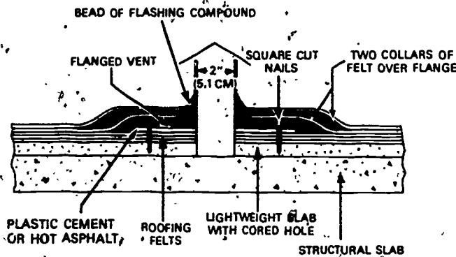
Fig. 5-1. A typical pressure release vent
