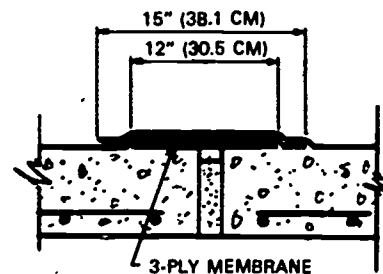
Expansion Joint
