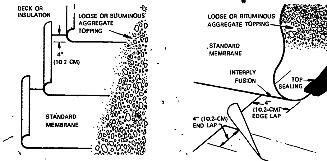
Fig. 4-5. Lapping the cold-applied bituminous membrane sheets (Koppers KMM)
