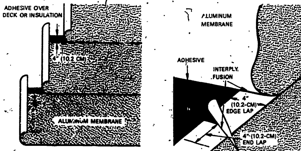
Fig. 4-7. Applying cold-process aluminum-grade bituminous sheet membrane (Koppers KMM)
