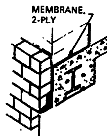
Spandrel Beam
