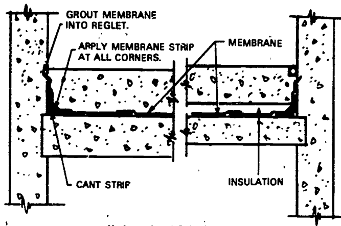
Horizontal and Split Slab
