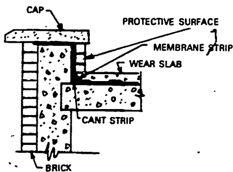
Split Slab Deck
