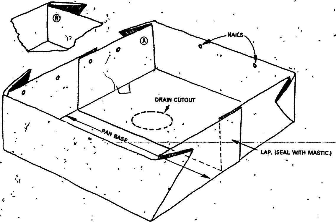
Fig.7-3. Construction of a shower pan (one ply shown)
