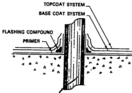
Flashing at a Small-Diameter Penetration
