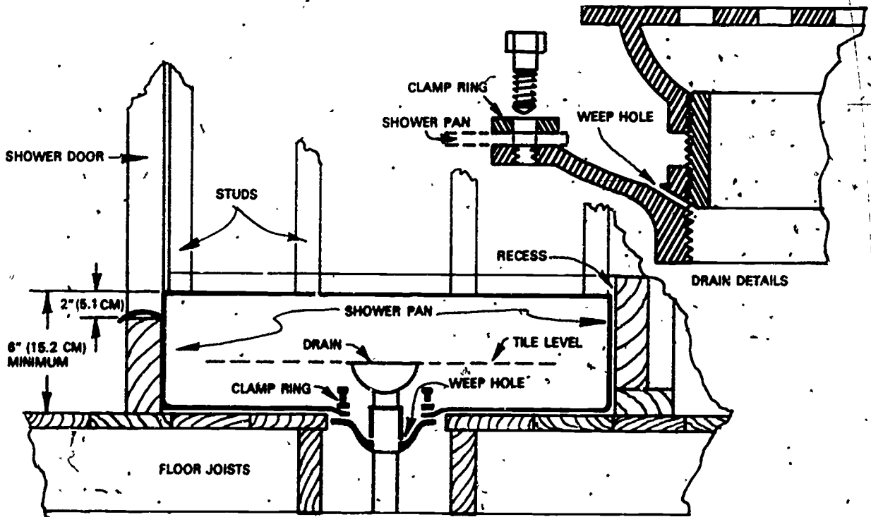
Fig.7-4. Installation of a shower pan and drain assembly
