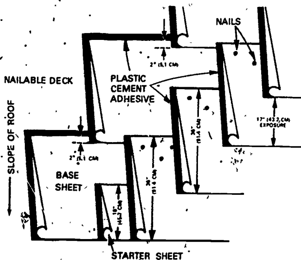
Fig. 3-2. One-ply base sheet with two-ply cold-applied roofing system
