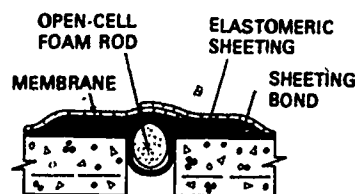
Deck Expansion Joint
