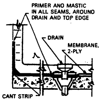
Planter-Shower Pan
