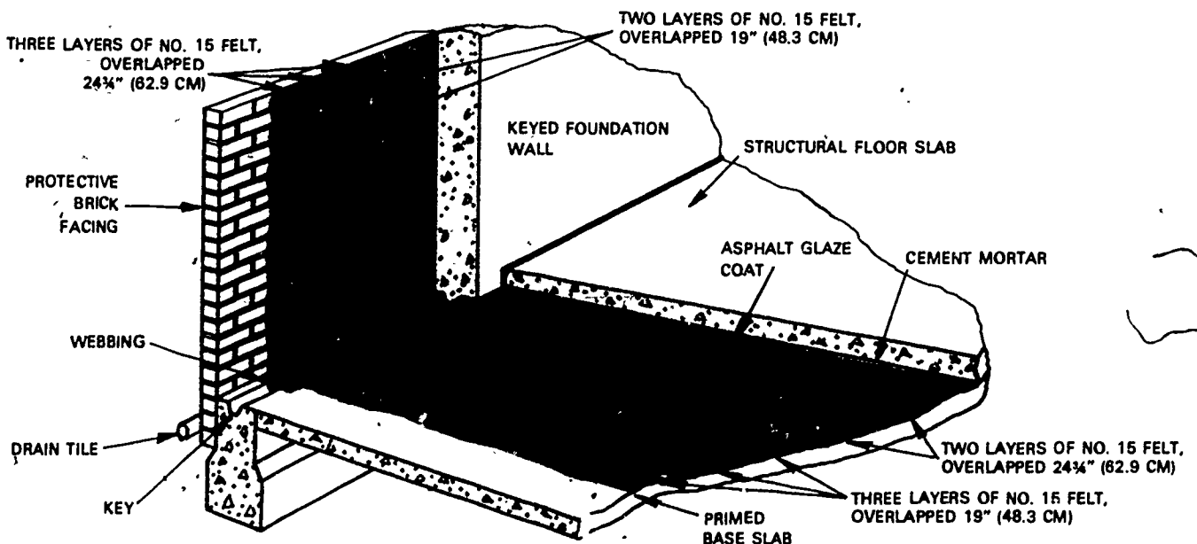
Fig.7-2. Inside method of waterproofing a foundation wall
