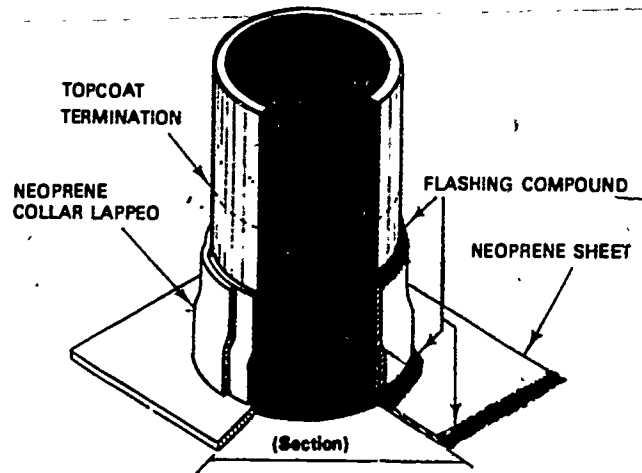
Flashing at a Large-Diameter Penetration
