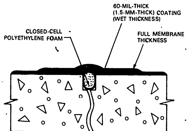
Fig. 8-3. Sealing a working crack (Tremco's TREMproof 50)
