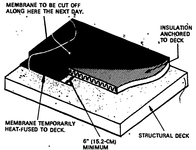
Fig. 4-3. A standard water stop
