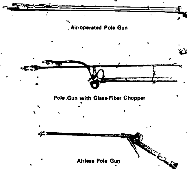
Fig.2-5. Spray guns for applying cold-process fluids
