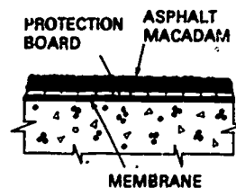
Vehicular Deck
