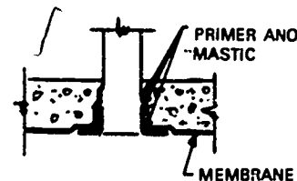
Drain and Post
