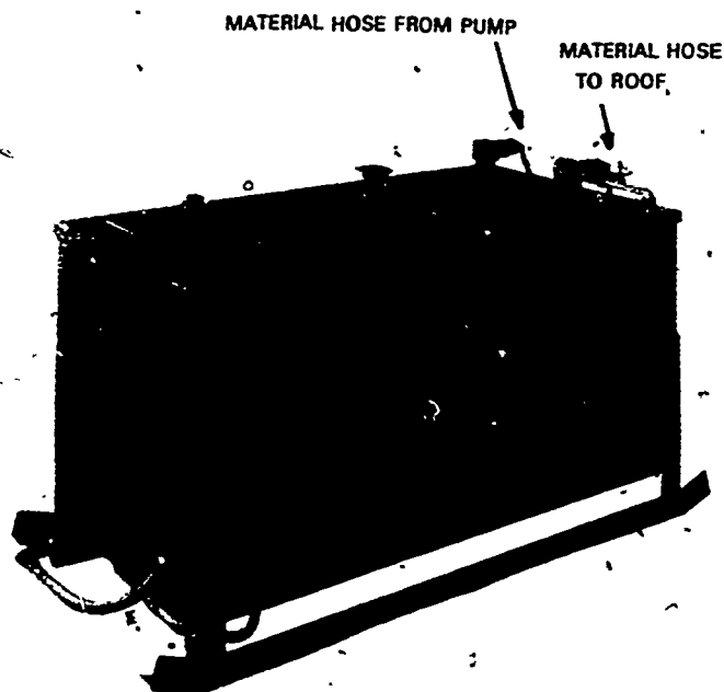
Fig. 2-3. An in-line warming kettle for cold-applied materials
