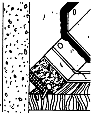
Fig. 3-1. Cant strip detail
