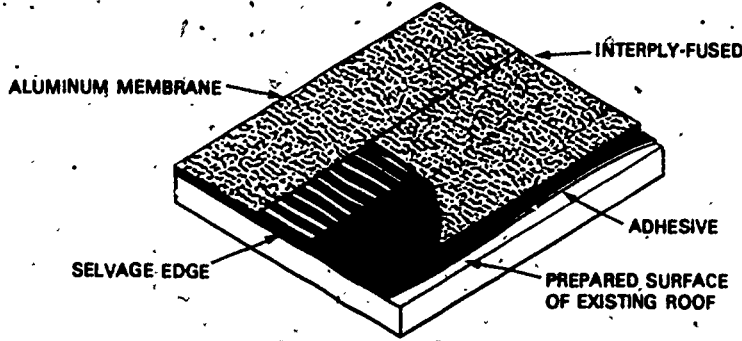
Fig. 4-8. Methods of reroofing with cold-applied bituminous sheet membranes (Koppers KMM)
