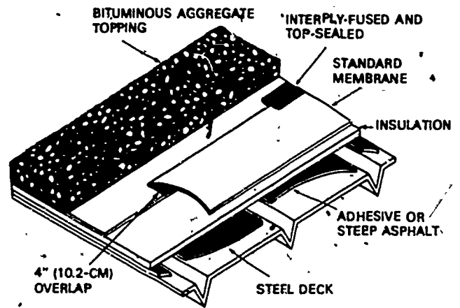
Fig. 4-2. Standard-grade cold-applied bituminous sheet membrane on a metal deck ( Koppers KMM )
