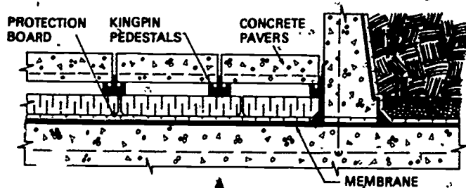
Insulated Plaza Deck Section with Planter
