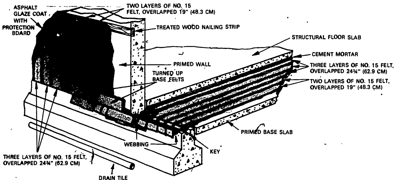
Fig.7-1. Waterproofing a concrete floor slab and foundation wall
