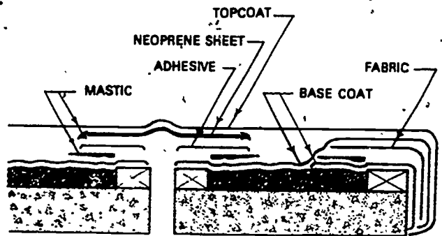
Flashing at Expansion Joint and Deck Edge
