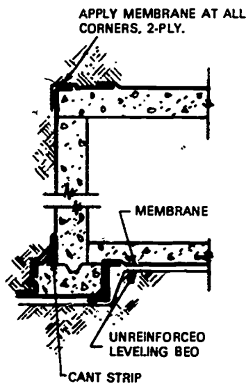
Slab on Grade
