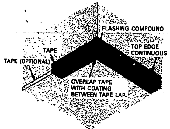
Flashing at a Vertical Section (outside corner)
