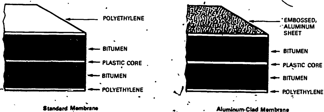
Fig. 4-1. Cold-applied standard-grade and aluminum-grade bituminous sheet membranes (Koppers KMM)
