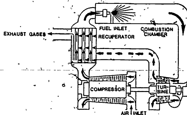
Figure 26. Schematic of Gas Turbine with Recuperative Exhaust System.
