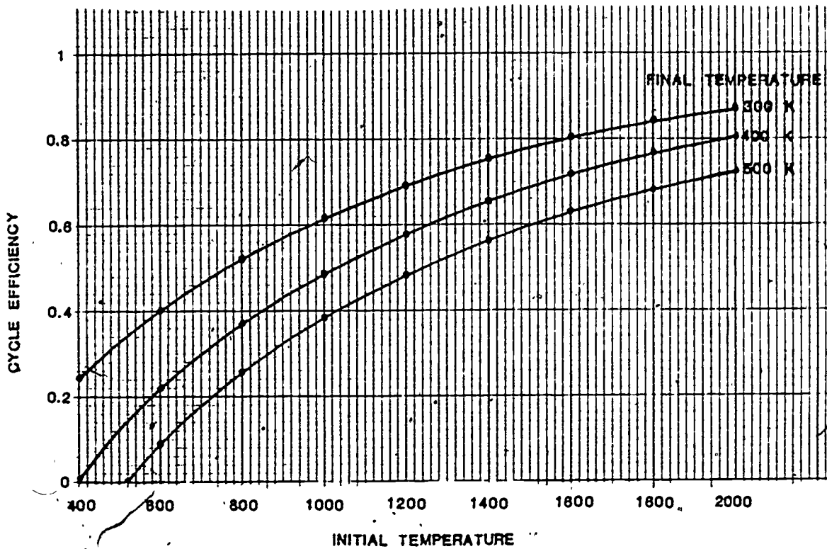
Figure 9. Maximum Cycle Efficiency Vs. Initial Temperature for Several Different Values of Final Temperature.
