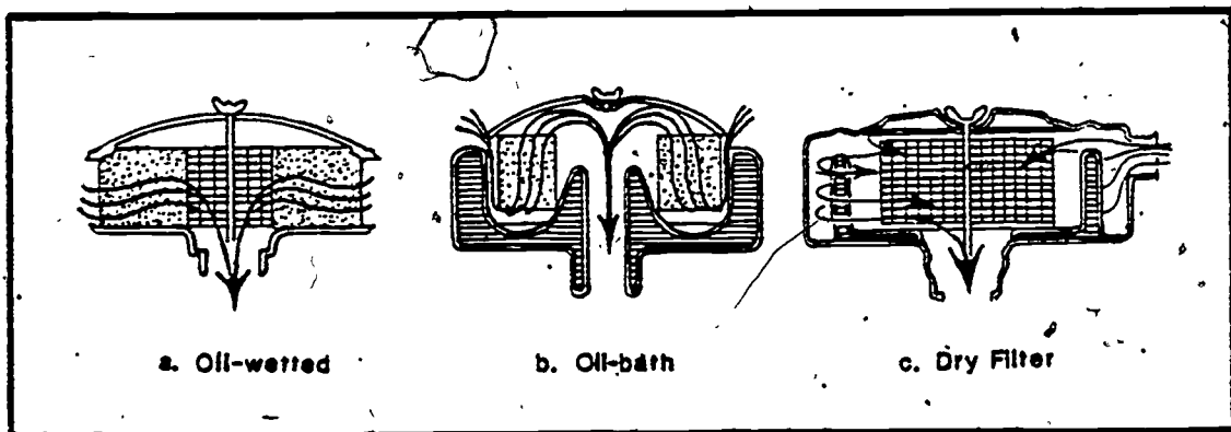
Figure 29. Three Types of Air Cleaners.
