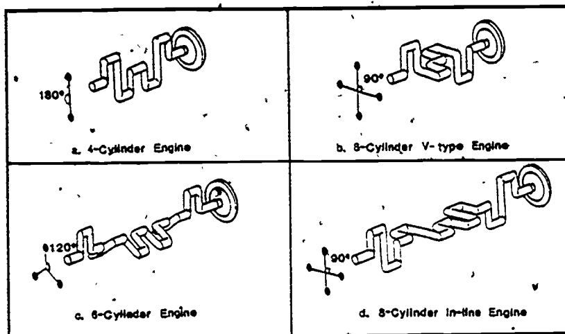
Figure 18. Crankshaft Configurations for Various Types of Engines.
