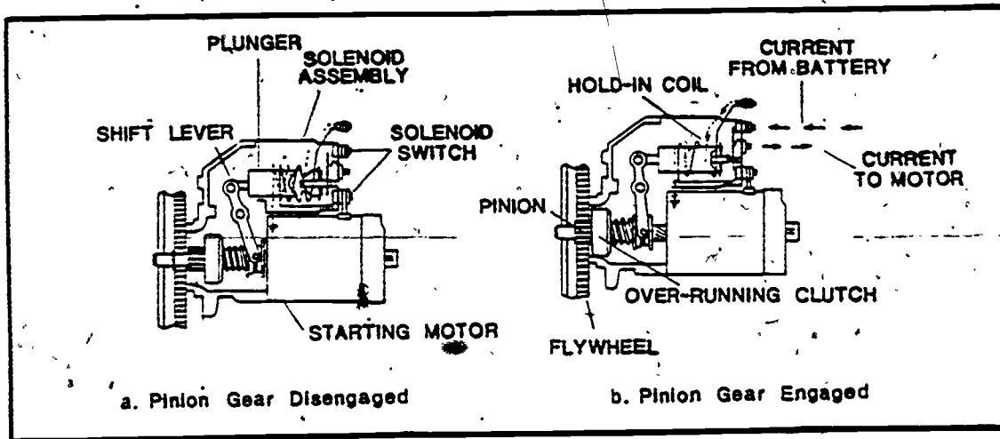
Figure 37. Operation of the Solenoid.
