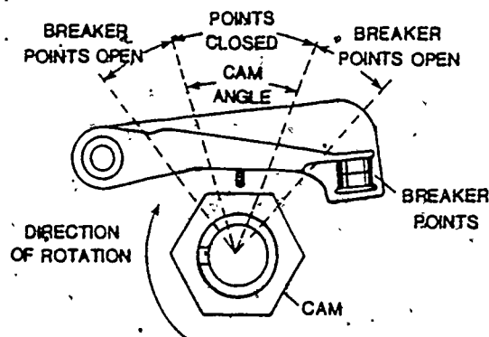
Figure 34. Distributor Cam and Breaker Points.
