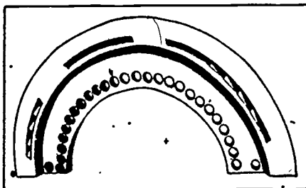
Figure 12. Typical Nozzle Block with Three Groups of Converging Nozzles.
