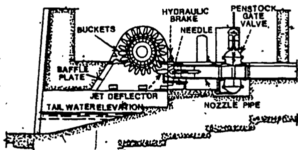
Figure 27. Impulse-Type Hydraulic Turbine.
