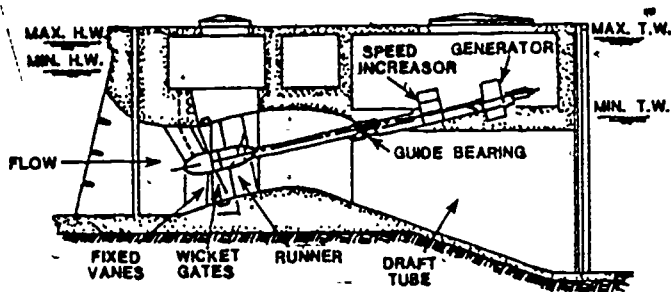
Figure 29. Axial-Flow Propeller Turbine.
