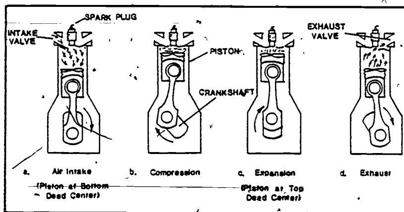
Figure 6. Four-Stroke Cycle: One Power Stroke Out of Two Revolutions.
