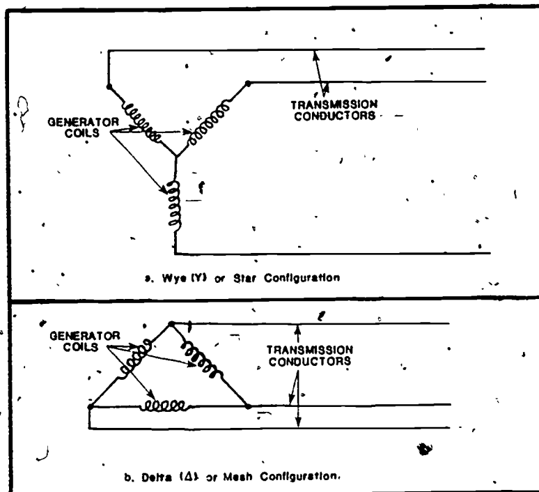
Figure 6. Connections for Three-Phase Alternating Current.
