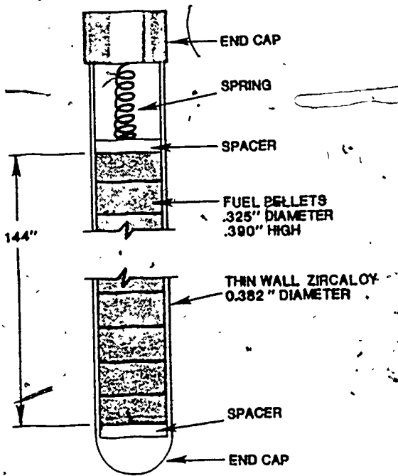
Figure 1. Schematic Diagram of a Typical Fuel Rod Structure.
