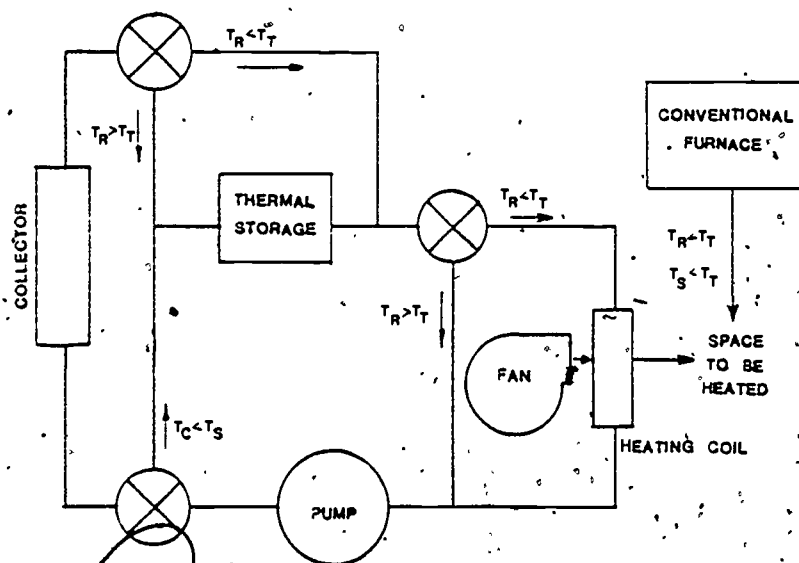
Figure 15. Control Circuit.
