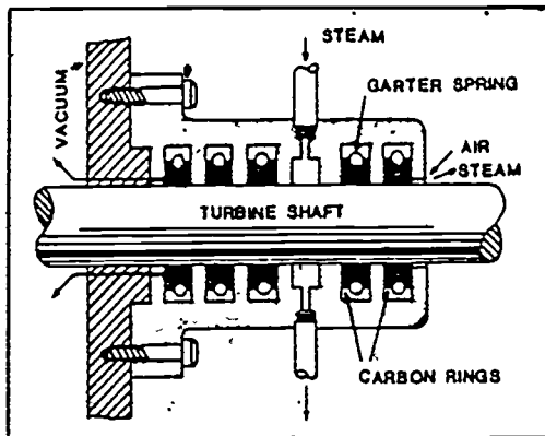
Figure 16. Carbon Rings
