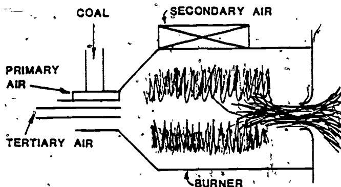
Figure 4. Diagram of Cyclone Furnace.
