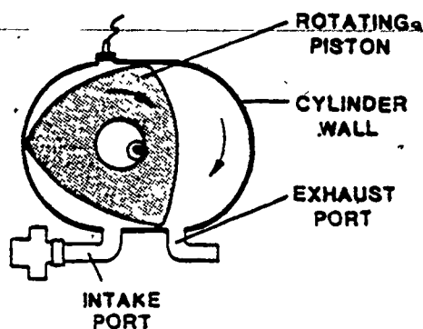
Figure 4. Rotary Engine.
