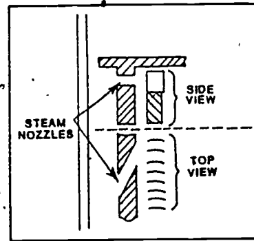
Figure 3. Top and Side Views of Single-Stage Impulse Turbine.
