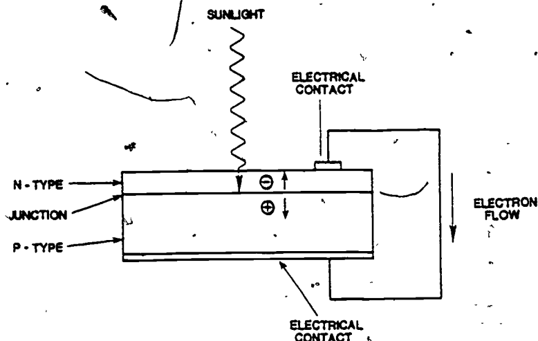
Figure 15. Diagram of Photovoltaic Cell.
