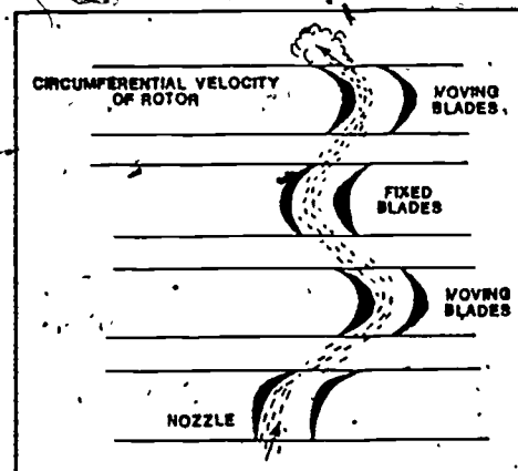
Figure 5. Double-Row Curtis Turbine (Velocity Staging).
