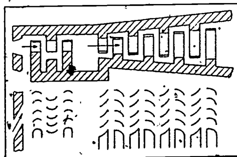
Figure 10. Combination Impulse-Reaction Turbine.
