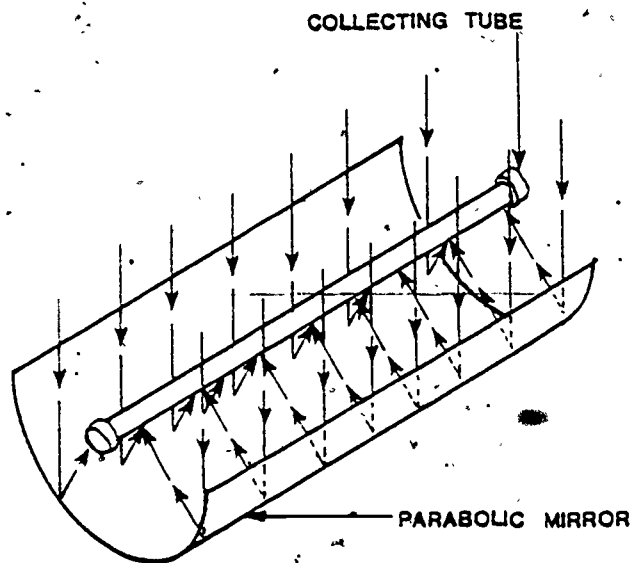
Figure 11. Example of Focusing Collector.
