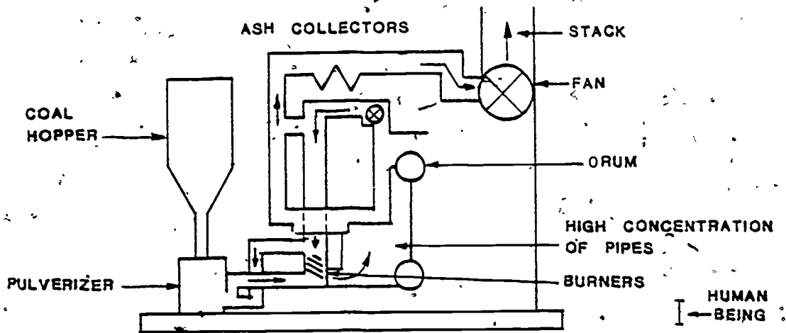
Figure 9. Steam-Generating Facility Powered by Pulverized Coal.
