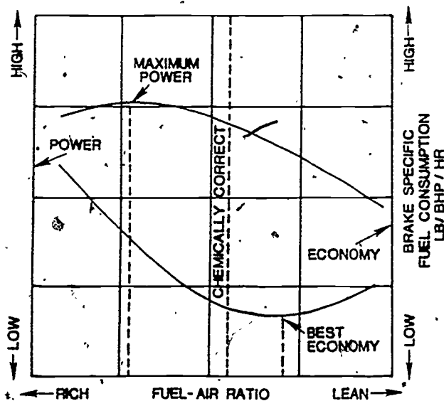
Figure 32. Economy Vs. Power in Internal Combustion Engines.
