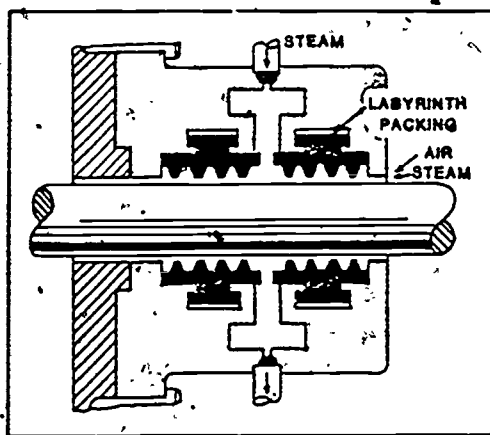
Figure 17. Labyrinth Gland.
