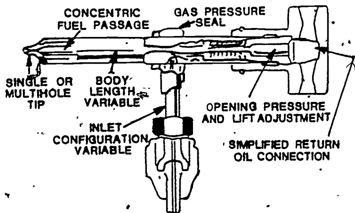
Figure 27. Single-or Multiple-Hole Nozzles.
