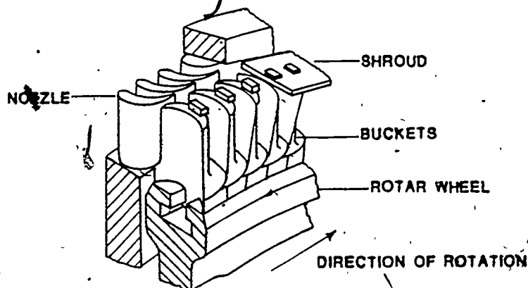
Figure 14. Parts of a Rotor.
