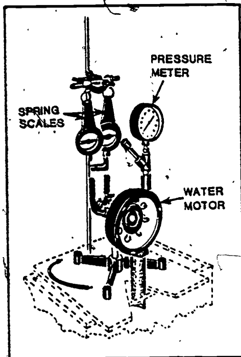
Laboratory Setup.
