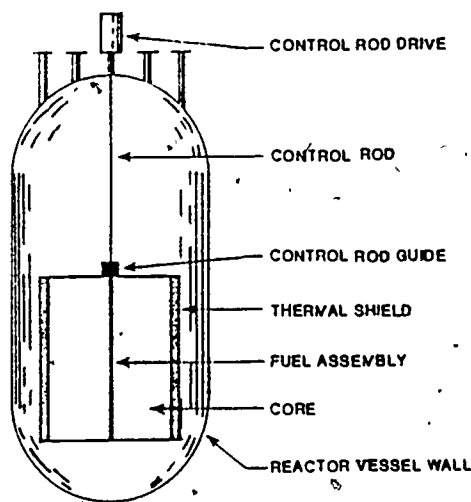
Figure 3. Schematic Diagram of Reactor Vessel.
