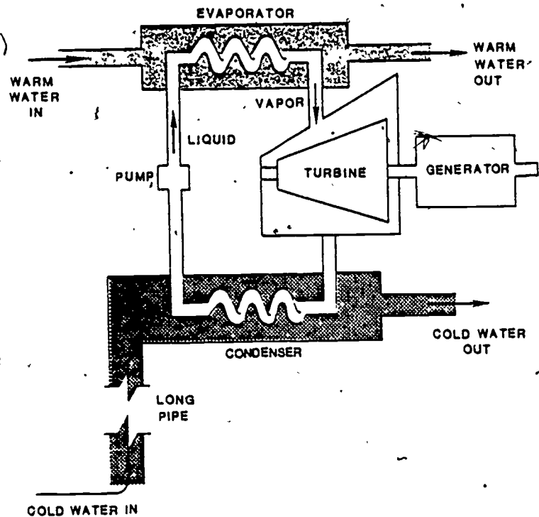
Figure 15. Diagram of Ocean Thermal Energy Conversion.
