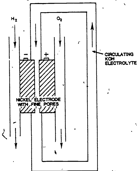
Figure 12. Diagram of Bacon-Type Fuel Cell.
