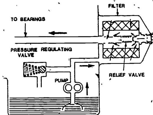
Figure 22. Full-Flow Oil Filter.
