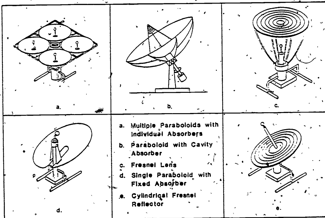
Figure 12. Examples of Concentrating Collectors.
