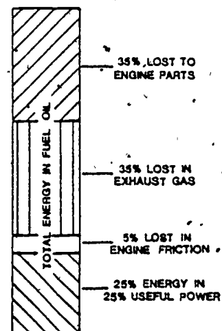
Figure 7. Energy Utilization in an Engine.
