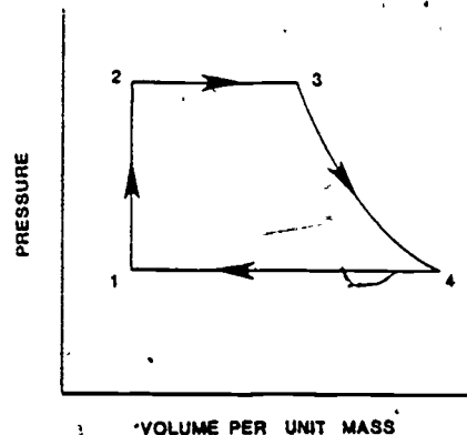
Figure 2. The Rankine Cycle.
