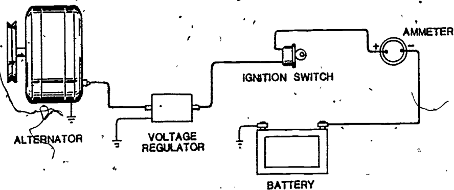
Figure 38. Schematic of a Charging System.
