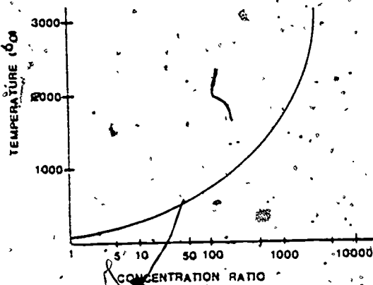
Figure 13. Fluid Temperature Vs. Concentration Ratio for Concentrating Collectors, for Insolation of 1000 \text{ W/m}^2 .
