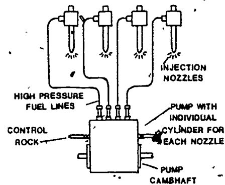
Figure 24. Pump-Injection Fuel System.
