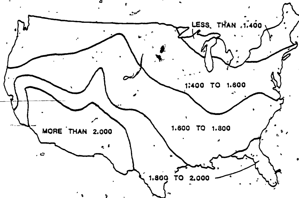
Figure 7. Annual Insolation in the U.S. (Numbers indicate kWh/m 2 .)
