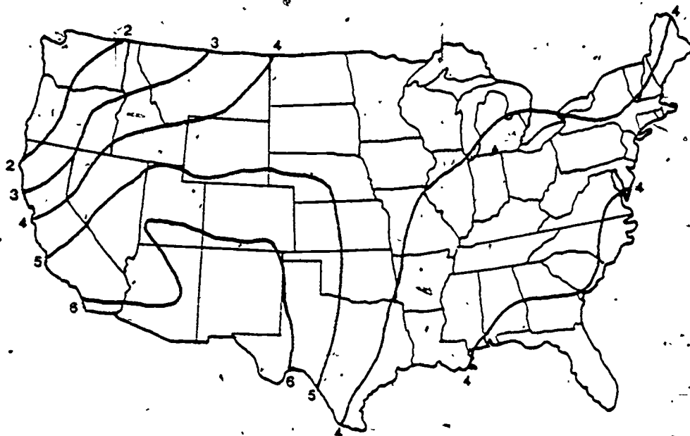
Figure 6. Contours of Total Daily Solar Energy Striking a Surface Directly Facing the Sun in Winter. (Units are in kWh/m 2 .)
