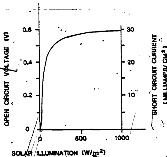
Figure 17. Output of Typical Silicon Photovoltaic Cell Vs. Incident Solar Illumination.
