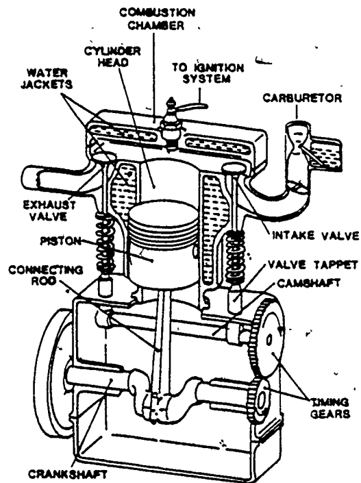
Figure 3. Schematic of a Reciprocating Engine.
