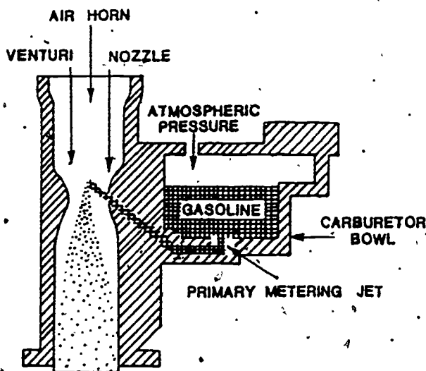
Figure 31. Simplified Carburetor.
