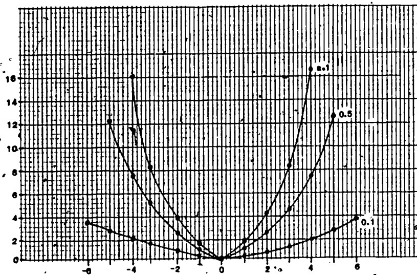
Figure 19. Examples of Parabolas.
