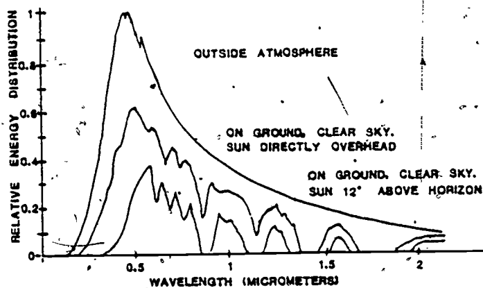
Figure 2. Wavelength Distribution of Solar Energy.
