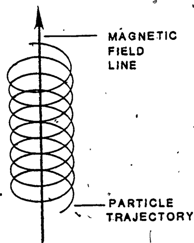
Figure 11. Trajectory of Charged Particle in a Magnetic Field.
