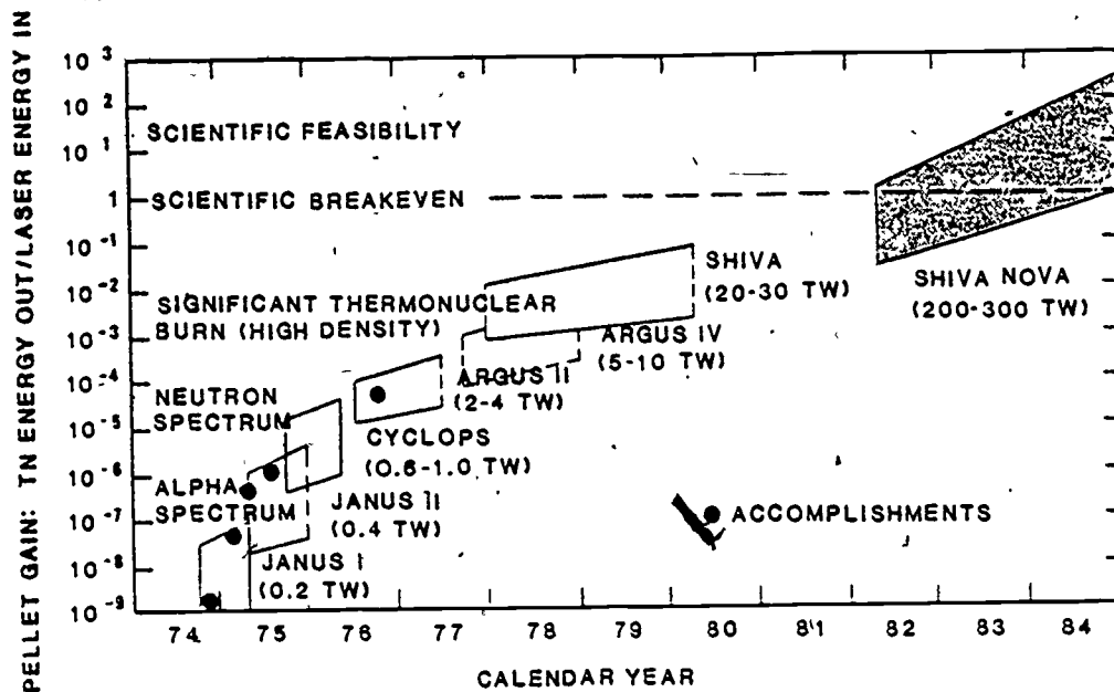
Figure 14. Laser Fusion Energy Yield Projections.
