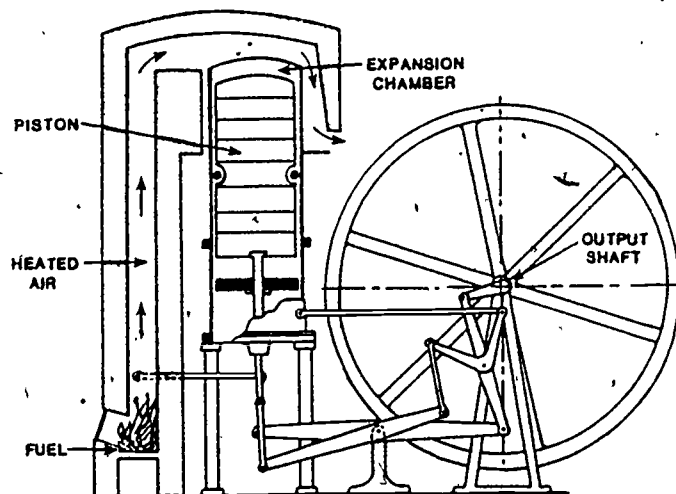
Figure 1. Early Stirling Engine.
