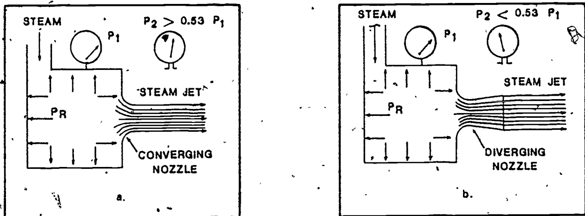
Figure 11. Two Types of Nozzles Used in Steam Turbines.
