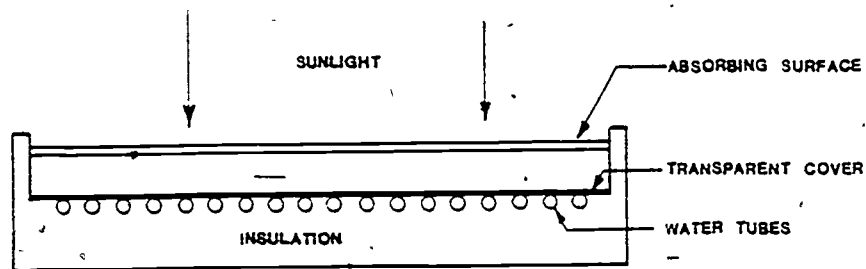
Figure 10. Schematic Diagram of a Basic Flat-Plate Collector.
