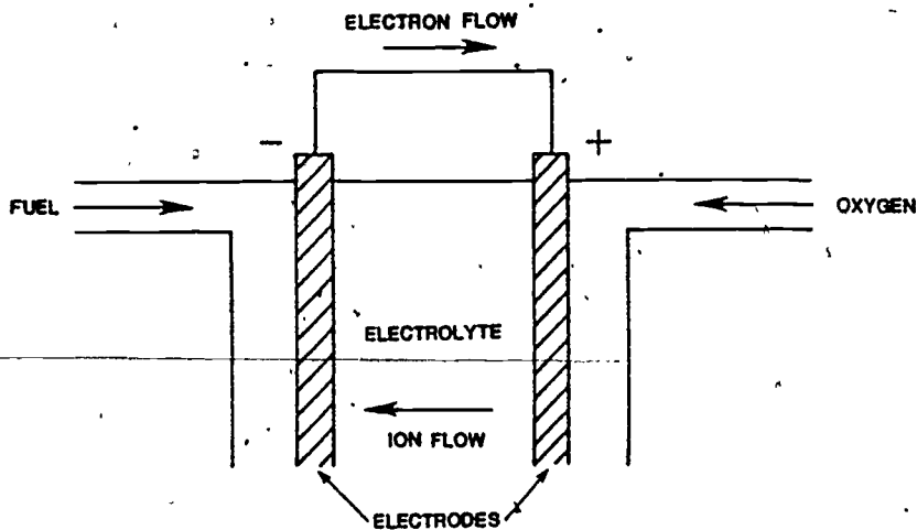
Figure 11. Schematic Diagram of Fuel Cell.
