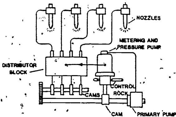
Figure 25. Distributor Fuel Injection System.
