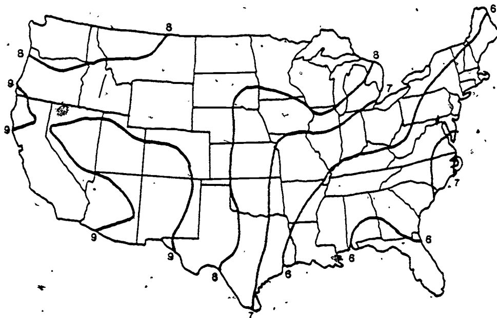
Figure 5. Contours of Total Daily Solar Energy Striking a Surface Directly Facing the Sun in Summer. (Units are in kWh/m 2 .)
