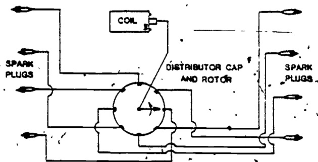
Figure 35. Schematic of High Voltage Ignition Circuit.
