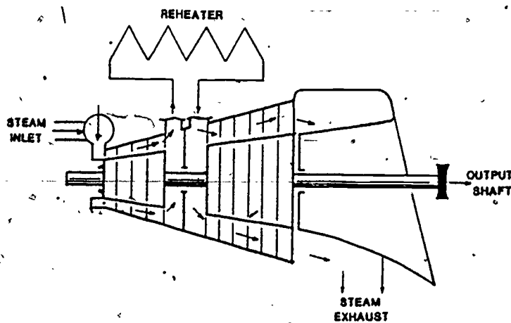
Figure 21. Single-Reheat Turbine.
