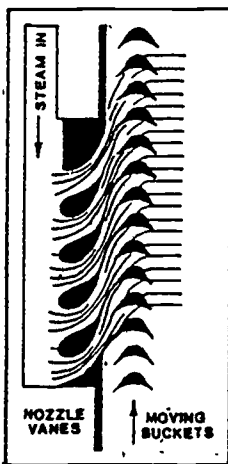
Figure 2. Schematic of Impulse Stage Blading.
