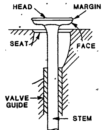
Figure 15. Valve.
