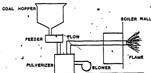
Figure 2. Schematic Diagram of a Direct-Firing System for Pulverized Coal.
