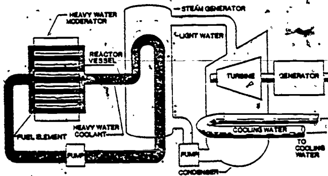
Figure 7. Diagram of a Heavy Water Reactor.
