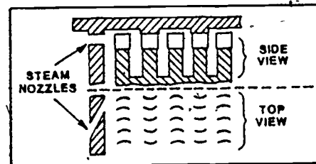
Figure 4. Top and Side Views of Velocity-Stage Impulse Turbine.
