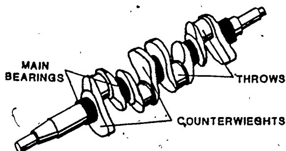
Figure 17. Crankshaft.
