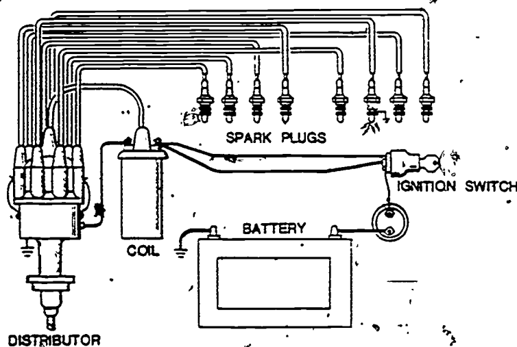
Figure 33. Schematic of a Typical Ignition System.
