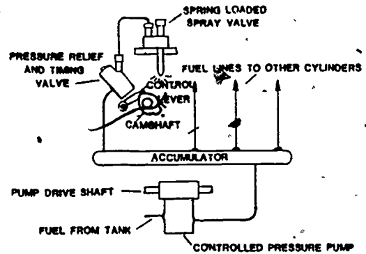
Figure 23. Common-Rail Fuel Injection System.
