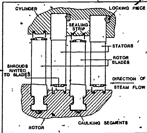
Figure 15. Positioning and Mounting of Stator Blading.
