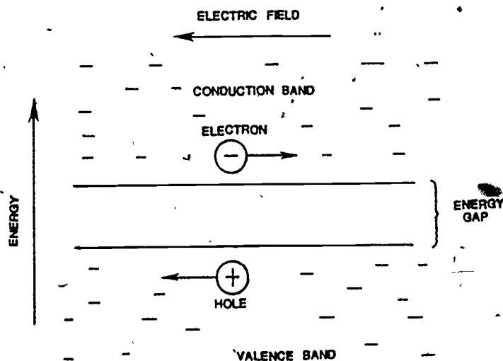
Figure 13. Diagram of Energy Gap, Conduction Band, Valence Band, and Current Carriers in a Semiconductor.
