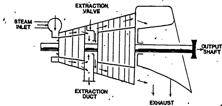
Figure 20. Single Automatic Extraction Turbine.
