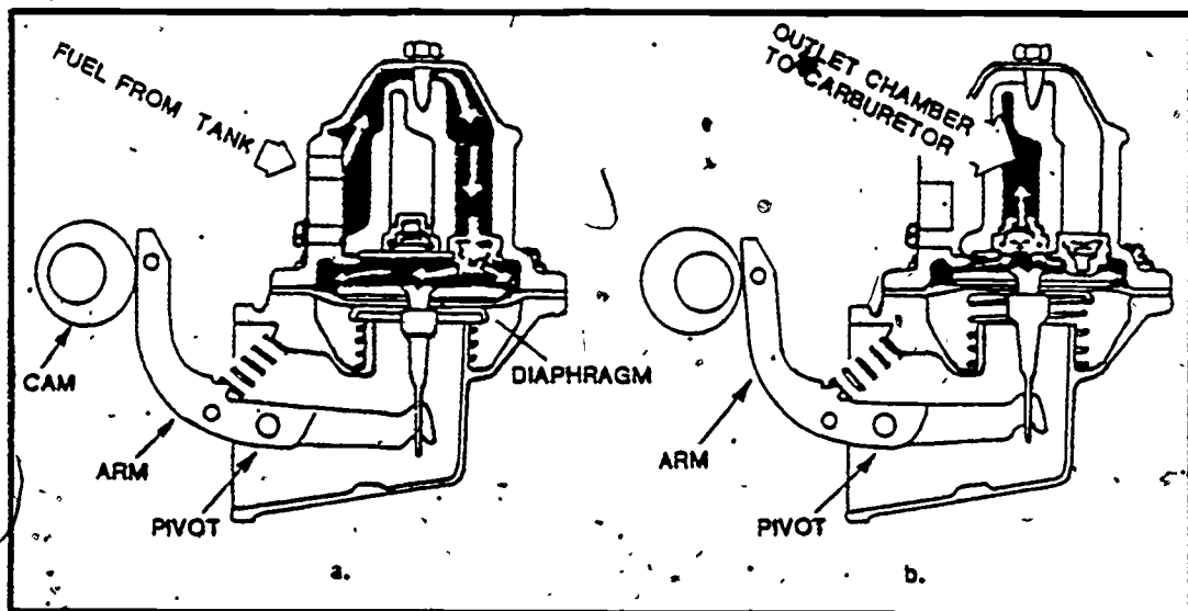
Figure 28. Typical Gasoline Fuel Pump.
