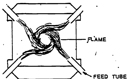
Figure 3. Corner-Fired Tangential Burning.
