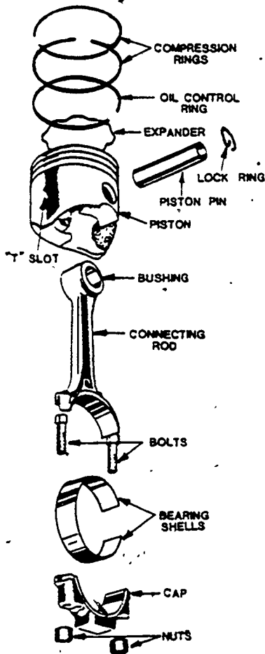
Figure 16. Exploded View of Piston and Connecting Rod Assembly.
