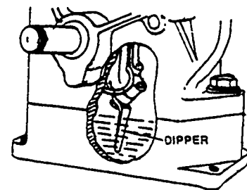
Figure 19. Splash Lubrication System.
