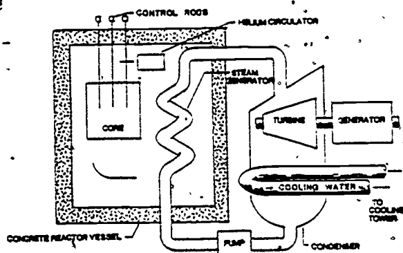
Figure 8. Diagram of a High Temperature Gas Cooled Reactor (HTGR).
