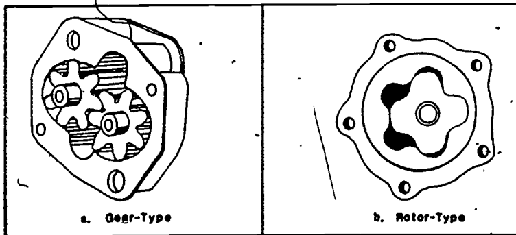
Figure 21. Oil Pumps.
