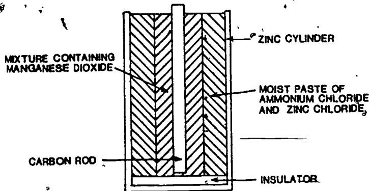
Figure 10. Diagram of Leclanche Cell.
