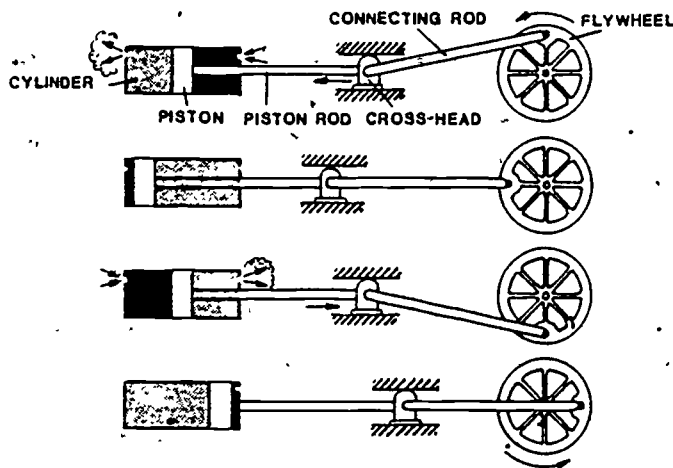
Figure 2. Schematic of a Steam Engine.
