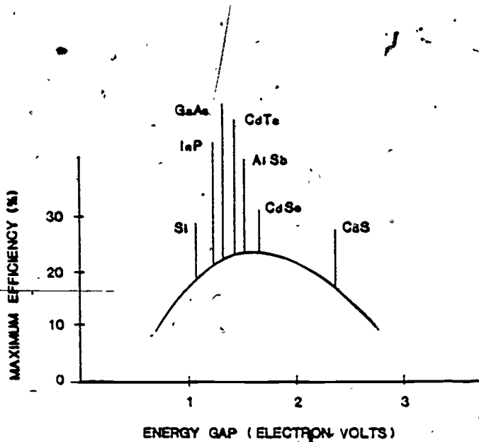
Figure 16. Maximum Photovoltaic Conversion Efficiency Vs. Semiconductor Energy Gap.
