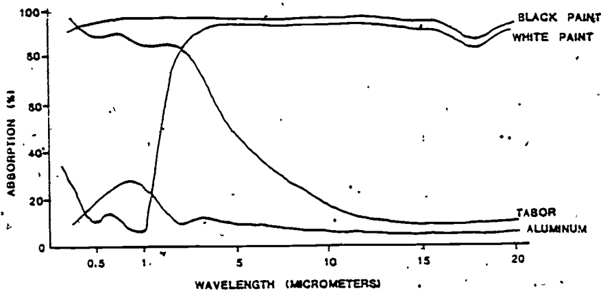
Figure 8. Absorption vs. Wavelength for Several Materials.
