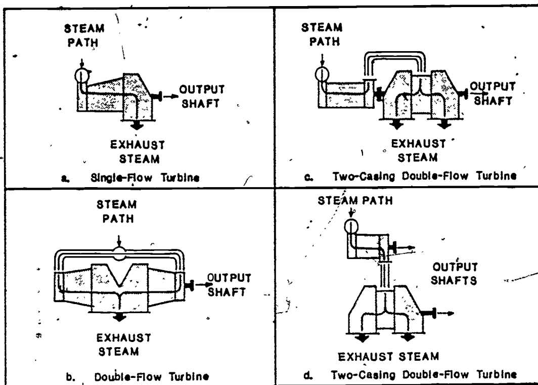
Figure 18. Steam Flow Paths for Multistage Turbines.
