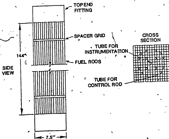
Figure 2. Schematic Diagram of Fuel Assembly Composed of 15 x 15 Array of Fuel Rods.
