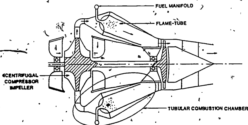
Figure 24. Cross Section of Turbine with Tubular Combustor and Centrifugal Compressor.
