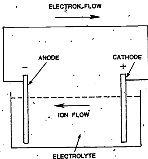
Figure 9. Diagram of Electric Cell.
