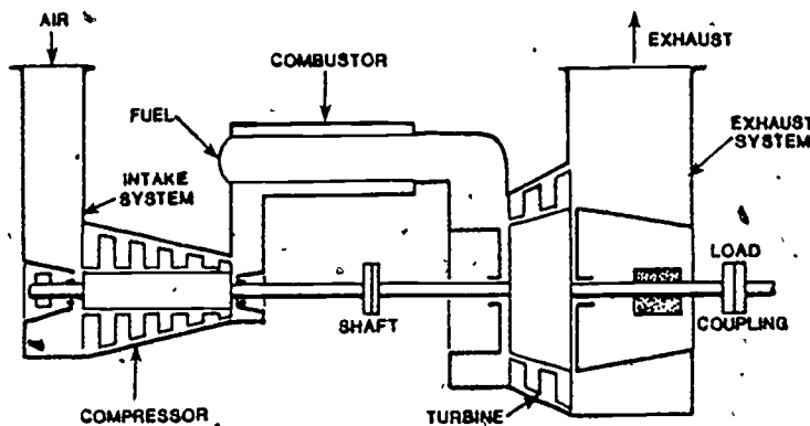
Figure 22. Schematic of a Simple Gas Turbine.
