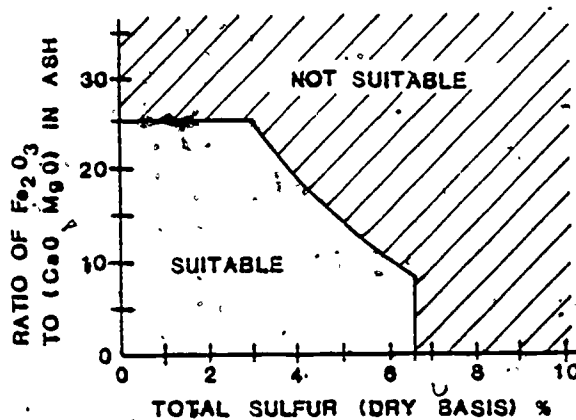
Figure 5. Suitability of Coal for Cyclone Furnaces.
