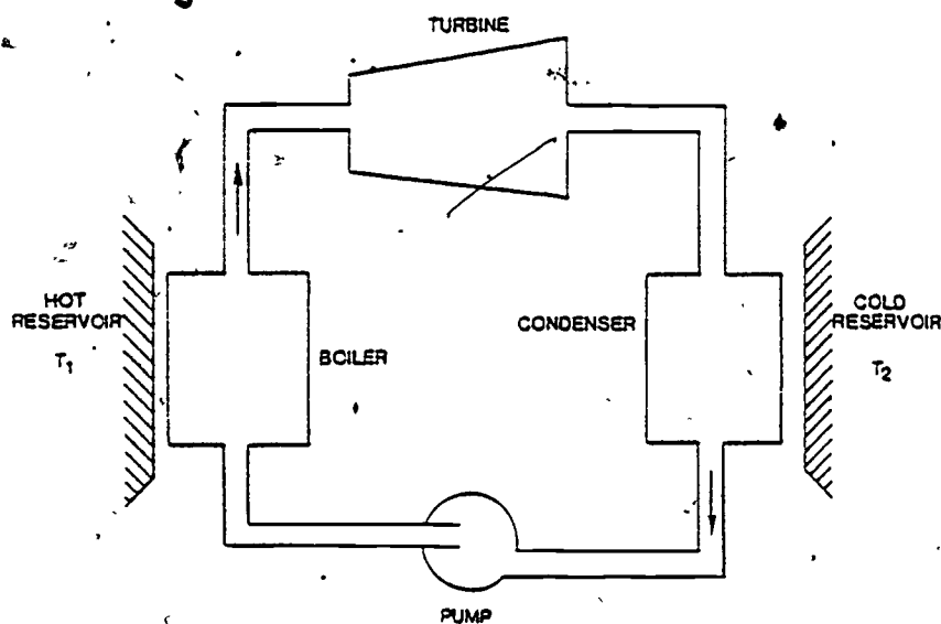
Figure 1. Elementary Steam Power Plant.
