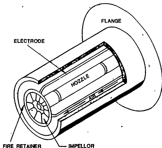
Figure 3. Cut-Away View of Burner for Gaseous or Liquid Fuels.
