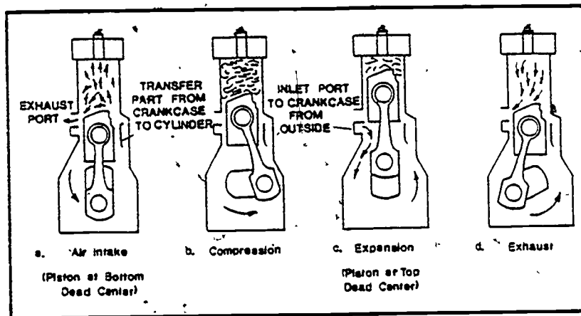
Figure 5. Two-Stroke Cycle:—One Power Stroke Out of Each Revolution.
