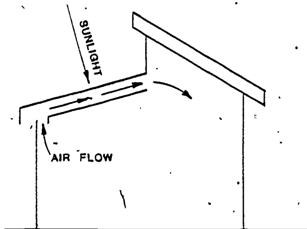
Figure 16. Schematic Diagram of a Thermosyphoning Roof.
