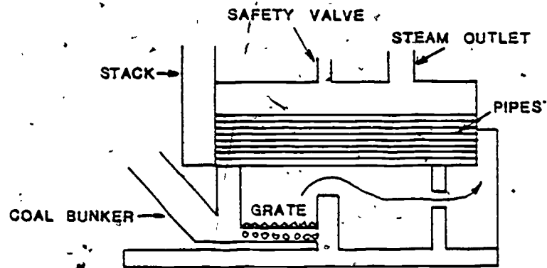
Figure 6. Schematic Diagram of a Fire-Tube Boiler with an Underfeed Coal Stoker. (Arrows show direction of gas flow.)
