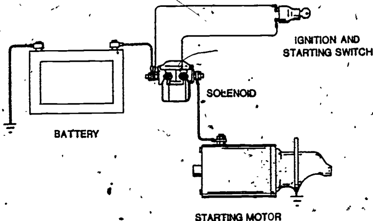
Figure 36. Schematic of a Typical Starting System.
