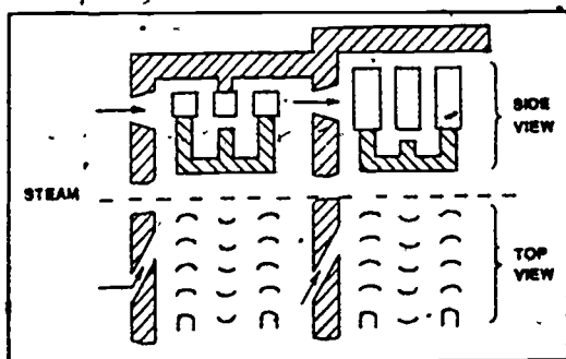
Figure 7. Top and Side Views of Combination Pressure- and Velocity-Stage Turbine.
