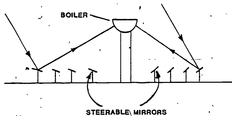
Figure 18. Tower Concept for Solar Power Generation.
