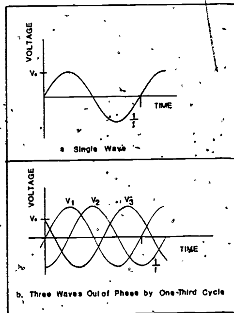
Figure 5. Sine Waves.
