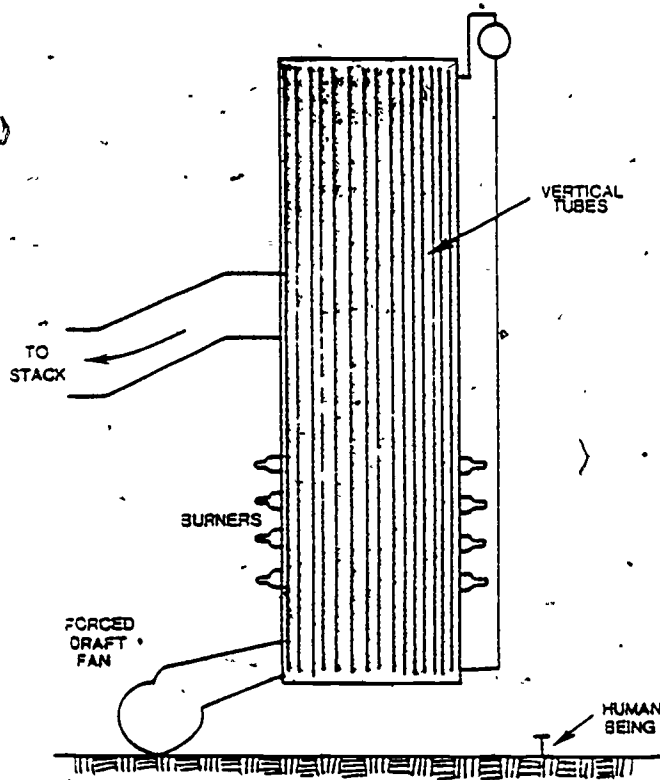
Figure 4. Schematic Diagram of a Combustion System for Gaseous or Liquid Fuels.
