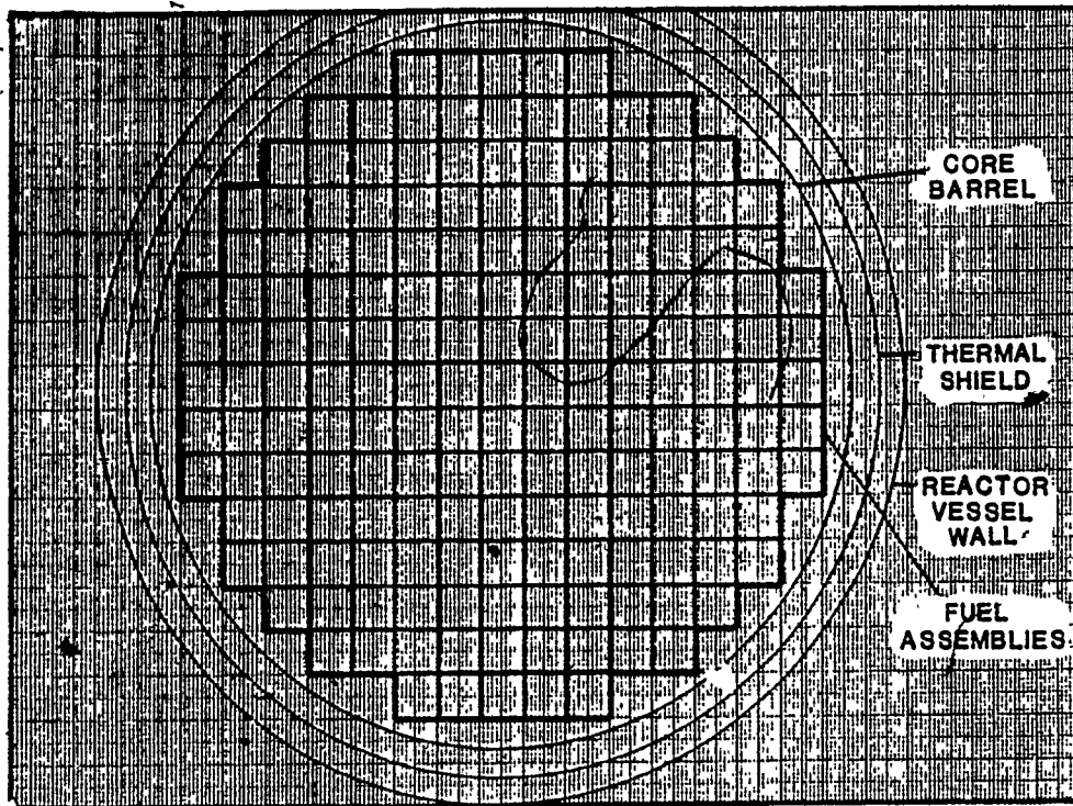
Figure 4. Schematic Diagram of Cross Section of Reactor Vessel and Core Comprised of 177 Fuel Assemblies.
