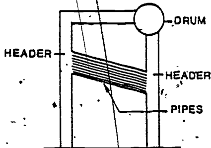
Figure 7. Schematic Diagram of a Straight Water-Tube Boiler With Inclined Tubes.
