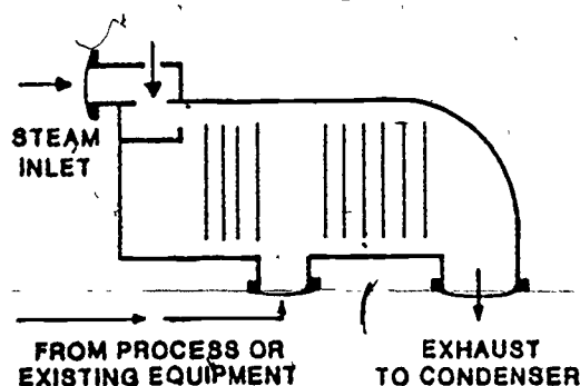
Figure 19. Mixed Pressure Turbine.
