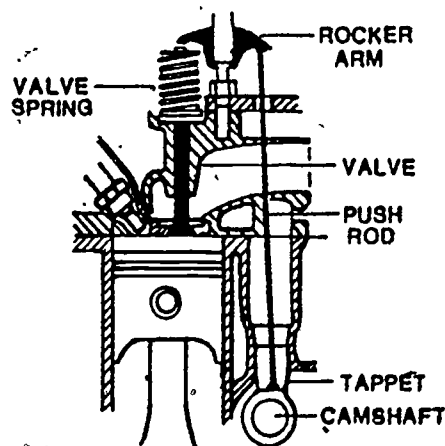
Figure 12. Valve Train.
