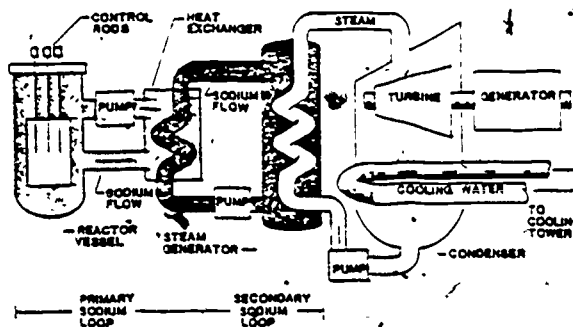
Figure 9. Diagram of Liquid-Metal Fast Breeder Reactor (LMFBFR).
