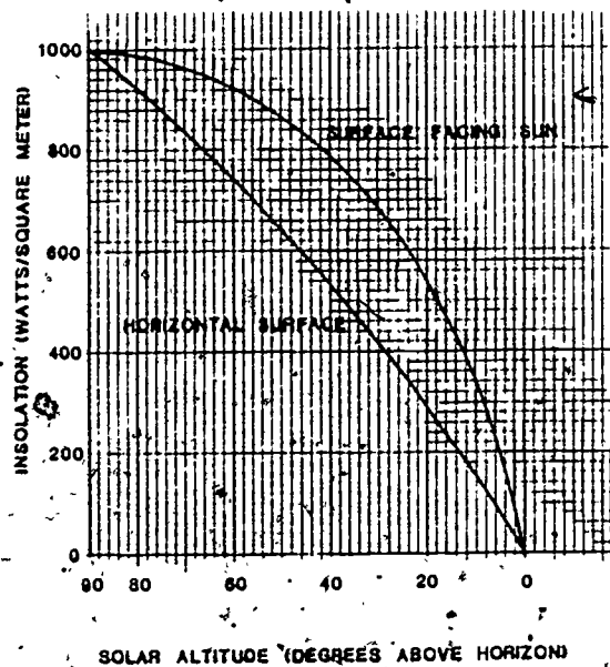
Figure 4. Insolation on Flat Surfaces on a Clear Day.
