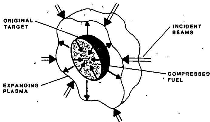
Figure 13. Diagram of Processes in Inertial Confinement Fusion.
