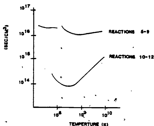
Figure 10. The Lawson Criterion.
