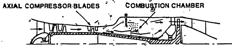
Figure 25. Cross Section of an Annular Combustion Chamber.
