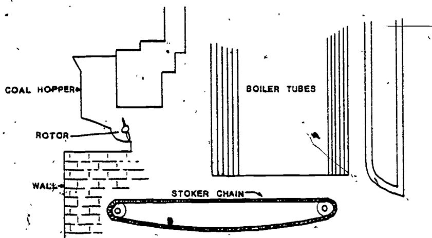
Figure 1. Schematic Diagram of a Spreader Stoker.
