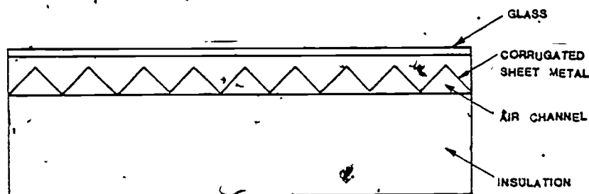
Figure 17. Typical Design for Flat-Plate Collector, Using Air as the Working Fluid.
