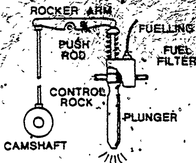
Figure 26. Unit-Injection Fuel
