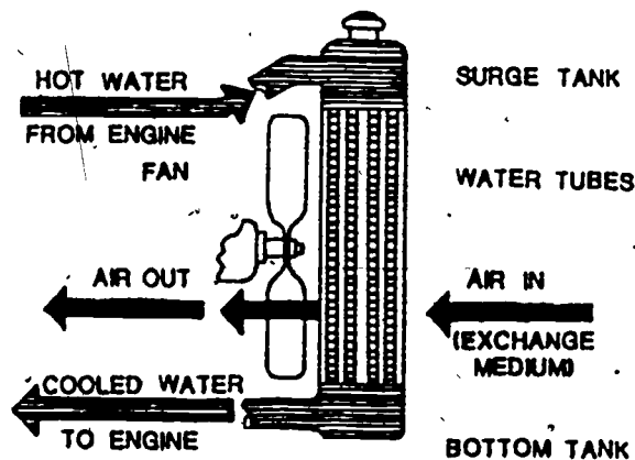
Figure 8. Radiator.
