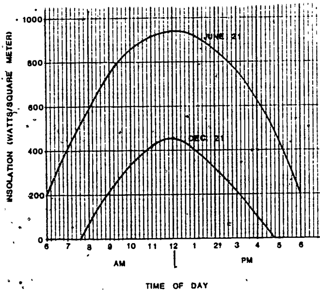
Figure 3. Insolation on a Horizontal Surface for 40^\circ North Latitude.
