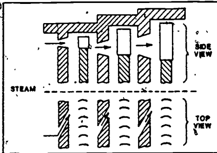
Figure 6. Top and Side Views of Pressure-Stage Impulse Turbine.
