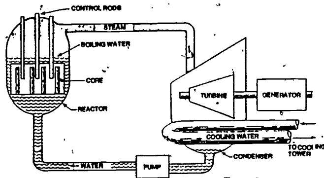
Figure 5. Diagram of a Boiling Water Reactor System.
