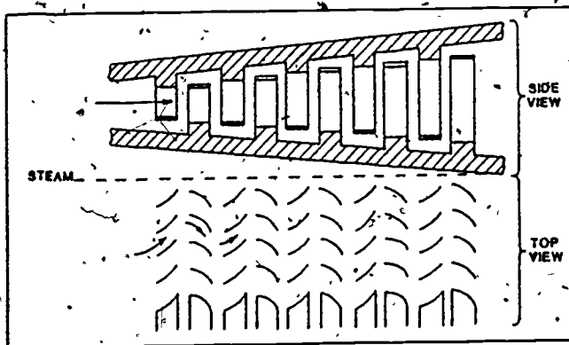
Figure 9. Top and Side View of Reaction Turbine.
