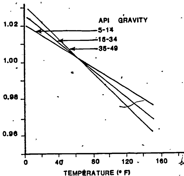
Figure 1. Temperature Dependent Correction Factor for Fuel Oil Volume.
