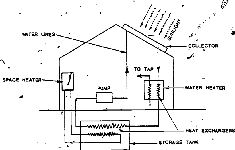
Figure 14. Sample System for Solar Space and Water Heating.
