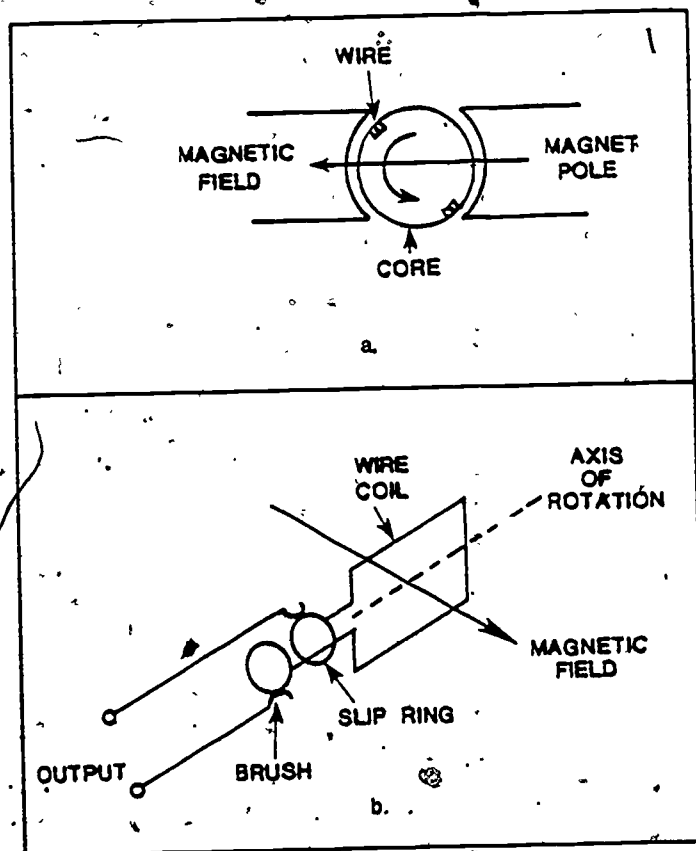
Figure 4. Configurations of an Alternating Current Generator.
