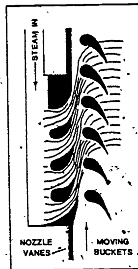
Figure 8. Schematic of Reaction-Stage Blading.
