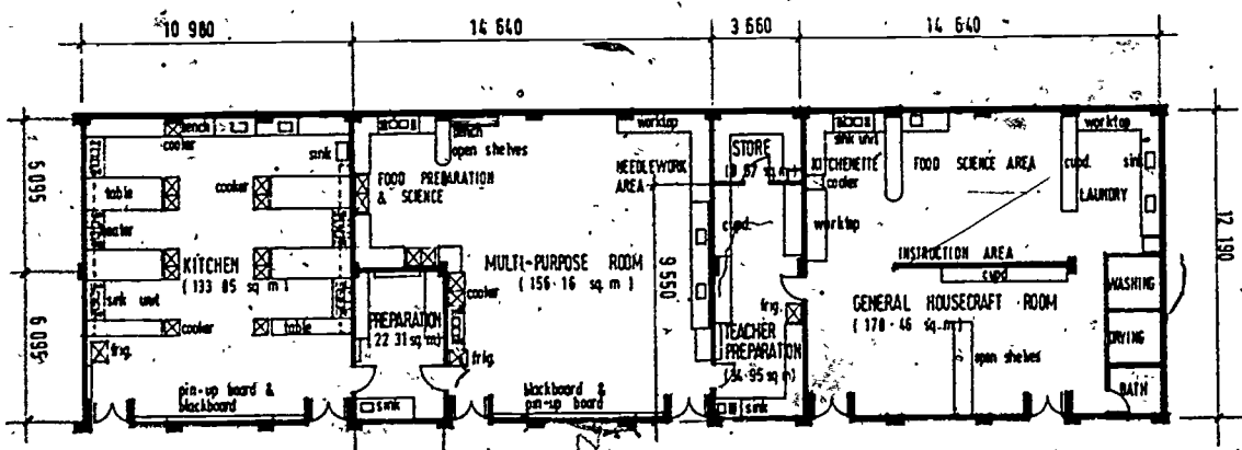
Figure 15. Layout plan of home economics rooms (Science block 2nd floor)
