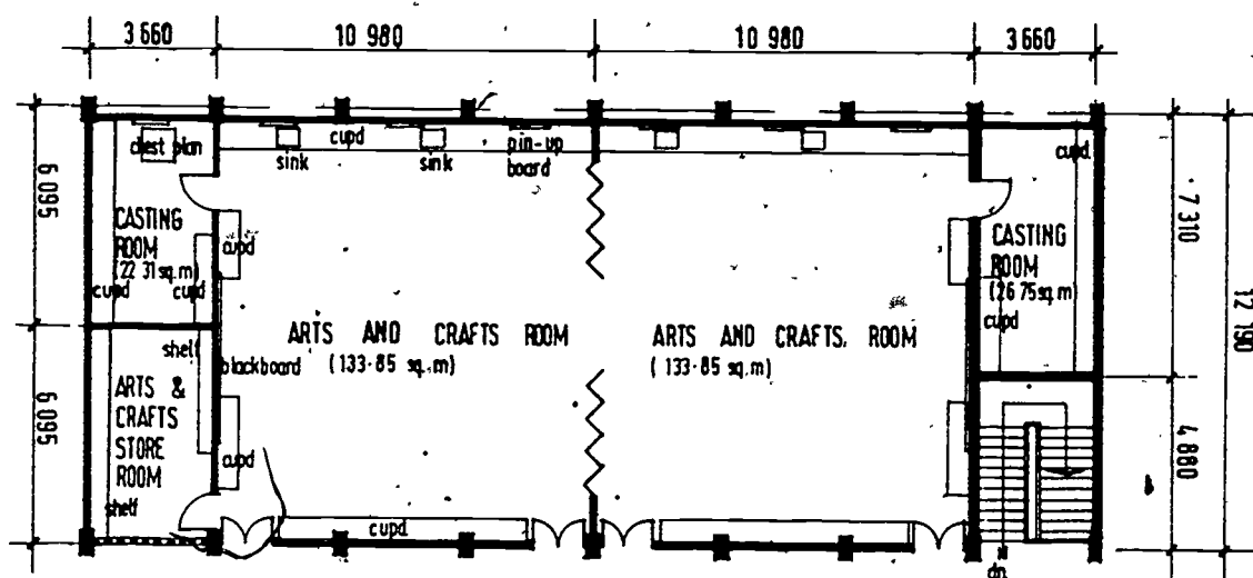
Figure 18. Layout plan of art and crafts rooms (Workshop block, 2nd floor)
