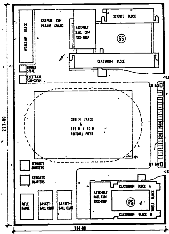
Figure 6. Layout plan for a combination of a primary and a secondary school
