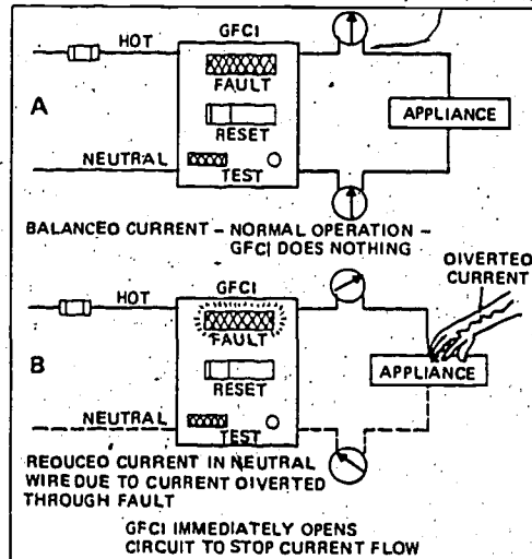
Fig. 7-8. Ground fault circuit interrupters (GFCI).
