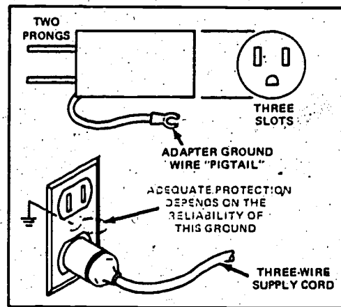
Fig. 7-10. Proper use of equipment grounding adapter.
