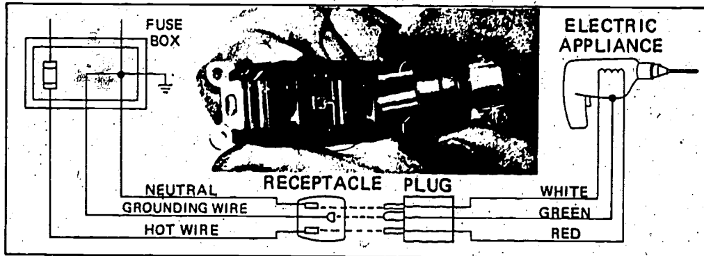
Fig. 7-7. Typical equipment grounding circuit.
