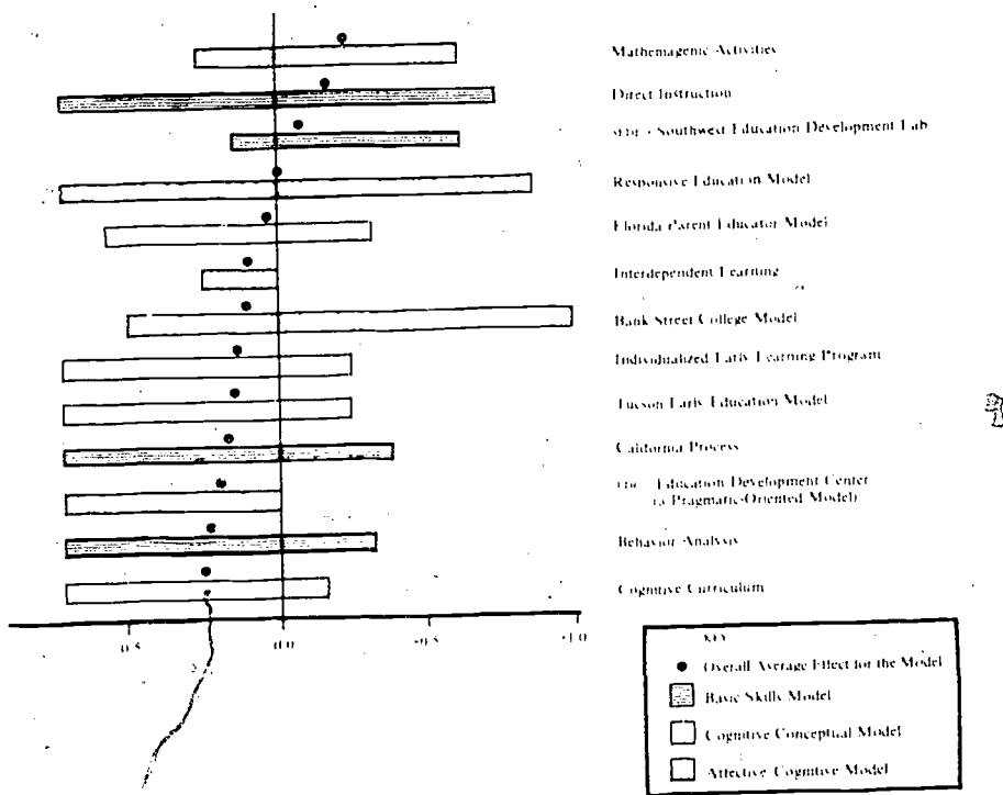
Figure 3 Ranges of Site Average Effects on Cognitive Conceptual Skills for Thirteen Follow Through Models 18
