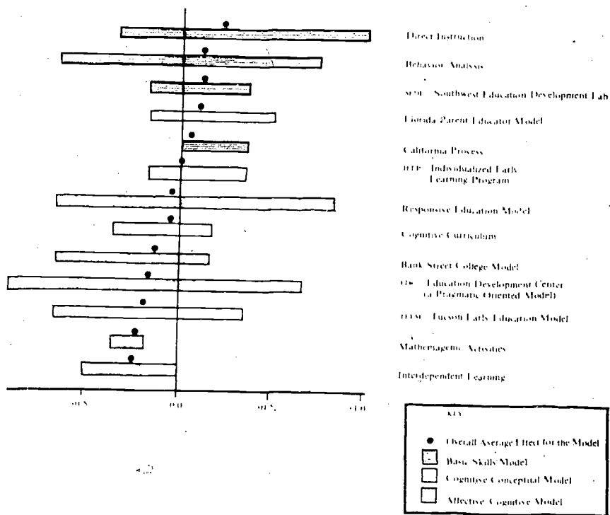
Figure 4 Ranges of Site Average Effects on Affective Outcomes for Thirteen Follow Through Models 19
