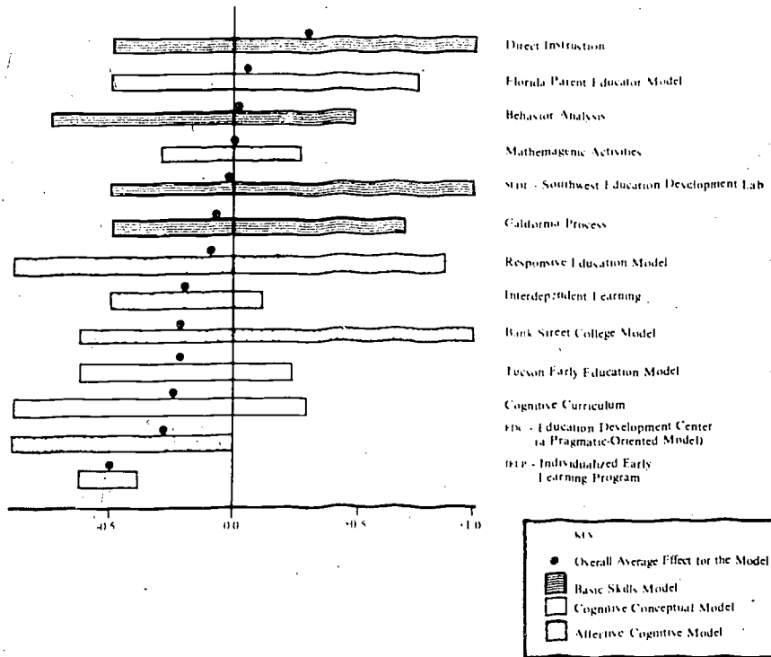
Figure 2 Ranges of Site Average Effects on Basic Skills for Thirteen Follow Through Models 17
