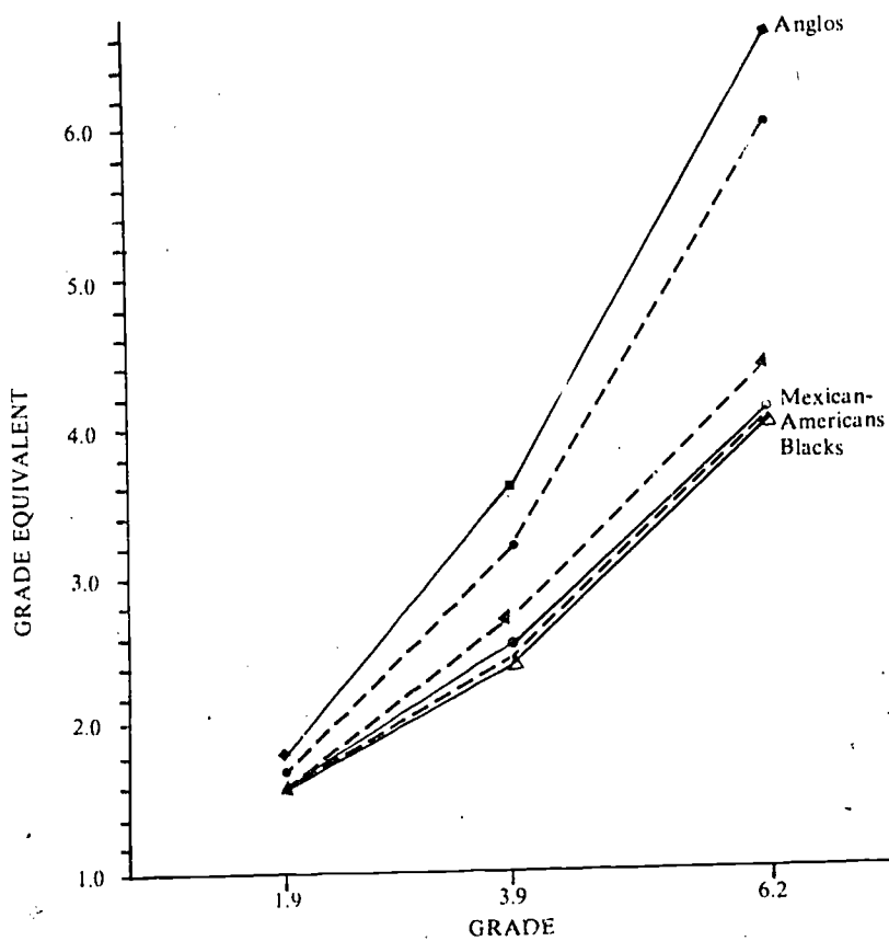
Figure 1 Mean reading achievement for the longitudinal (solid lines) and cross sectional (dashed) samples of Anglos, Mexican-Americans, and Blacks. 4
