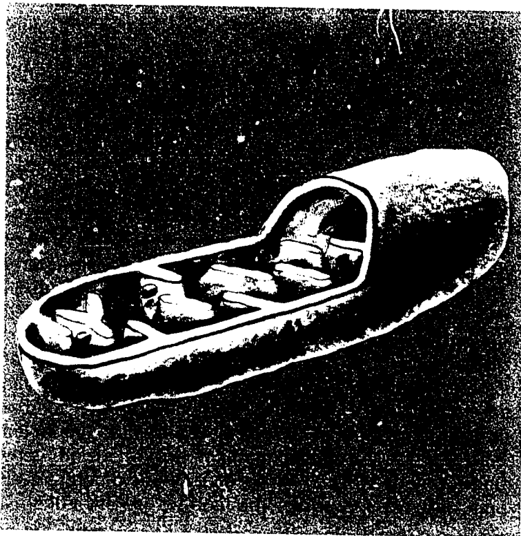
A mitochondrion.
