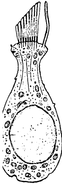
Hair cell
