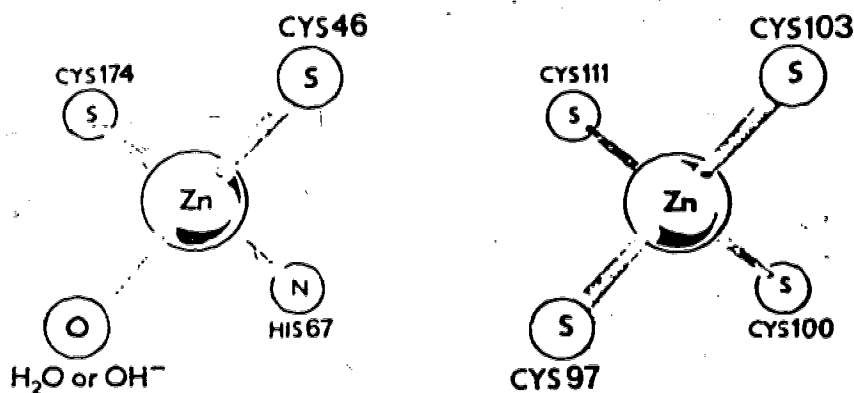
Figure 2. Ligands of the Catalytic (left) and Structural (right) Zinc Atoms in Horse Liver Alcohol Dehydrogenase
