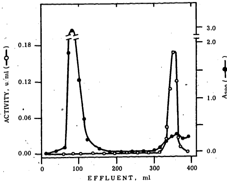
Figure 4. AMP-Agarose Affinity Chromatography of \Pi -ADH
