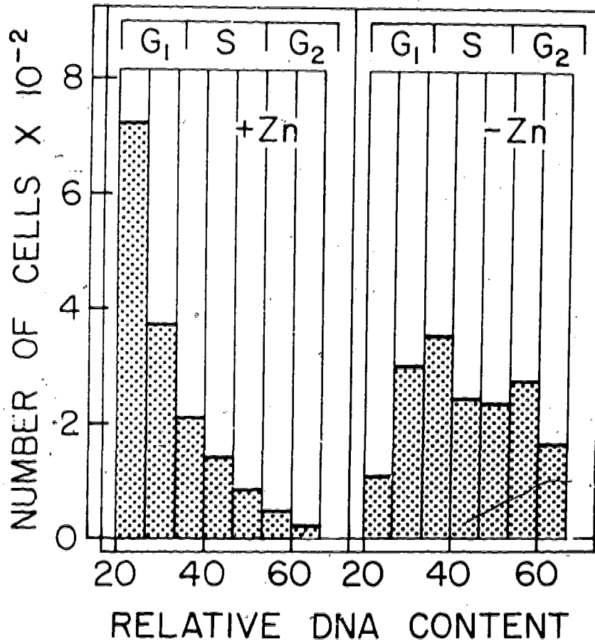
Figure 3. Comparison of DNA Histograms of (+Zn) and (-Zn) E. gracilis
