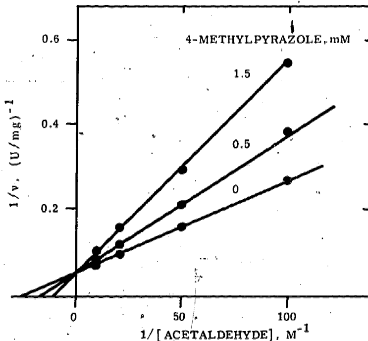
Figure 5. 4-Methylpyrazole Inhibition of Acetaldehyde Reduction by \Pi -ADH
