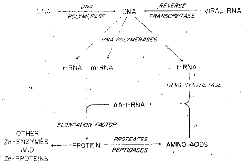
Figure 6. Zinc in Nucleic Acid and Protein Metabolism
