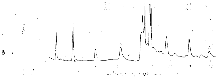
Figure 8. High-Pressure Liquid Chromatographic Analysis of Base Composition of mRNA from (+Zn) and (-Zn) E. gracilis
