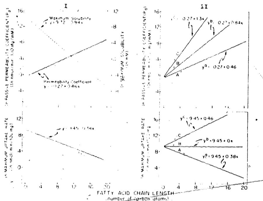
Figure 5. Effect of the Relative Polarity of a Solute Molecule on Its Maximum Rate of Transmembrane Movement
