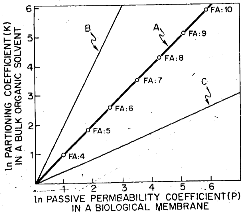
Figure 3. Comparison of Passive Permeability Coefficients ( P ) for a Series of Fatty Acids With the Partitioning Coefficients of These Same Molecules Between Bulk Buffer Solution and a Bulk Organic Solvent
