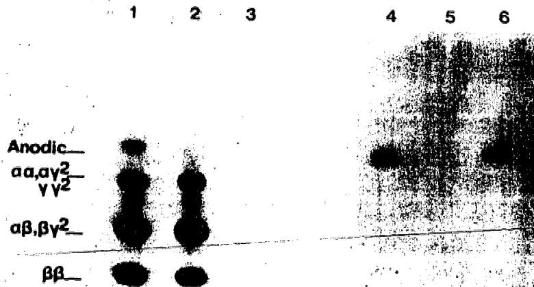
Figure 3. Identification of the Human ADH Molecular Forms in Liver Homogenate and the Enzyme Fractions Separated by CapGapp-Sephrose
