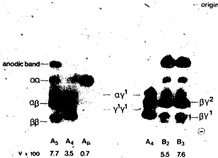
Figure 1. Starch Gel Electrophoresis of Human Liver ADH Obtained from Autopsy (A) and Biopsy (B) Specimens
