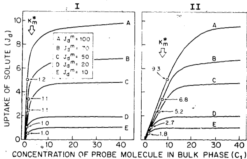
Figure 11. Effect of the Maximal Transport Rates ( J_d^m ) on the Apparent K_m Values in the Presence of a Diffusion Barrier of Low and High Resistance
