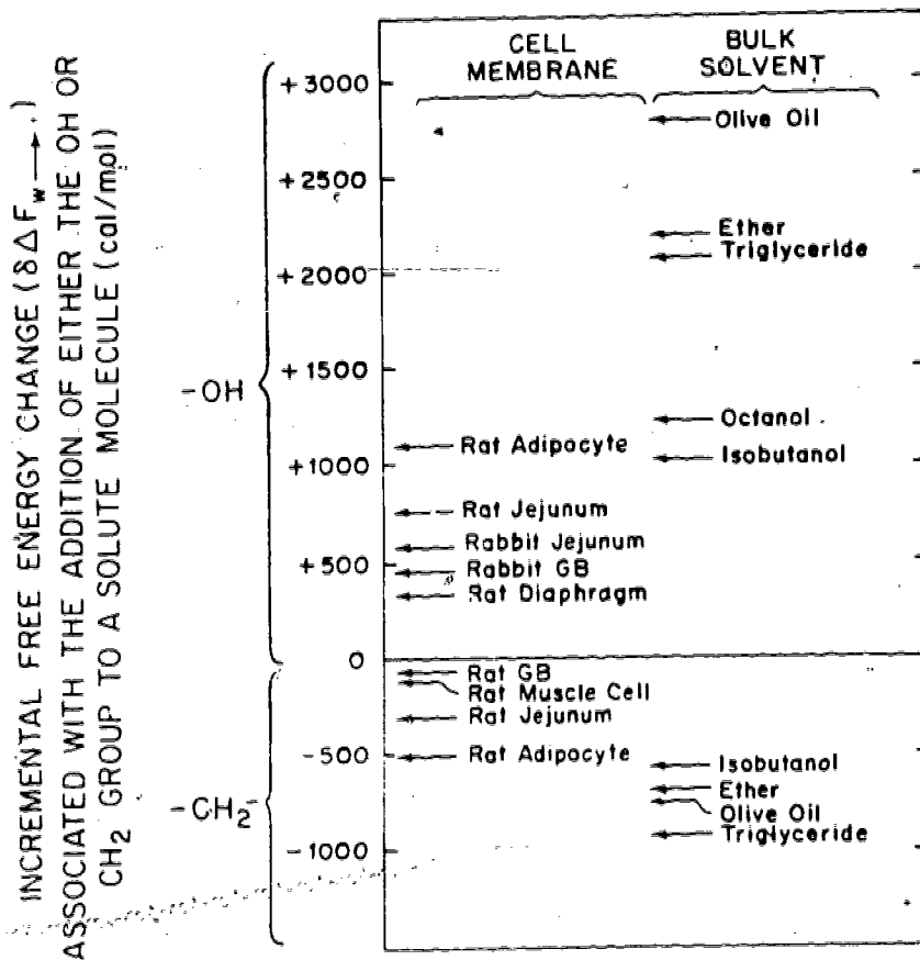
Figure 4. Incremental Free Energy Changes ( \delta\Delta F_{w-1} ) Associated With the Addition of Either the -OH or -CH 2 - Groups to a Solute Molecule
