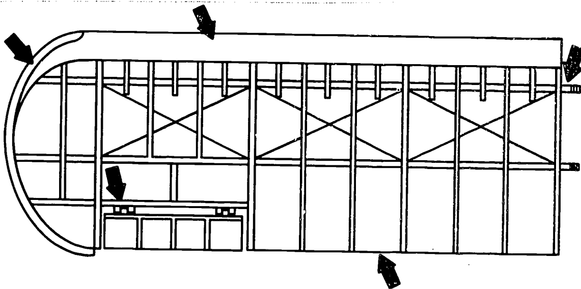
FIGURE 5-3. Wood structure inspection points.
