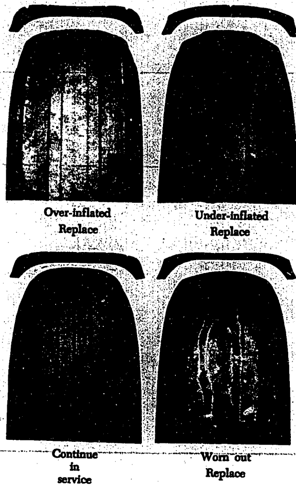
FIGURE 4-1. Examples of tire defects.
