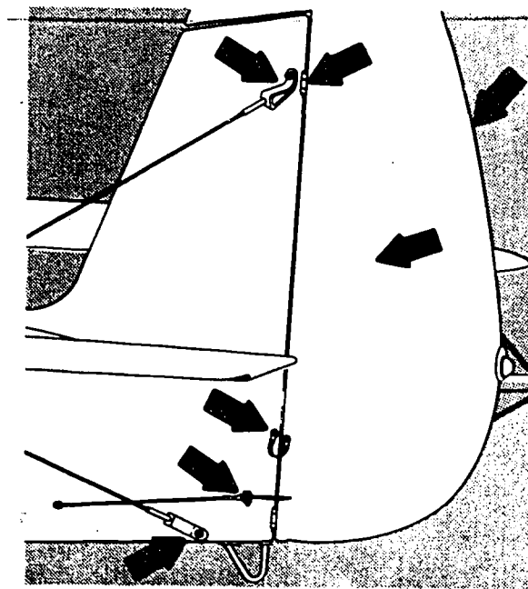
FIGURE 6-4. Rudder checkpoints.
