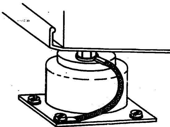
FIGURE 8-3. Bonding radio equipment to shock mount.
