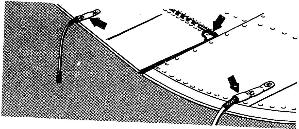
FIGURE 8-9. Bonding wires and trailing edge static wicks.
