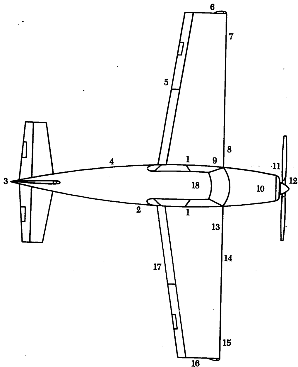
FIGURE 10-1. Inspection chart—preflight.
