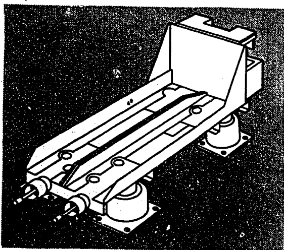
FIGURE 8-4. Communication/navigation equipment shock mount.
