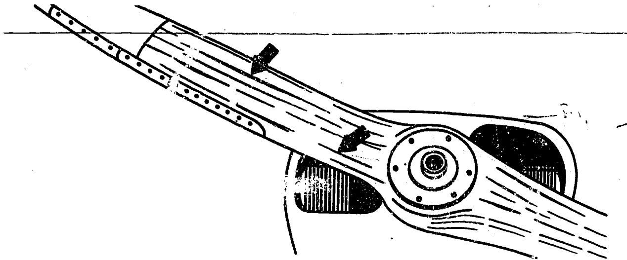
FIGURE 7-5. Wood propeller blade—cracked and separated laminations.
