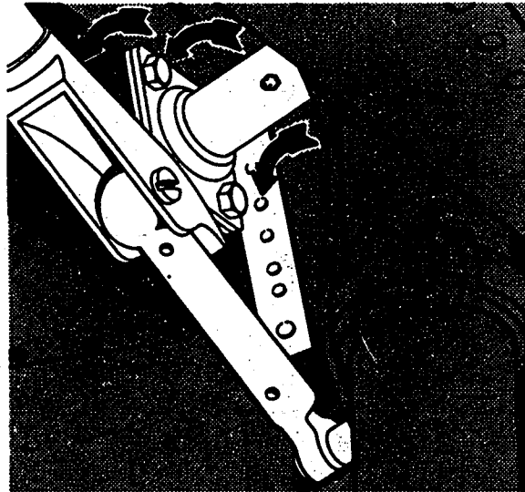
FIGURE 4-24. Gear attachment structure checkpoints.
