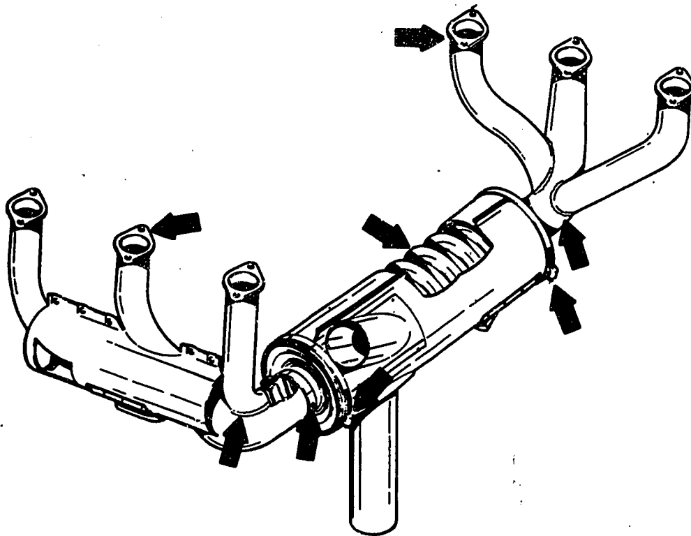
FIGURE 3-15. Exhaust manifold checkpoints.
