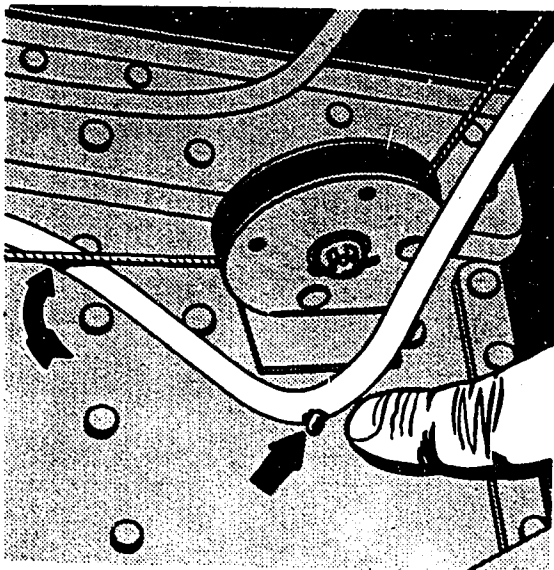
FIGURE 1-11. Leakage from chafed hydraulic line.
