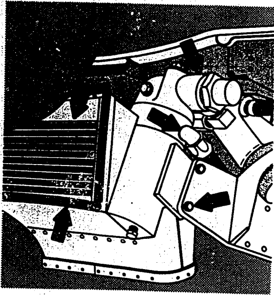
FIGURE 3-11. Oil-cooler checkpoints.
