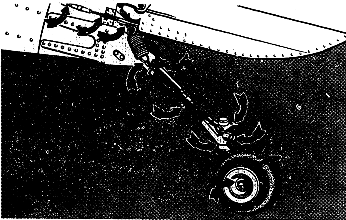
FIGURE 4-15. Steerable tailwheel inspection points.
