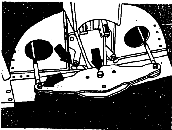
FIGURE 2-7. Bellcrank checkpoints.
