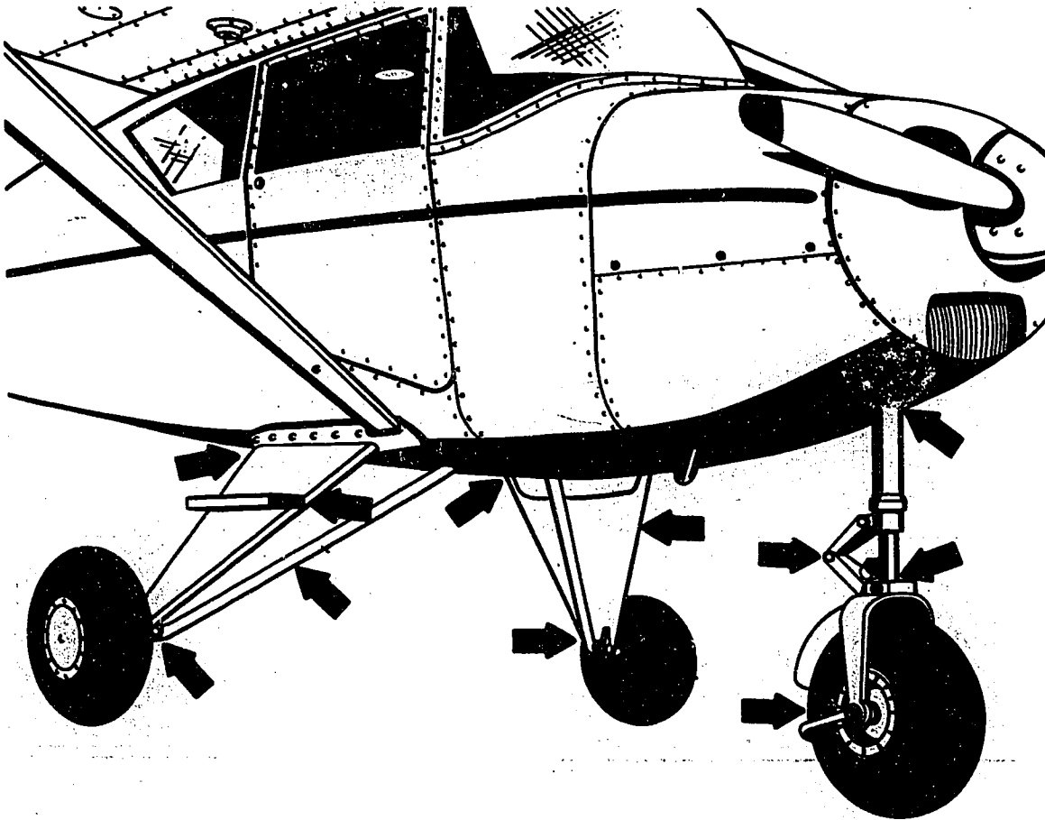
FIGURE 4-11. Wheel checkpoints.
