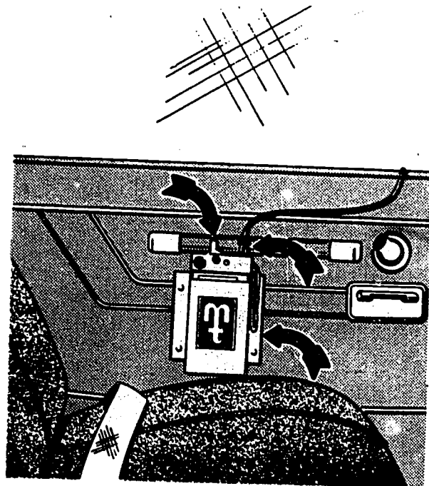
9-4. Emergency locator transmitter – portable mount.
