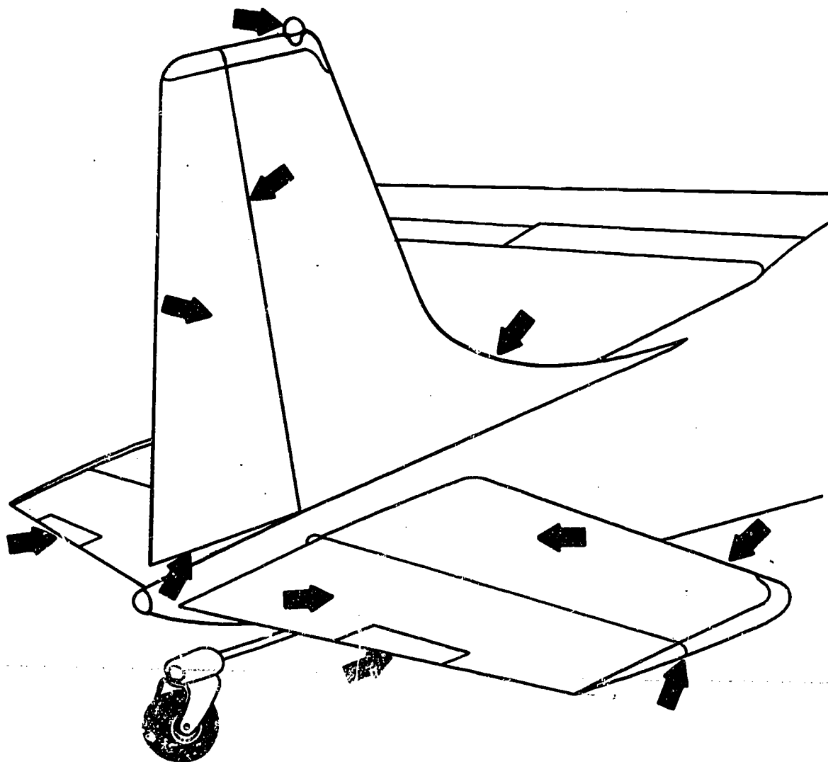
FIGURE 6-1. Inspection chart—empennage.
