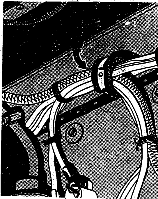
FIGURE 5-10. Electrical wiring, proper routing.
