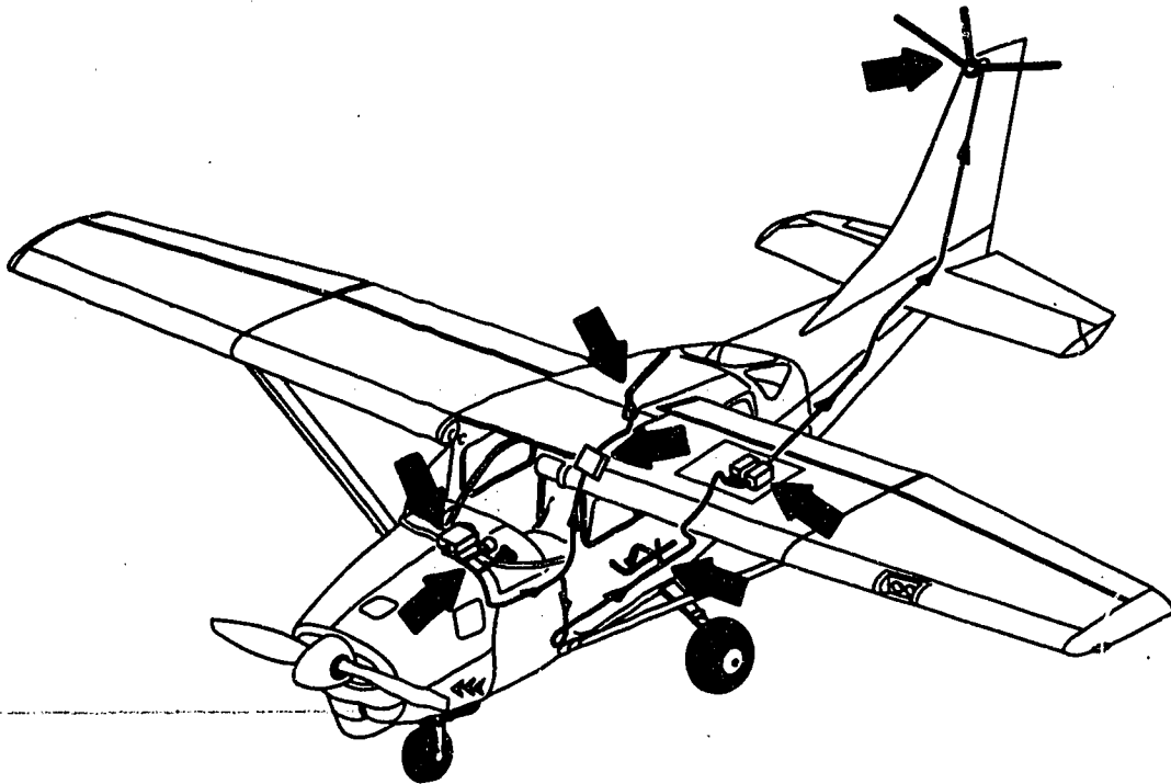
FIGURE 8-1. Inspection chart—radio.
