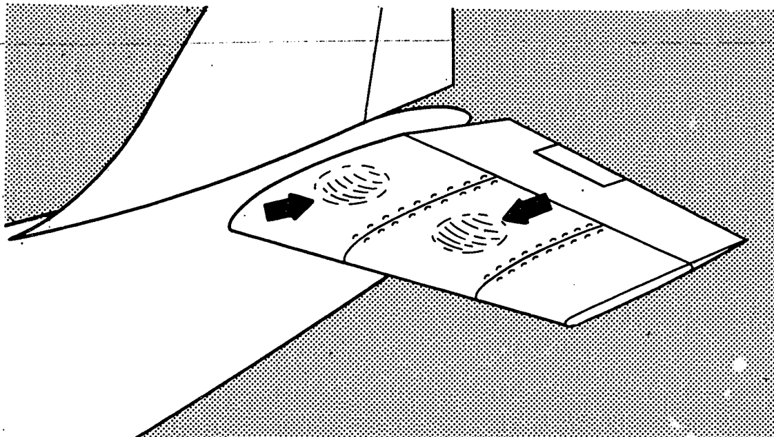
FIGURE 6-2. Oilcanning of metal skin.
