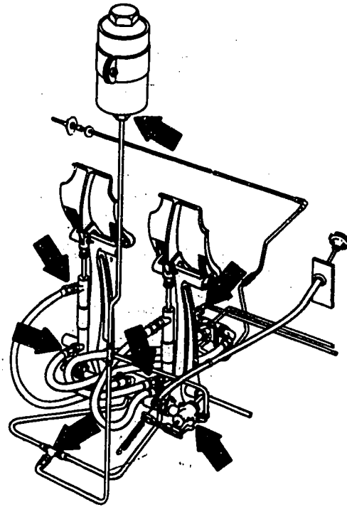
FIGURE 4-10. Cockpit-hydraulic brake line checkpoints.
