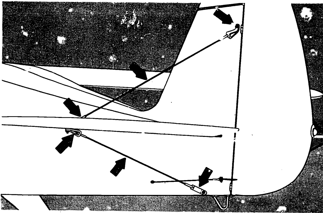
FIGURE 6-3. External bracing checkpoints.
