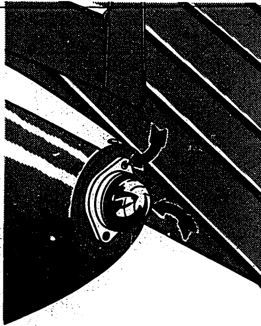
FIGURE 6-7. Position light checkpoints.
