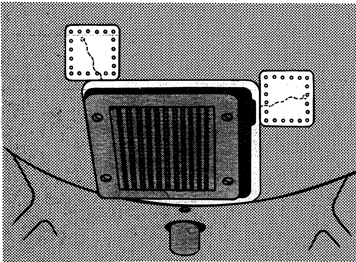
FIGURE 3-25. Repaired cowling.
