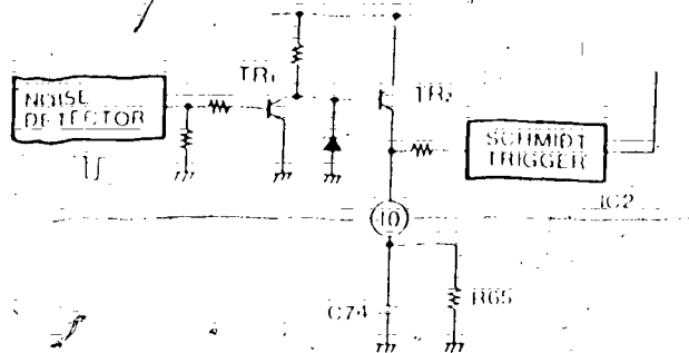
Fig. 25 Monostable multivibrator basic circuitry
