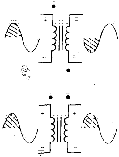
Fig. 8-26. Wave form relationships between input and output of a transformer.
