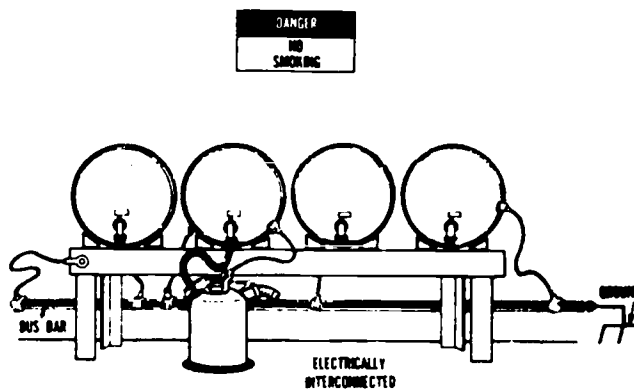
Drums grounded and bonded to receiving container
