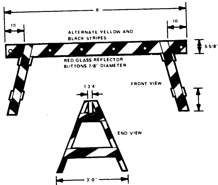
Example of Acceptable Barricade
