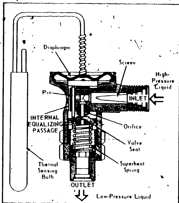
INTERNALLY EQUALIZED VALVE
