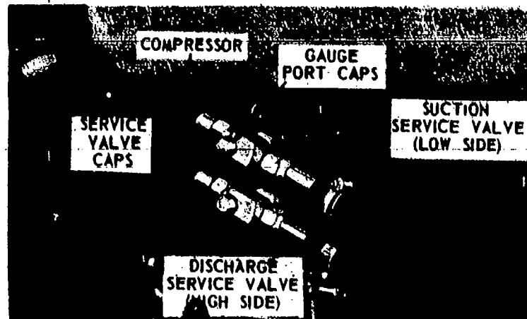
Fig. 44 — Location Of Service Valves In A Typical System
