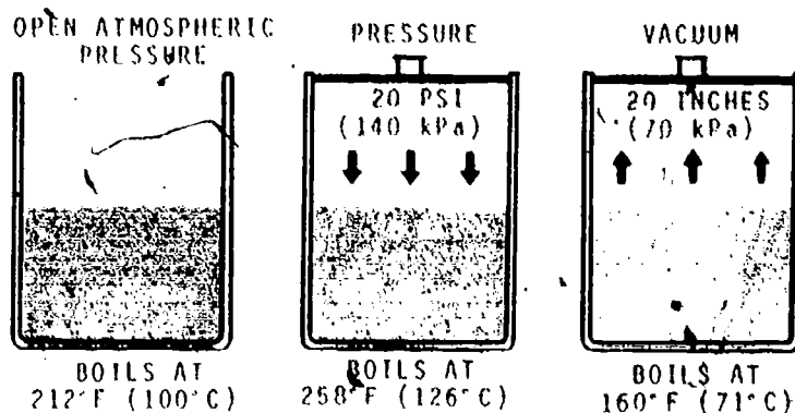
Fig. 6 - When A Liquid (Water) Boils At Various Pressures
