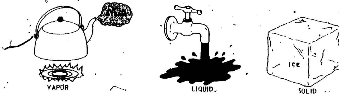
Fig. 3 — Water In The Three States Of Matter
