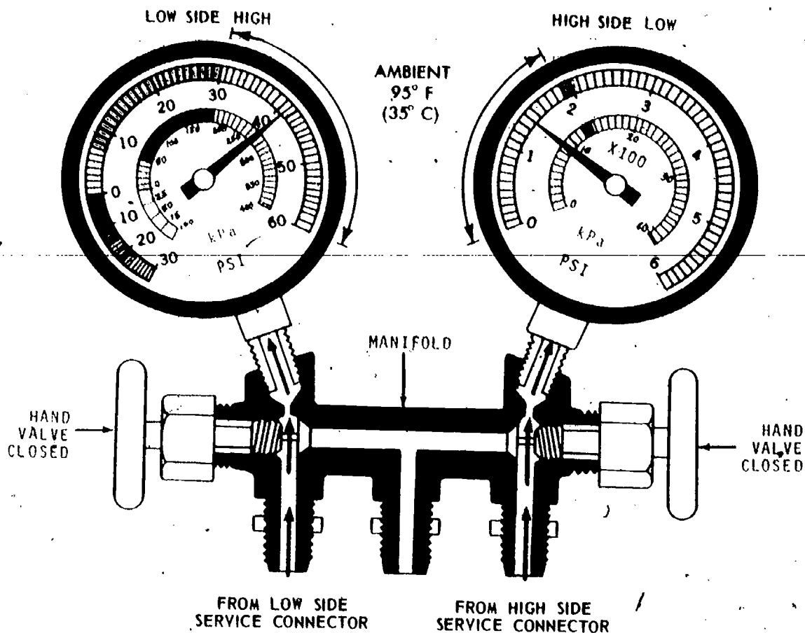
Fig. 63 — Condition No. 4
