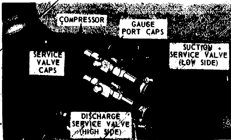
Fig. 86 — Service Valve On Compressor
