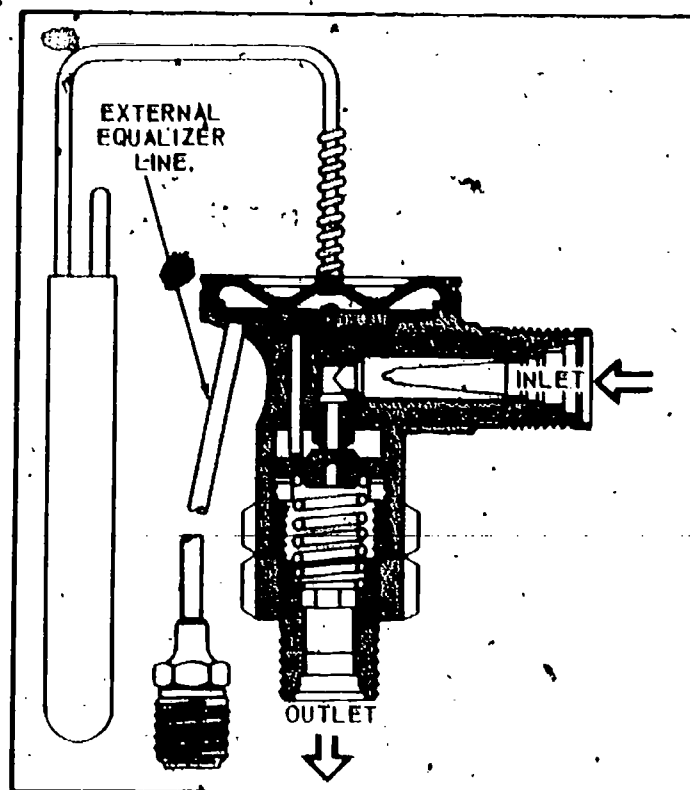
EXTERNALLY EQUALIZED VALVE
