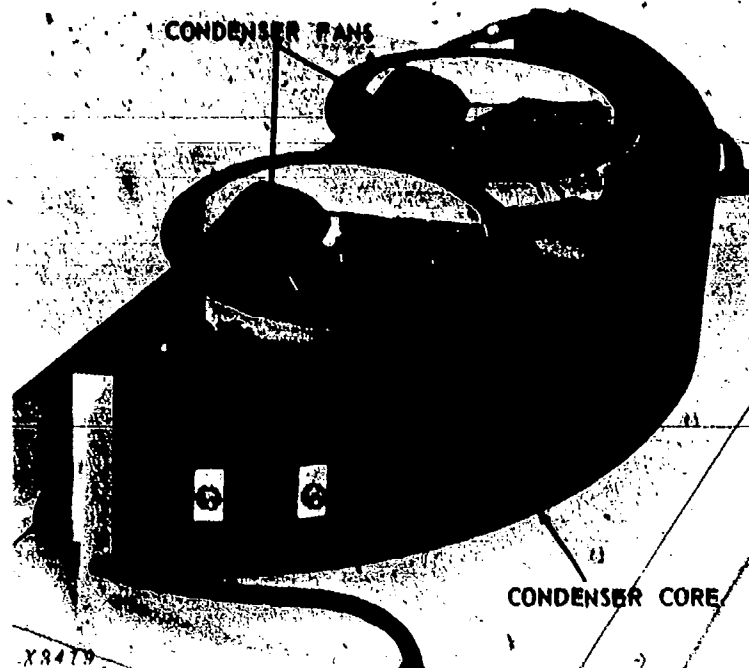
Fig. 23 — Forced Air Condenser
