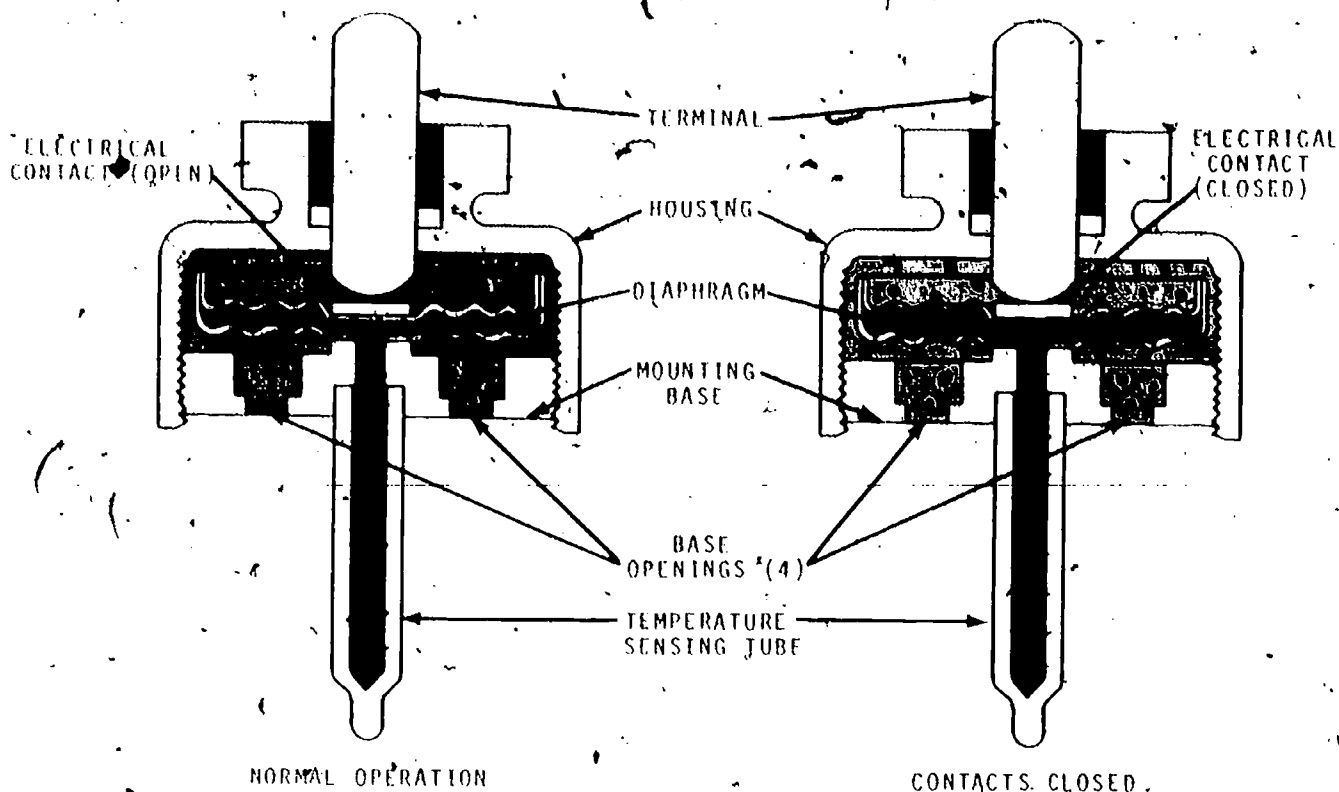
SUPERHEAT SHUTOFF SWITCH
