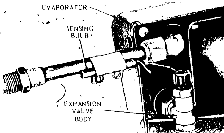
Fig 25 - Expansion Valve
