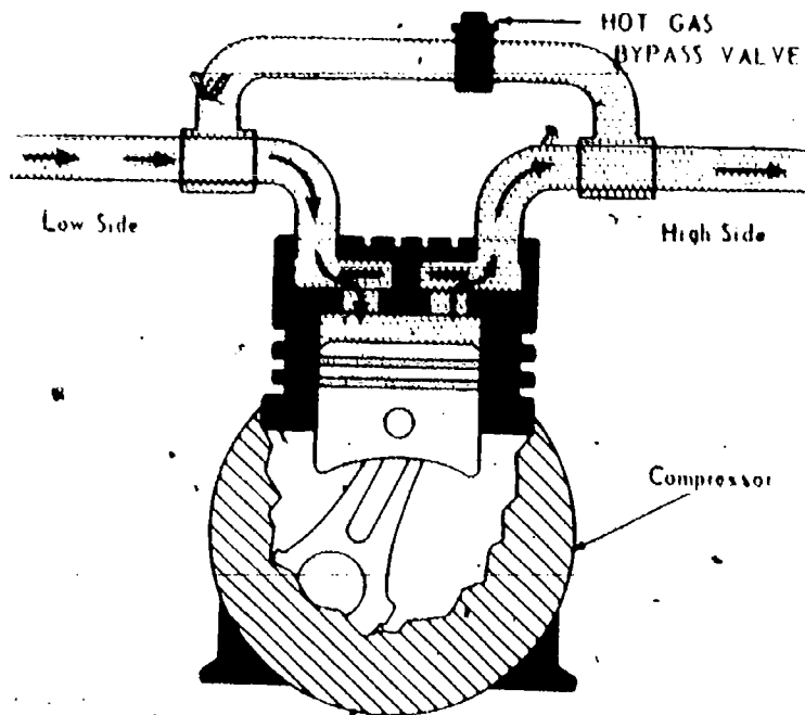
Fig. 33 — Hot Gas Bypass System.
