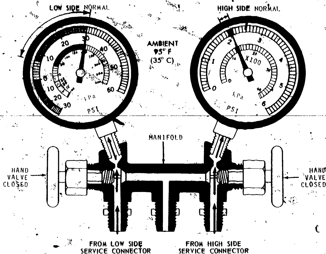
Fig. 59 — Condition No. 3
