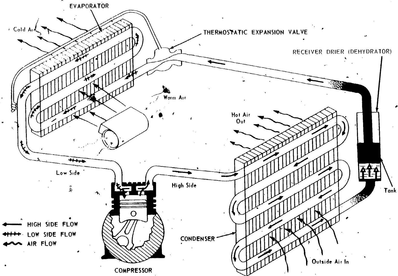
Fig. 27 — Air Conditioning System With Receiver-Drier (Dehydrator) Added
