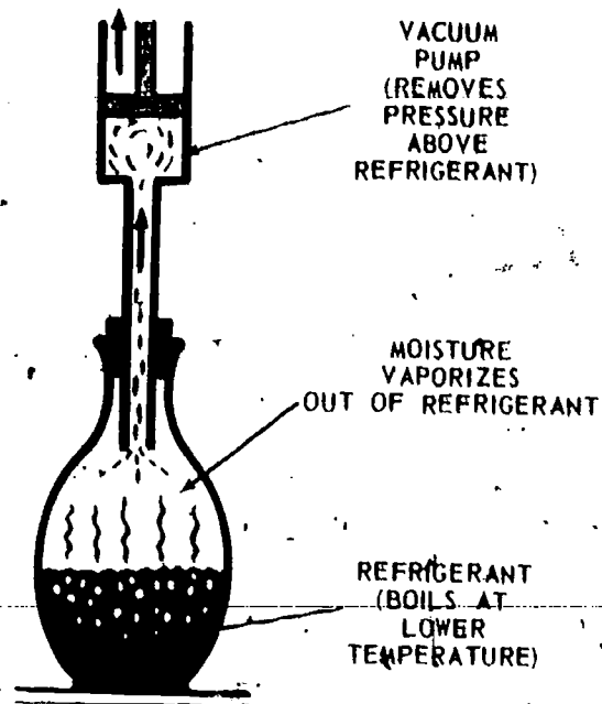
Fig. 11 — Boiling Of Liquid Under A Decrease in Pressure
