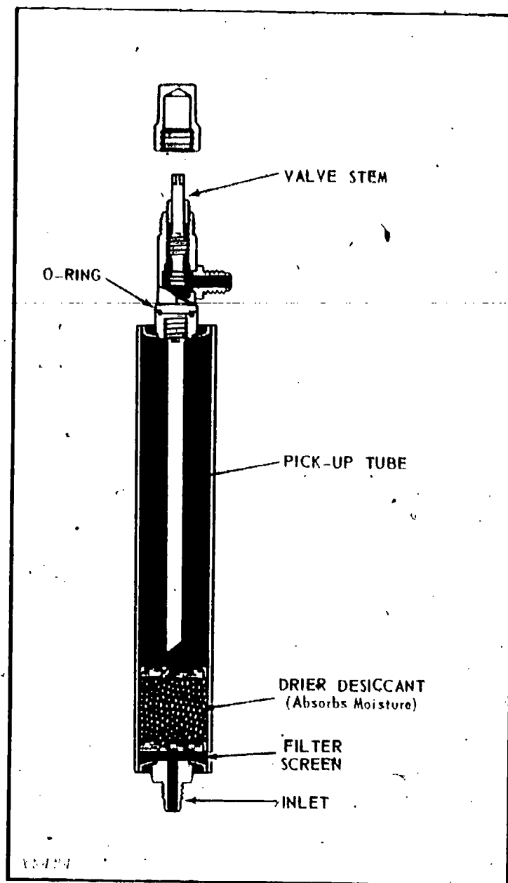
Fig. 28 — Receiver-Drier (Dehydrator)
