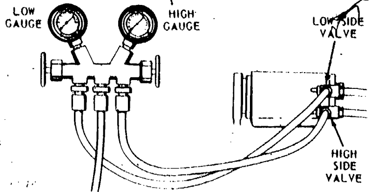
Fig 65 - First Identify and Connect Test Hose into High Side Of System
