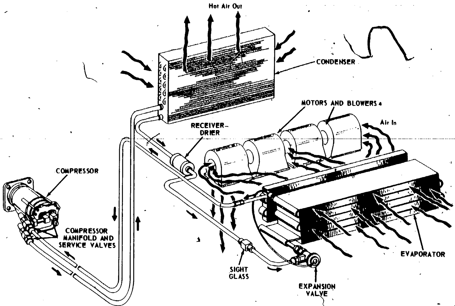
Fig. 51 — Basic Air Conditioning System For Farm Or Industrial Tractor With Cab
