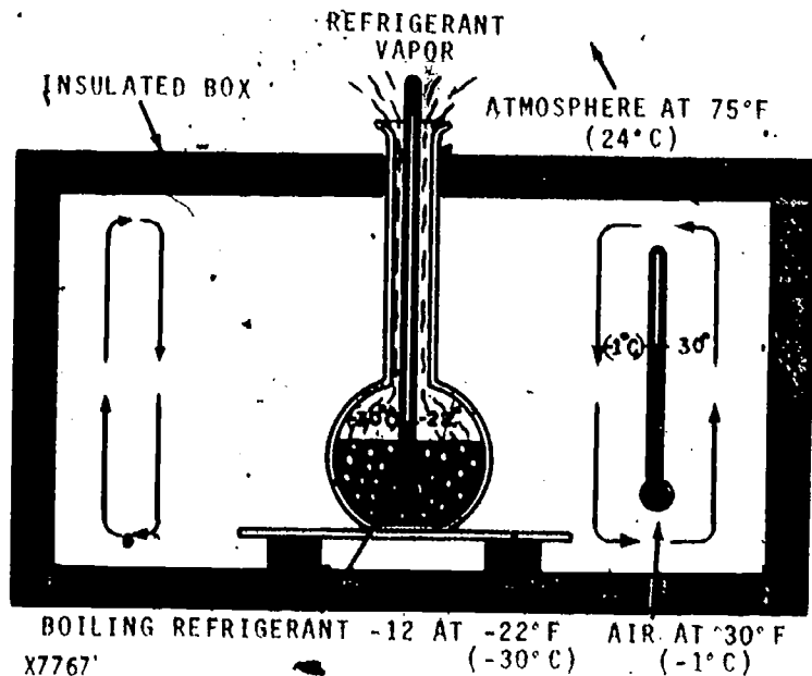
Fig. 9 - How Refrigeration Is Produced By Evaporating Refrigerant-12
