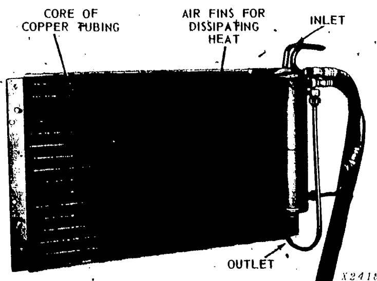
Fig. 22 — Condenser
