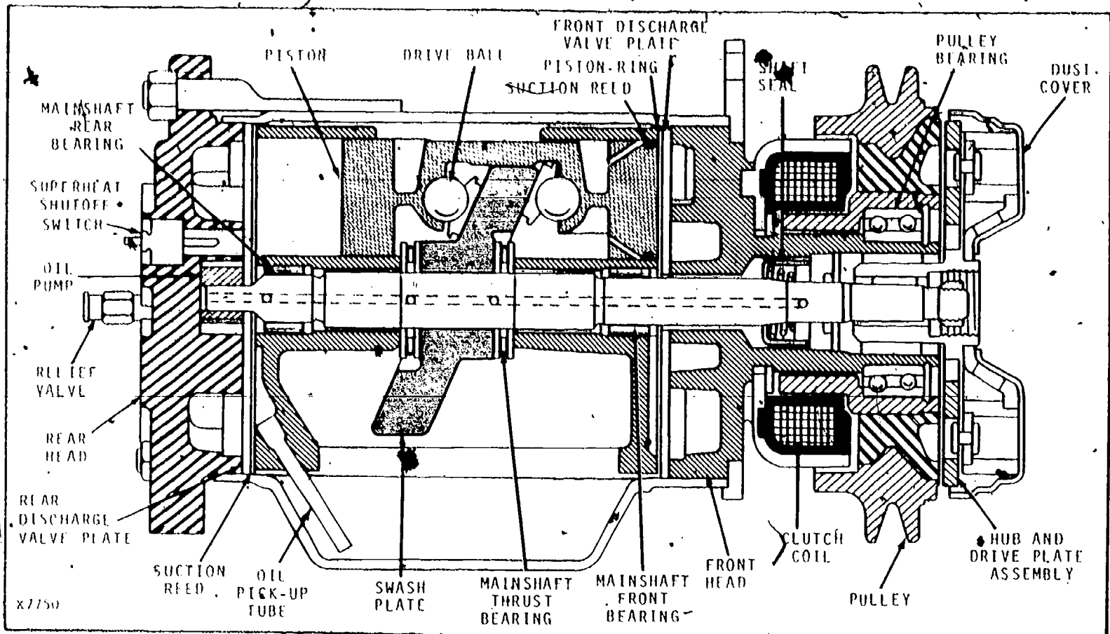
Fig. 19 — Axial Piston Compressor Controlled By Swashplate
