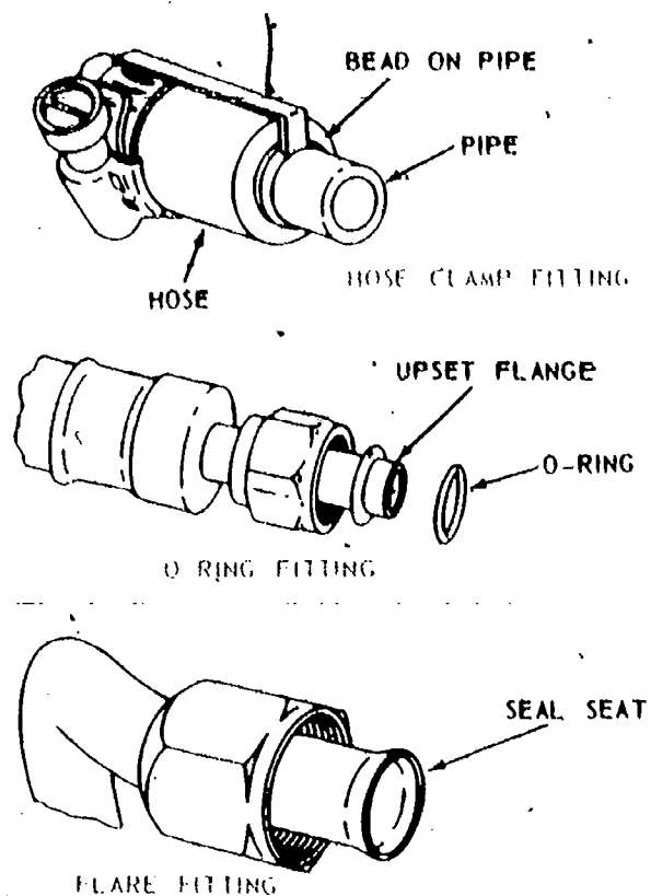
Fig. 36 — Types Of Line Connections
