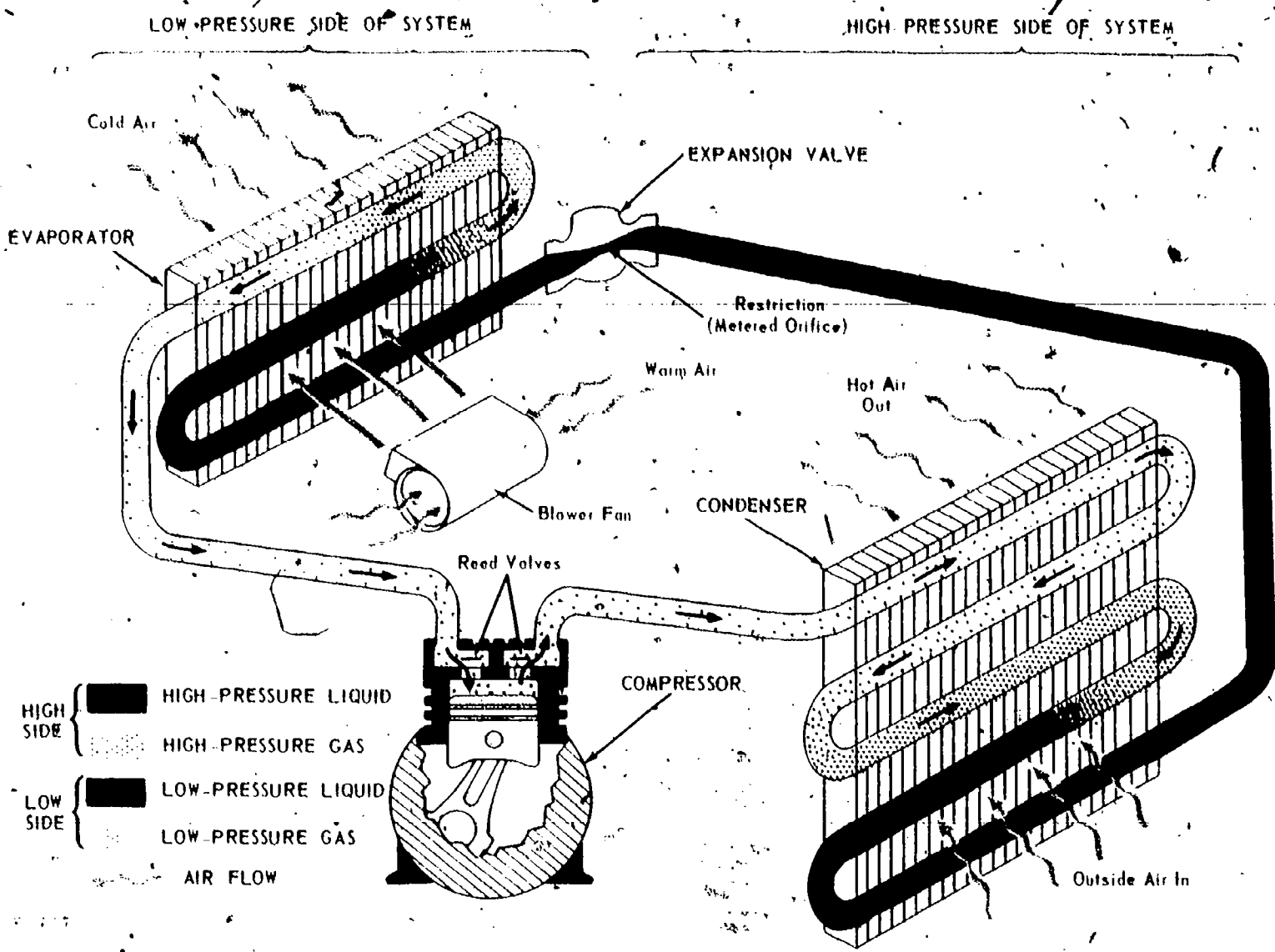
Fig. 17 — Basic Air Conditioning System
