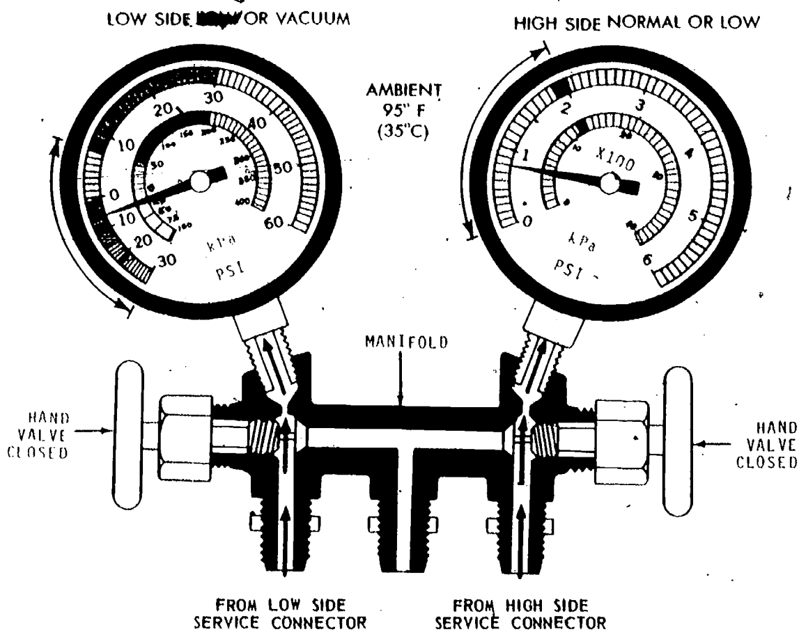
Fig. 52 — Condition No. 1
