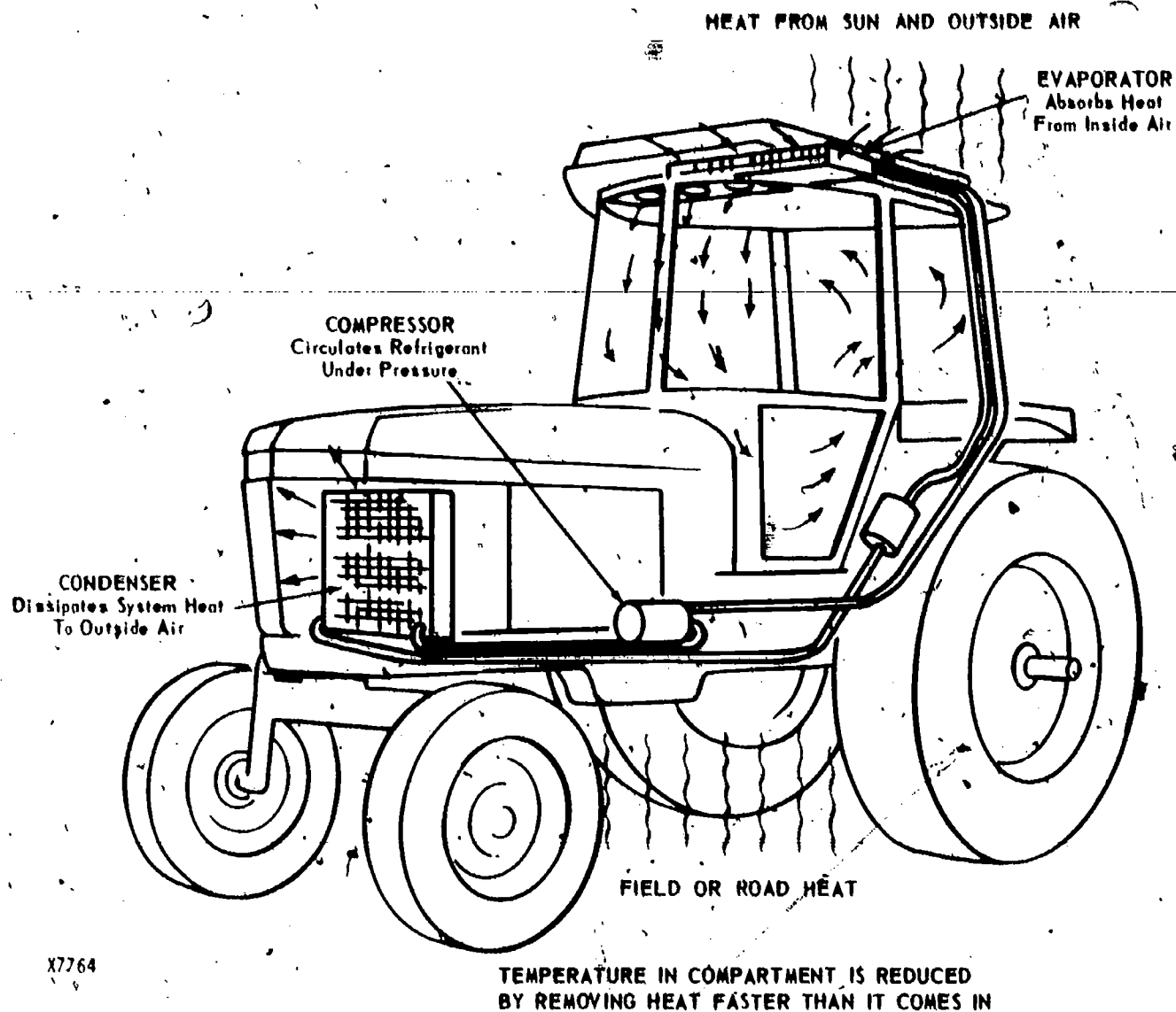
Fig. 1 — What Air Conditioning Does
