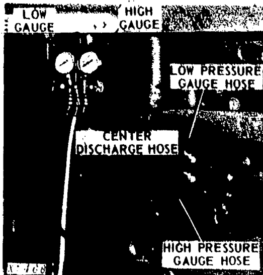
Fig. 67 — Read Low And High Side Gauges To Determine System's Condition
