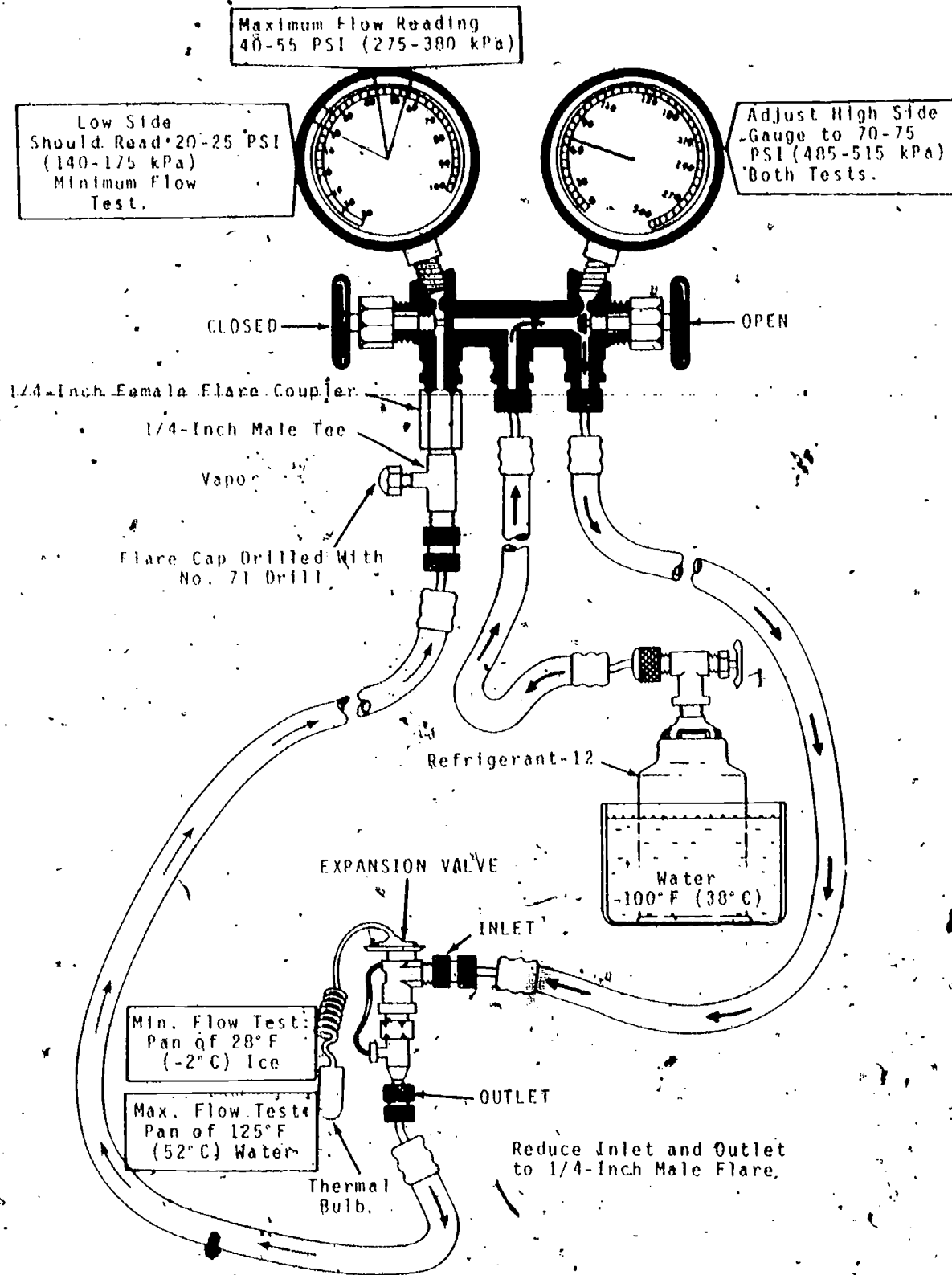
Fig. 75 — Bench Testing of Expansion Valve
