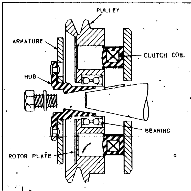
Fig 31 — Magnetic Clutch
