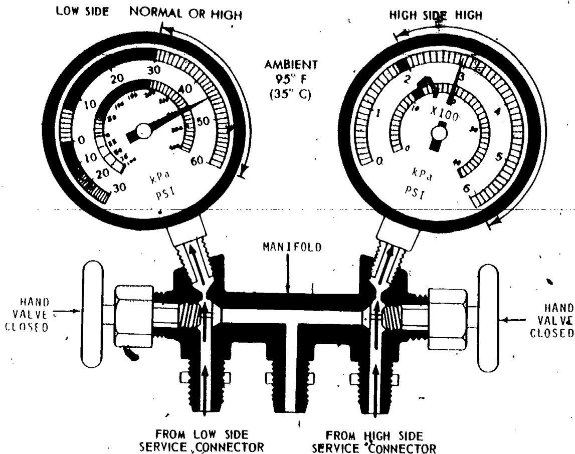
Fig. 54 — Condition No. 2
