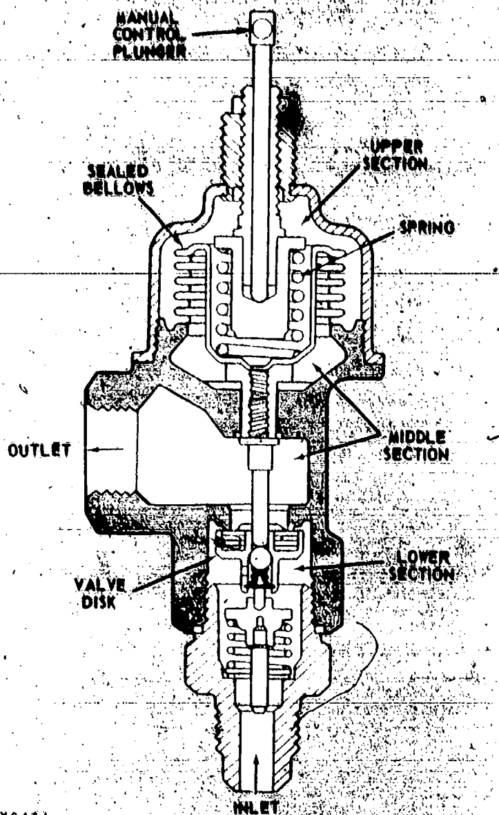
Fig. 35 — Modulator Valve
