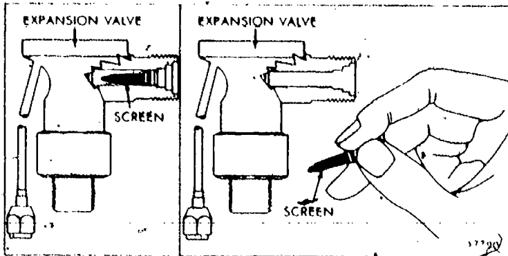
Fig. 53 — Inspect Inlet Screen
