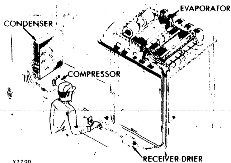
Fig. 62 — Feel Along High Side Line
