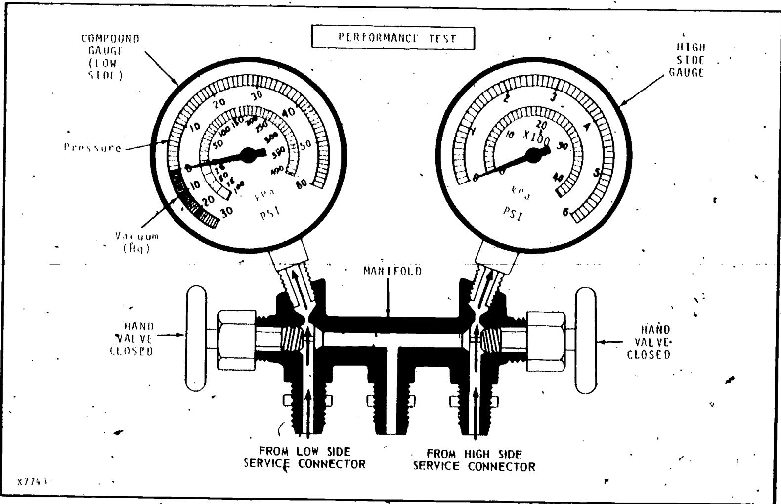
Fig. 39 — Refrigerant Flow To Gauges In Performance Test — Both Hand Valves Closed
