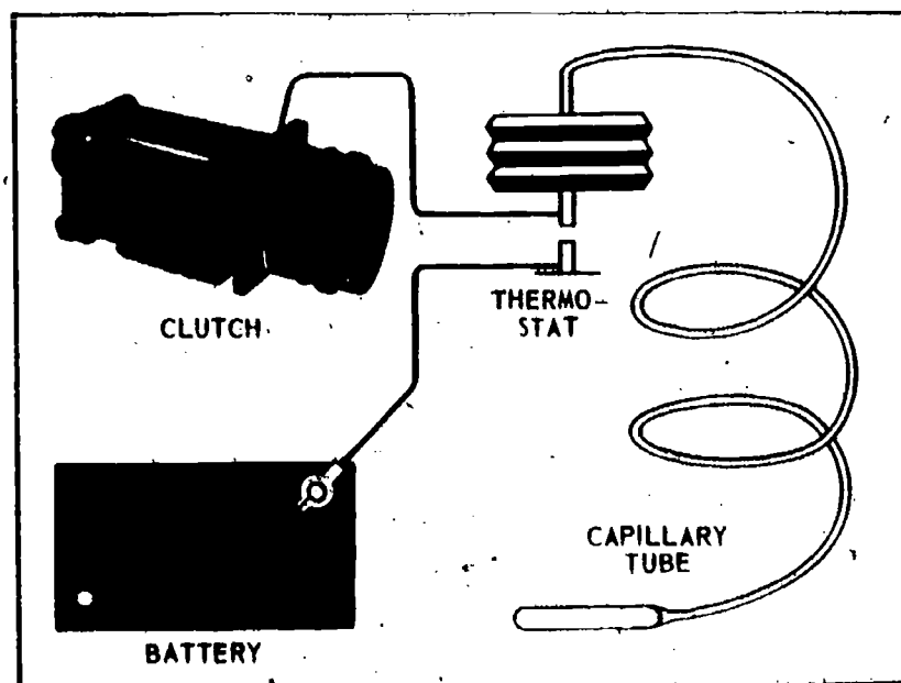
Fig. 30 — Thermostat Control
