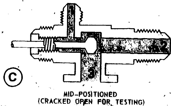
Fig. 43 — Service Valve (Hand Shutoff Type Shown)
