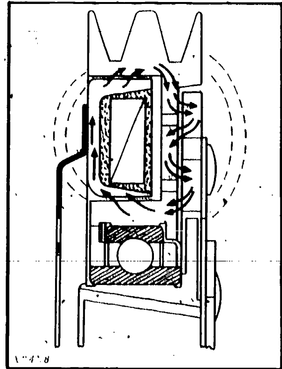
Fig. 32 — Magnetic Clutch Showing Path Of Magnetic Flow
