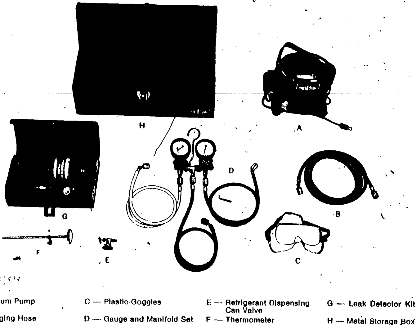
Fig. 38 — Complete Air Conditioning Service Kit
