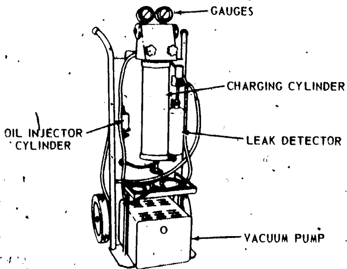
Fig 85 -- Portable Charging Station
