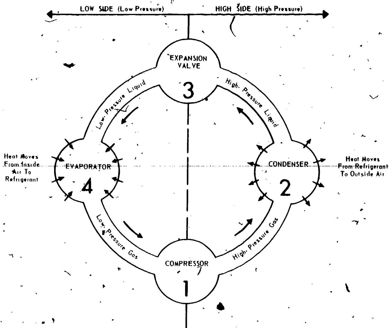
Fig. 10 — Complete Four-Part Cycle Of Refrigeration
