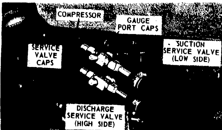
Fig. 64 — Location Of Service Valve Caps (Axial Compressor)
