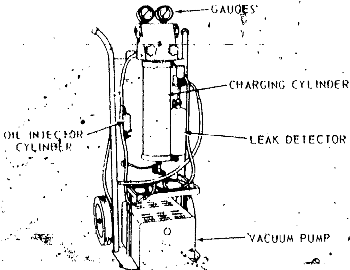
Fig. 82 — Portable Charging Station
