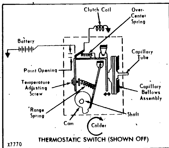
Fig. 30 — Thermostat Control
