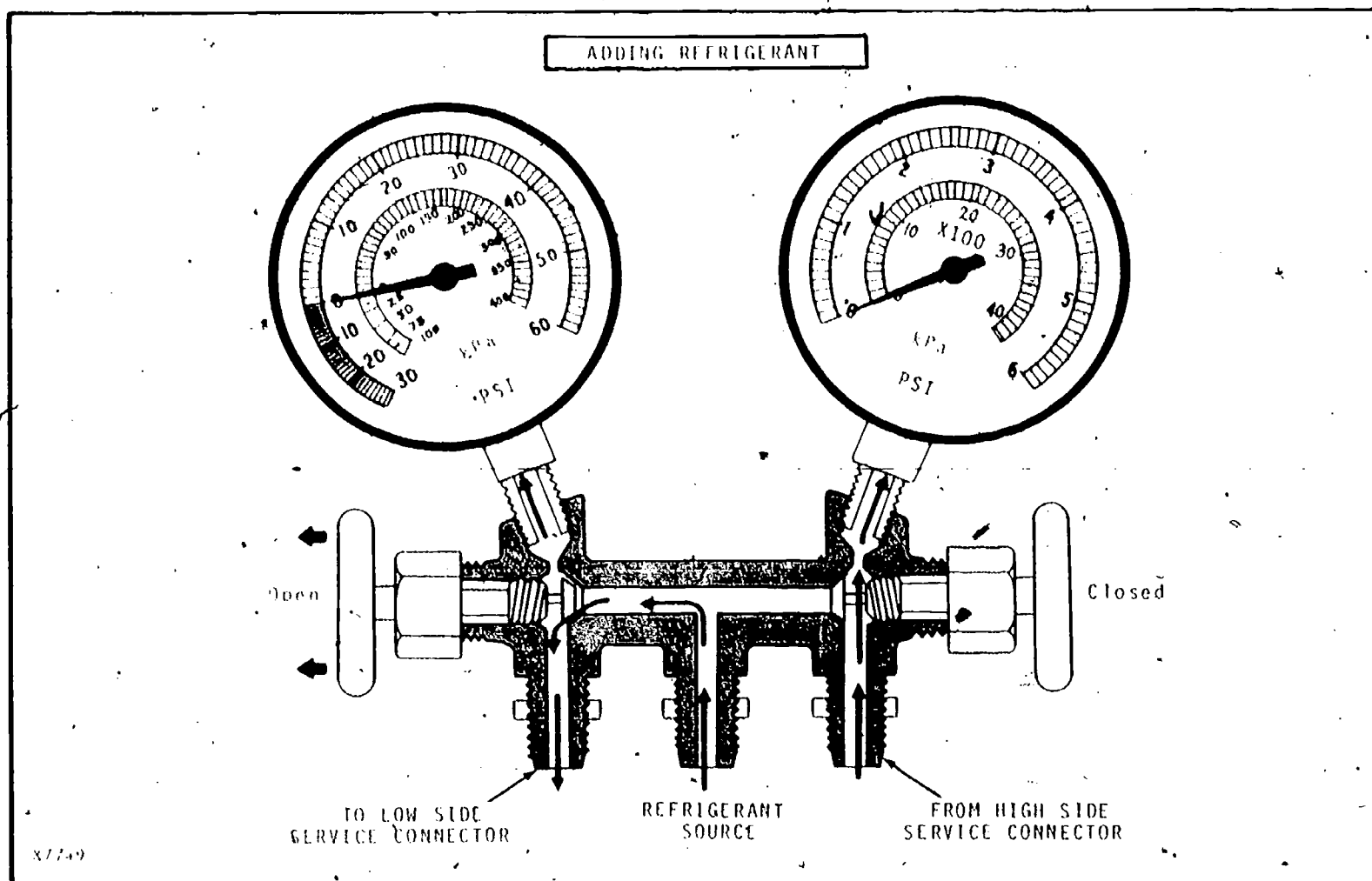
Fig. 40 — Refrigerant Flow To Gauges And Through Manifold While Adding Refrigerant
