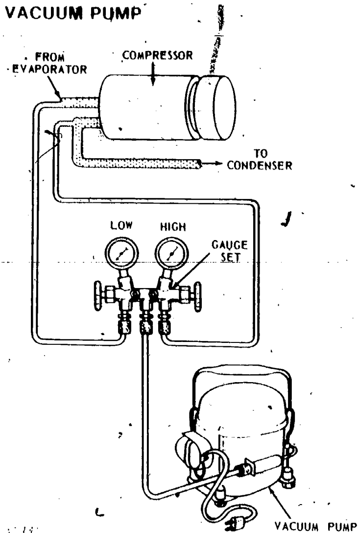
Fig. 47 — Using Vacuum Pump To Evacuate The System
