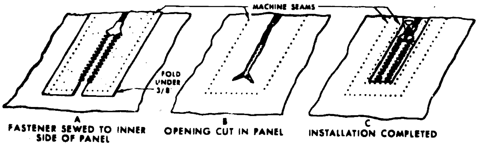
Figure 5. Modified VA-4 Interlocking Fastener Installation.
