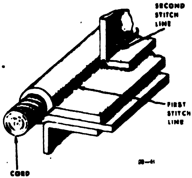
Figure 4. Cord Welt Seam.
