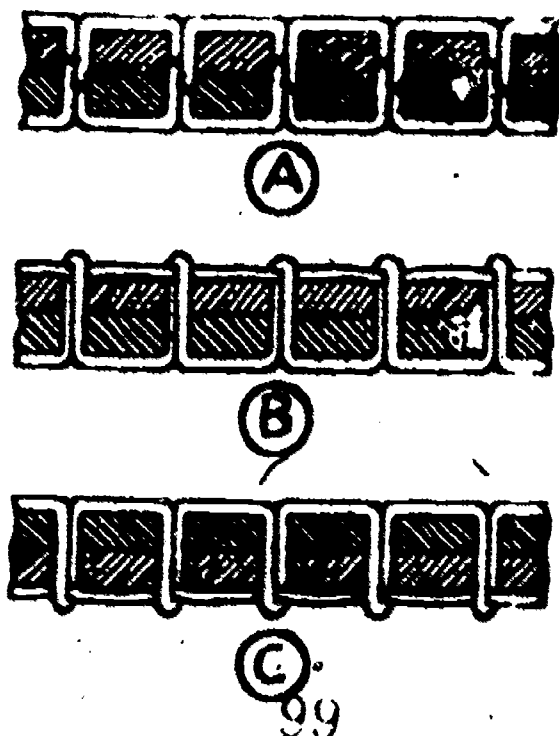
Figure 23. Correct and Incorrect Adjustments on Needle and Bobbin Threads.
