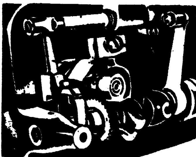
Figure 38. Adjustment of Rotary Hook.
