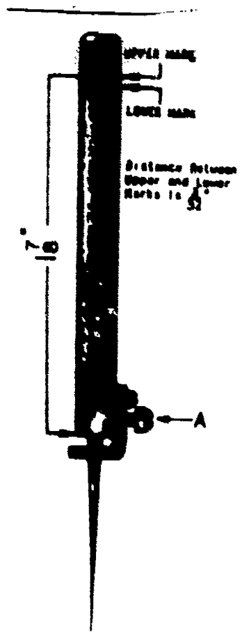
Figure 34. Marks on the Needle Bar of the 111W152 Sewing Machine.
