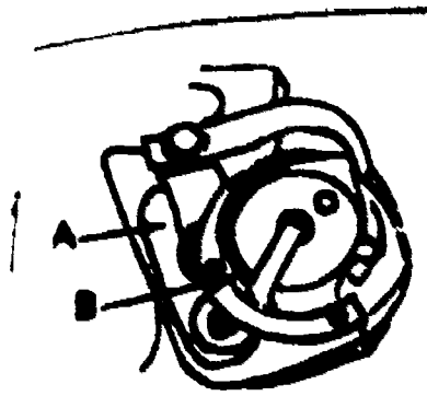
Figure 28. Hook Race and Bearing Lubrication.
