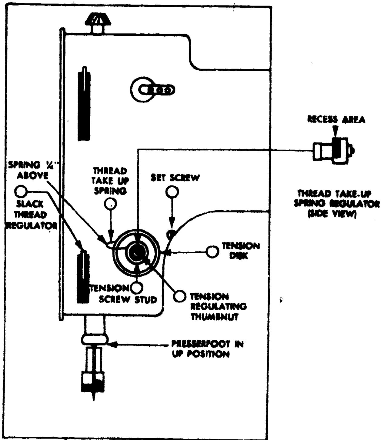
Figure 26. Adjustment of Thread Tension Assembly (Spring Tension and Position)
