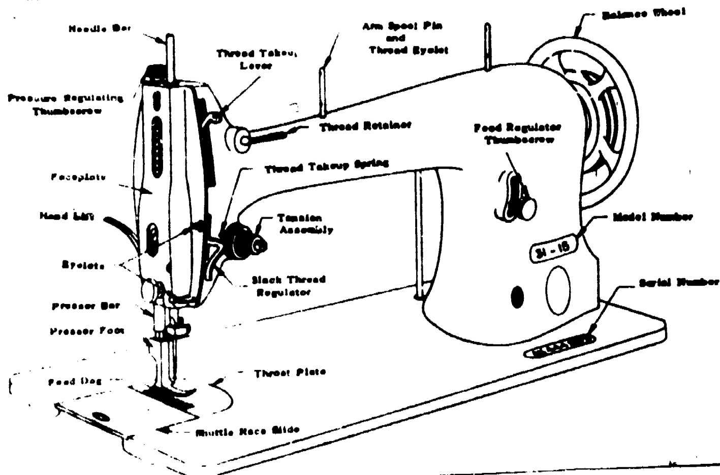
Figure 1. Class 31 Sewing Machine Head.
