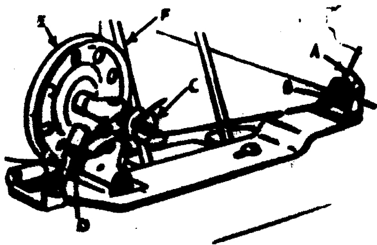
Figure 24. Winding the Bobbin.
