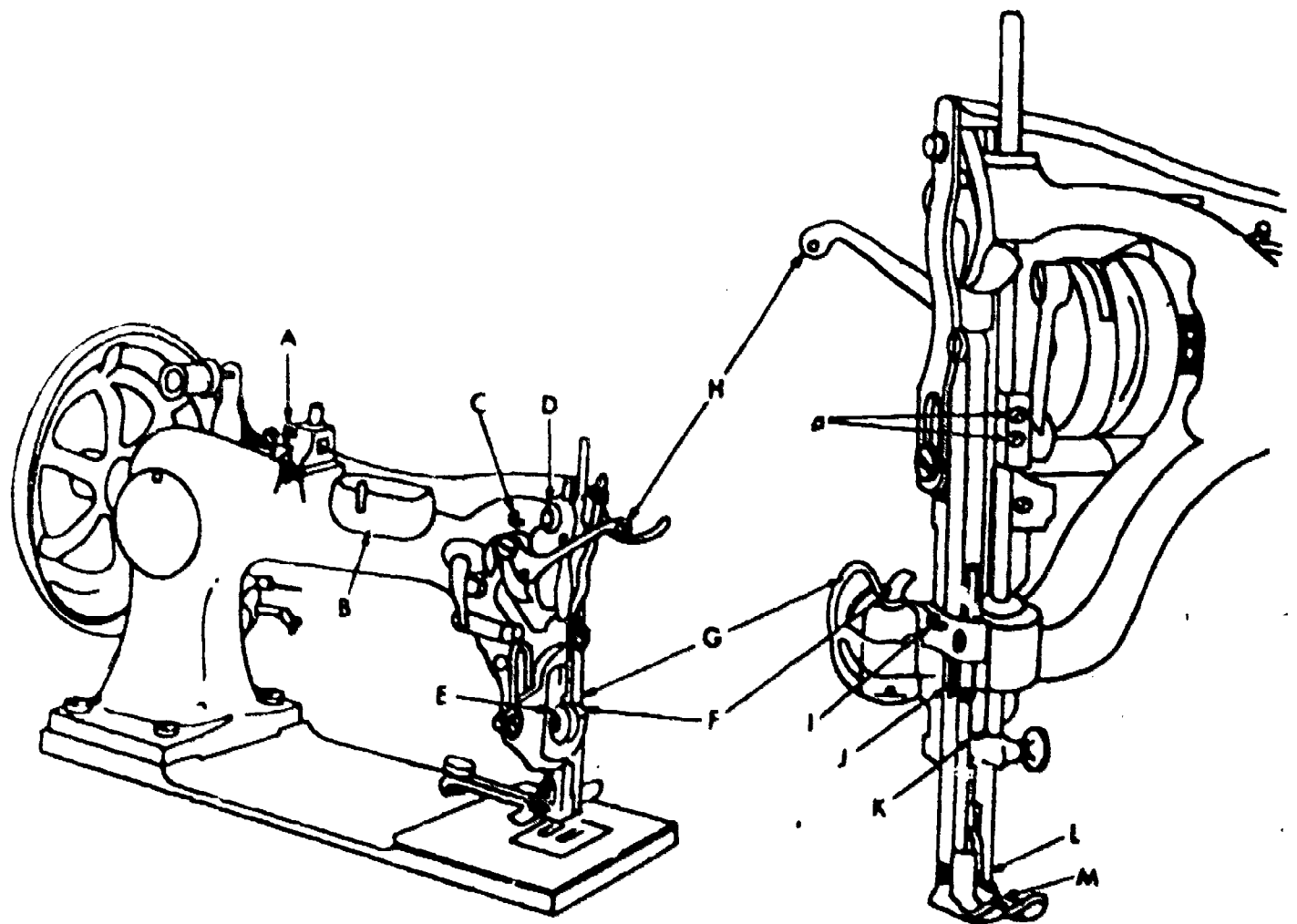
Figure 2. Threading the Class 7 Machine Head.
