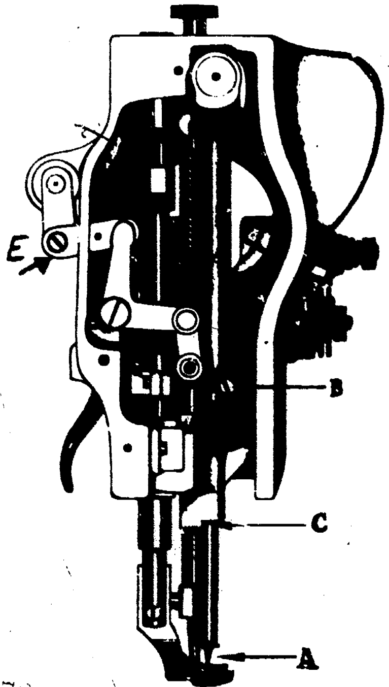
Figure 35. Setting the Needle Bar.
