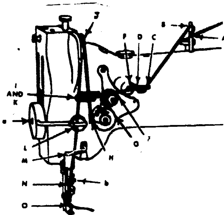
Figure 22. Threading the 111W Machine Head.
