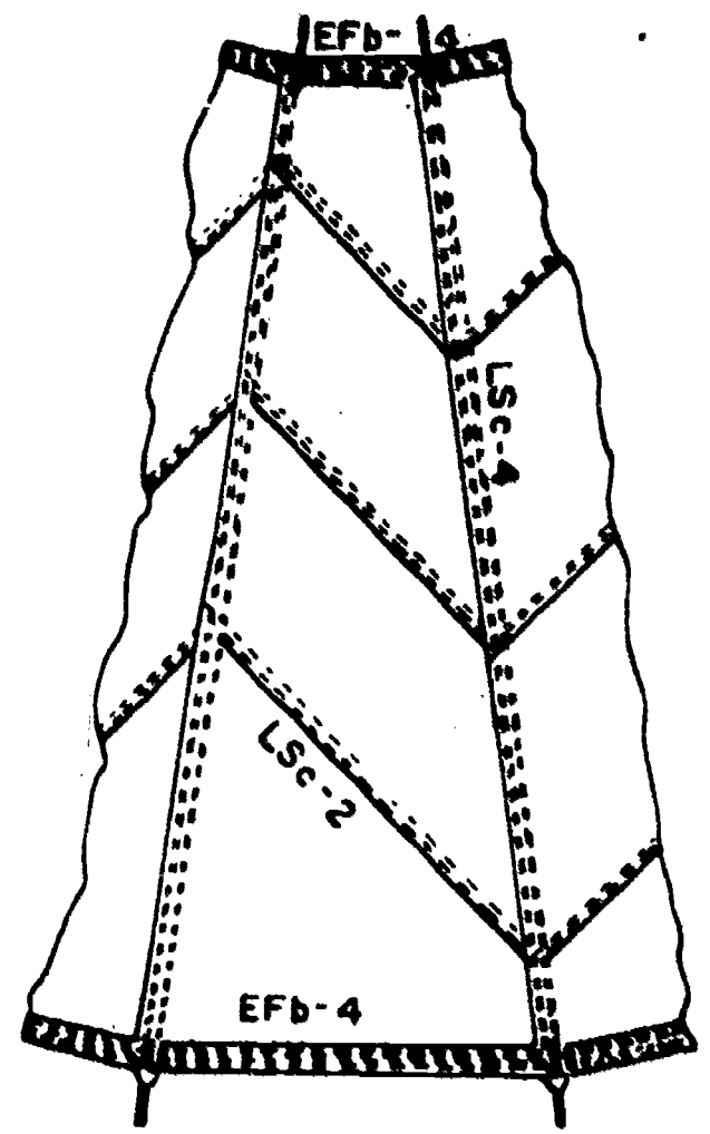
COMPLETE BIAS-CUT CANOPY PANEL
