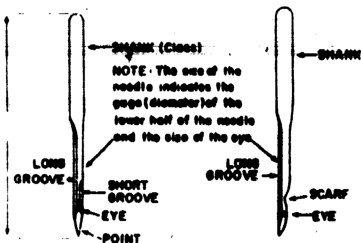
Figure 4. Sewing Machine Needles.
