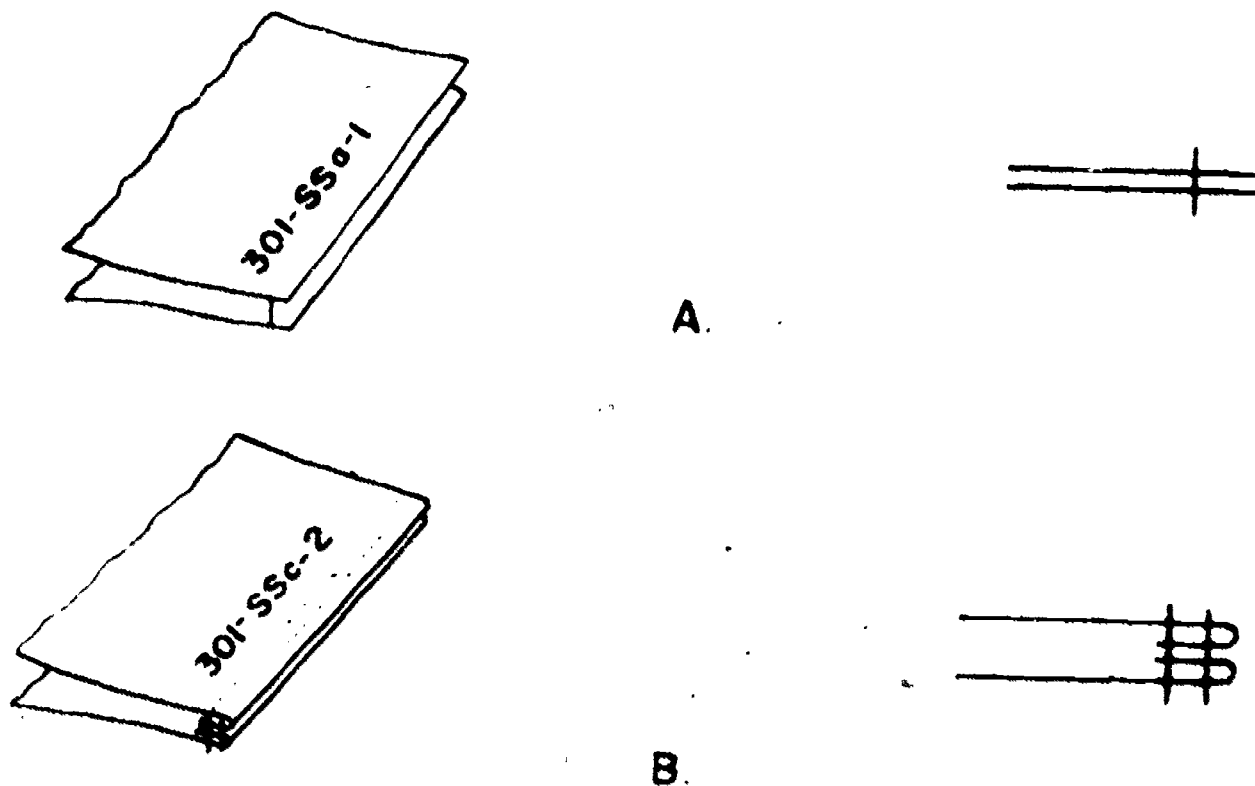
Figure 1. Types of Superimposed Seams with Cross-Sectional Views.
