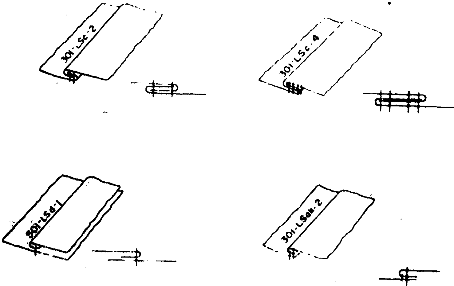
Figure 7. Lapped Seam Formation with Cross-Sectional Views.
