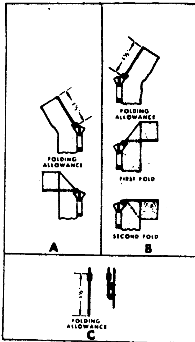
Figure 3. Methods of Folding Tapes.
