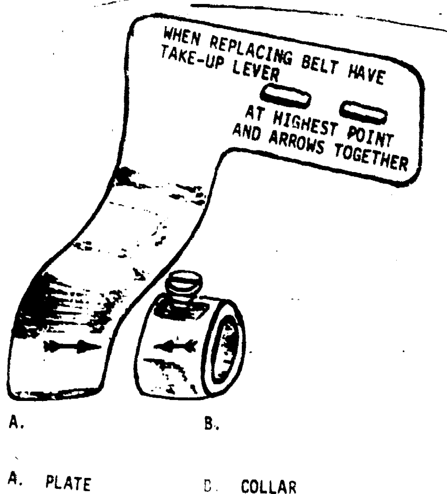
Figure 33. Arm Shaft Connection Belt Timing Collar and Plate.
