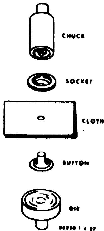
Figure 6. Glove Fastener Installation.
