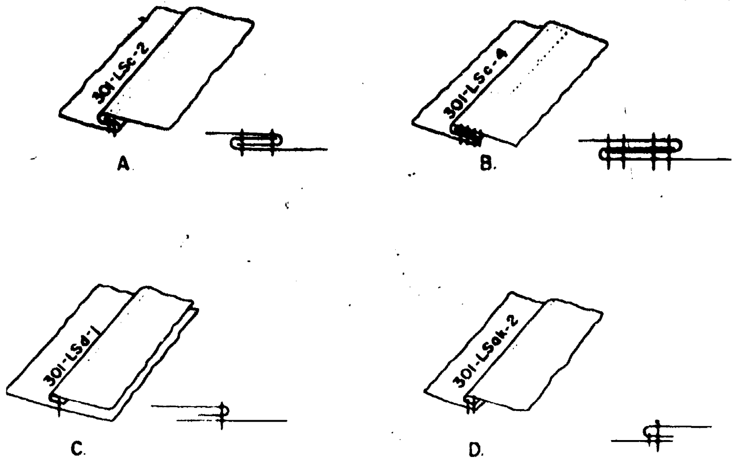
Figure 2. Lapped Seam Formation with Cross-Sectional Views.
