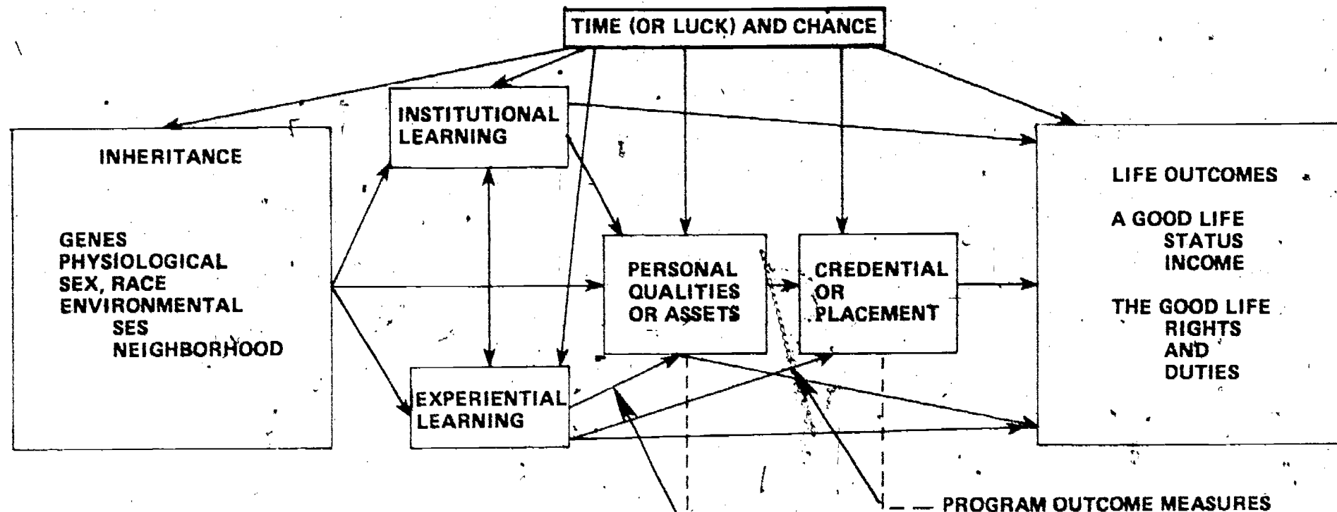
FIGURE 4. ALTERNATIVE PATH MODELS
