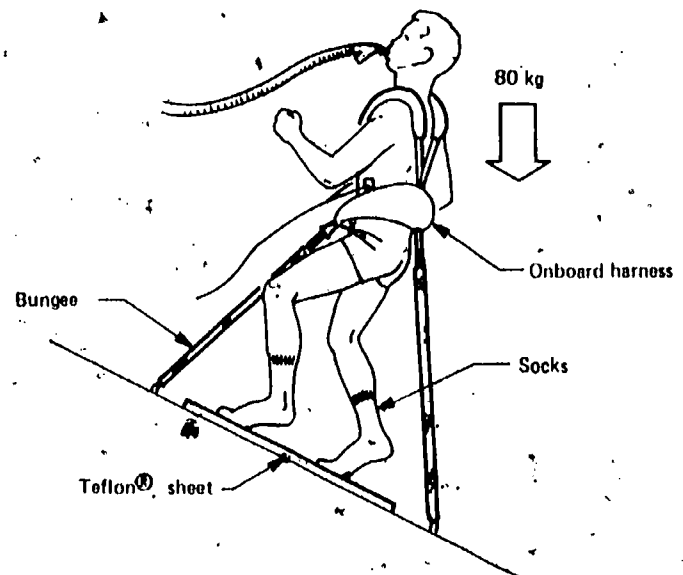
Fig. III-13. Treadmill arrangement. (From ref. III-24, p. 411.)
