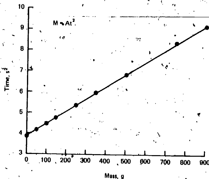
Fig. 11-5 (b). Calibration curve Skylab 2 small mass measuring device, mission day-9. (From ref. 11-12, p. 375.)
