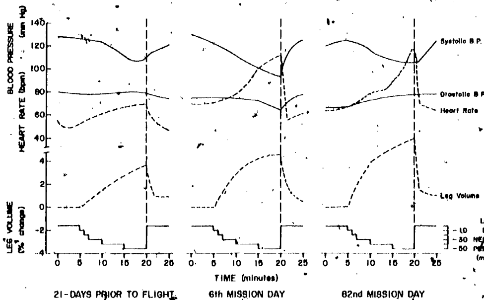
Fig. III-7 a, b, c. Cardiovascular responses of the Scientist Pilot, 3rd Manned Mission. (From ref. III-16, p. 556 and p. 582.)
