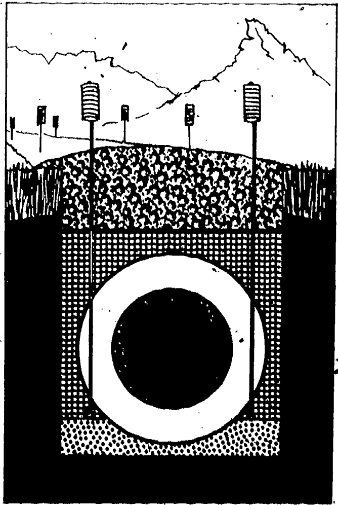
Figure 2 Metal heat sinks transfer the heat from the pipeline to above ground where the heat can be safely dissipated into the air
