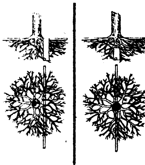
Tunnel beneath root systems. Drawings at left show trenching that would probably kill the tree. Drawings at right show how tunneling under the tree will preserve many of the important, feeder roots.
