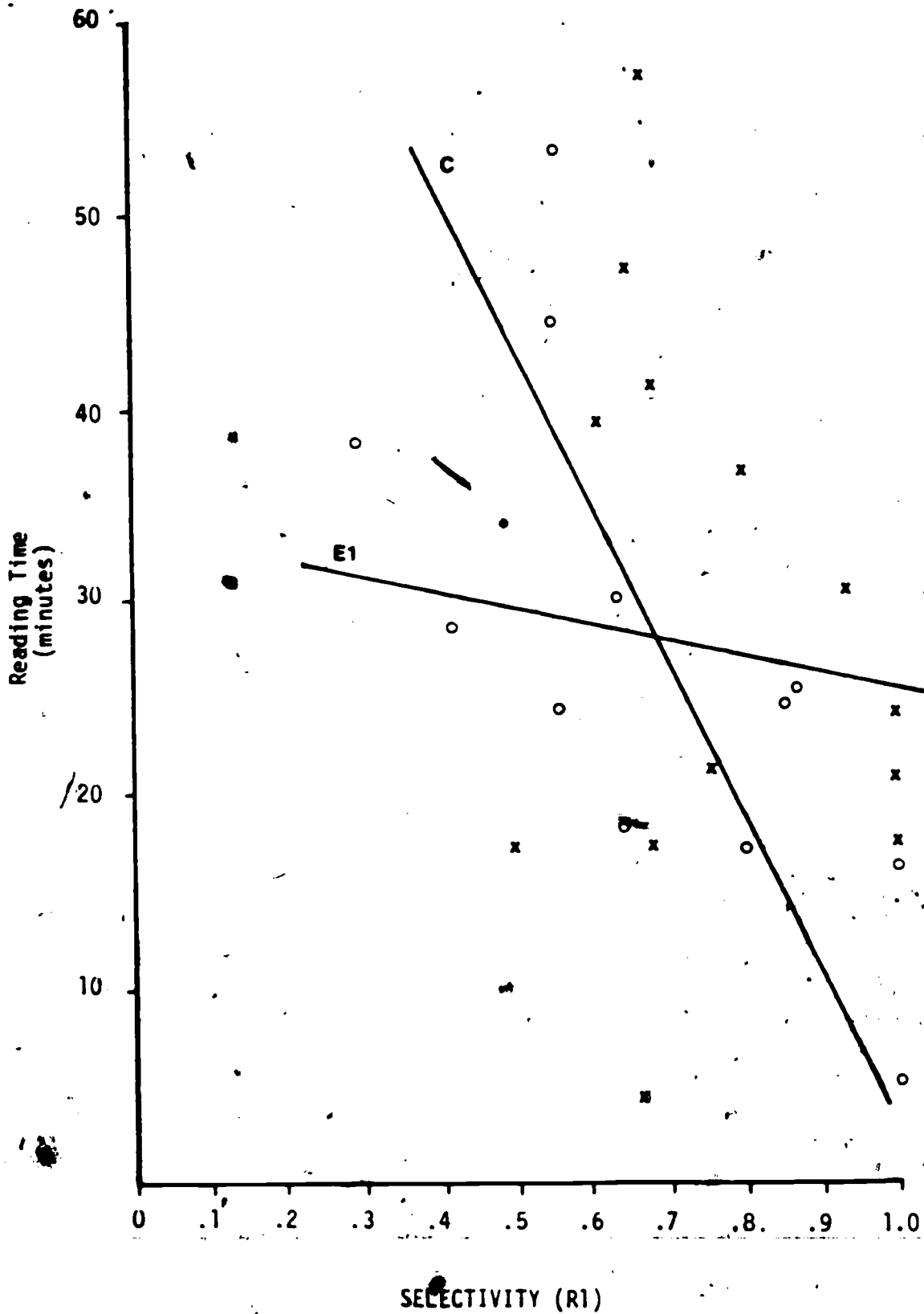
Figure 2. Correlations of selectivity and reading time for training + aids and control groups.
