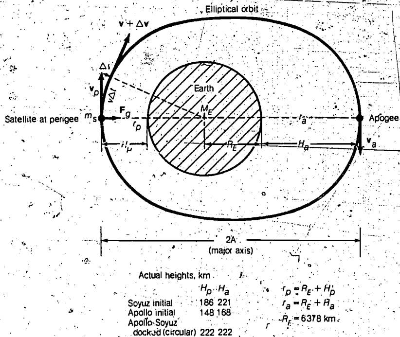
Figure 2.4 The orbit of a satellite around the Earth. The orbit size is exaggerated for clarity. The actual heights for Apollo and Soyuz are given at the bottom. The arrow F_g represents the force of gravity pulling the satellite mass m_s toward the large Earth mass M_E .
