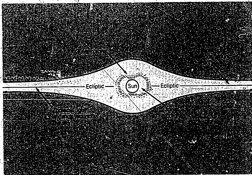
Schematic diagram of the inner corona, the outer corona, and the zodiacal light. Except for the edge of the Sun, there are no sharp edges to any of these regions.
