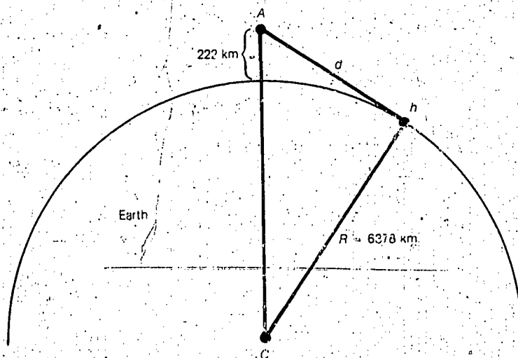
Distance to the horizon from Apollo-Soyuz. Because the line Ah is tangent to the Earth's surface at h , AhC is a 90^\circ angle.
