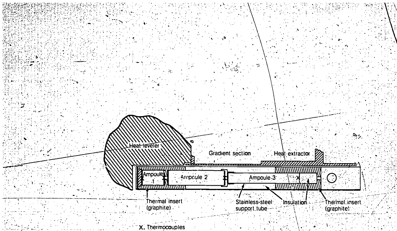
Figure 6.2 Furnace cartridge for the MA-070 Experiment. The heat leveler at the left is at the hot (bottom) end of the furnace, and the heat extractor at the right is at the cool (top) end. The three ampoules contained different mixes for heating and cooling. The manganese bismuth mix in Ampoule 3 cooled to form a strong magnetic eutectic. The graphite "inserts" and the insulation controlled the temperature gradient in Ampoules 2 and 3.
