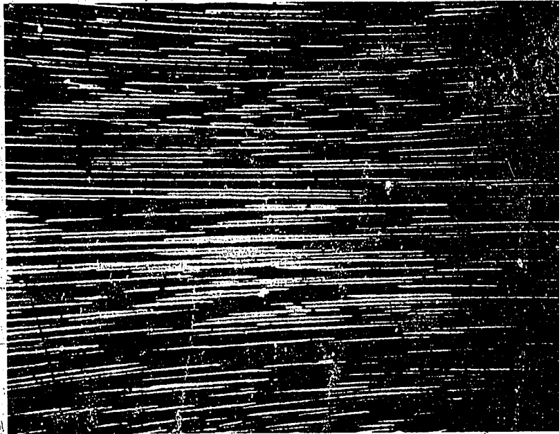
Figure 6.3 Lithium fluoride fibers in eutectic from the MA-131 Experiment. The cut-through bar of salt (enlarged 56 times) shows parallel fibers lined up by directional cooling from the molten state in zero-g.
