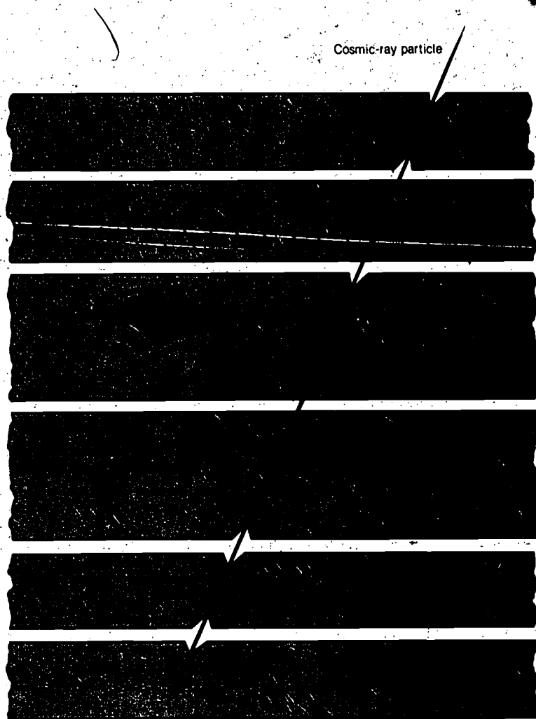
Part of Biostack III Container A with cosmic-ray track. Figure 3.2
