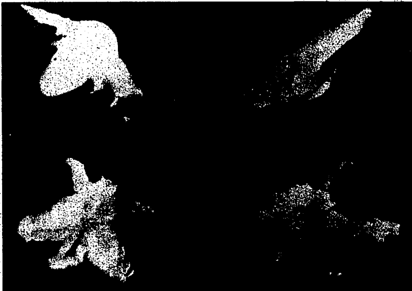
Malformations of Artemia salina induced by HZE particles that penetrated their eggs. Figure 3.8
