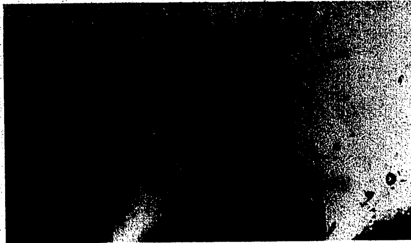
Figure 3.5 Etch cone of an HZE-particle track in CN, covered with Arabidopsis thaliana seeds in polyvinyl alcohol (PVA).
