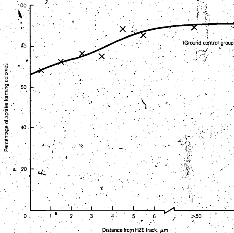
Figure 3.7 Percentage of spores forming colonies.
