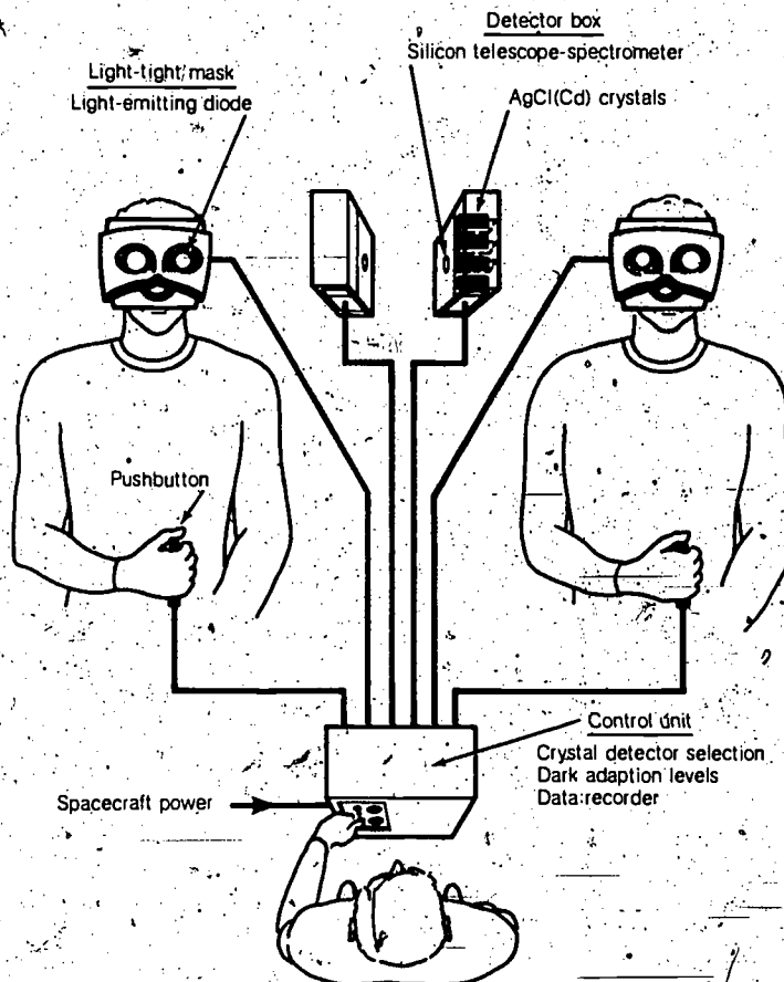
Figure 2.2 Experiment MA-106 layout.
