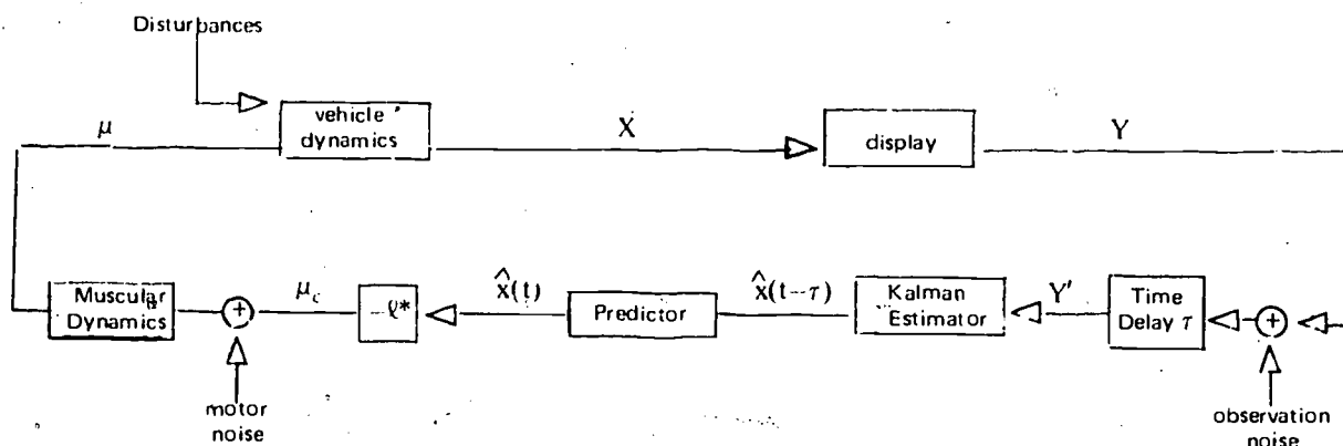
Figure 1. Optimal control model.
