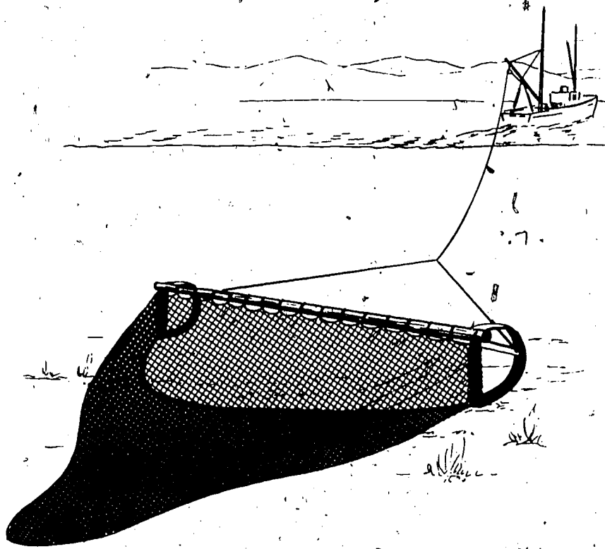
Figure 2. The beam trawl. (From Dumont and Sundstrom, 1961.)
