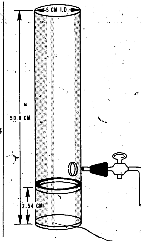
Figure 1. Plexiglas plankton settling tube with side drain and detachable cup. Not drawn to scale.
