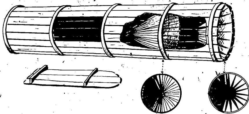
Figure 8. Slat trap. (From Dumont and Sundstrom, 1961.)
